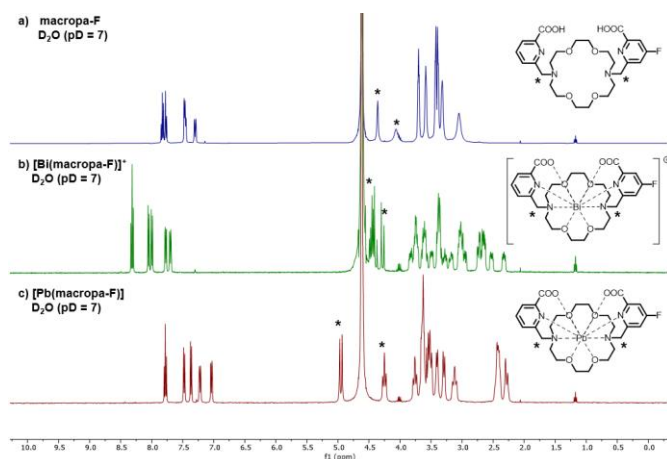
Figure 1: ^1\text{H} NMR spectra (400 MHz, 298 K, \text{D}_2\text{O} , \text{pD} = 7 , MeCN as internal reference) of a) macropa-F , b) [Bi(macropa-F)] + , and c) [Pb(macropa-F)] . The diagnostic aliphatic resonances are labelled with asterisks for each compound and indicate the diastereotopic benzylic methylene linker protons.
