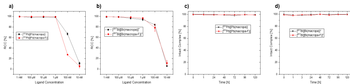
Figure 4: Summary of the radiolabelling efficiency experiments and kinetic stability studies of macropa and macropa-F with ^{203}\text{Pb} and ^{207}\text{Bi} . Experiments were performed in triplicate. a/b) Concentration-dependent radiolabelling studies with different concentrations of macropa and macropa-F and ^{203}\text{Pb} or ^{207}\text{Bi} . c) Human serum stability studies of ^{203}\text{Pb}[\text{Pb}(\text{macropa})] and ^{203}\text{Pb}[\text{Pb}(\text{macropa-F})] complexes at different time points. d) Human serum stability studies of ^{207}\text{Bi}[\text{Bi}(\text{macropa})]^+ and ^{207}\text{Bi}[\text{Bi}(\text{macropa-F})]^+ complexes at different time points.
