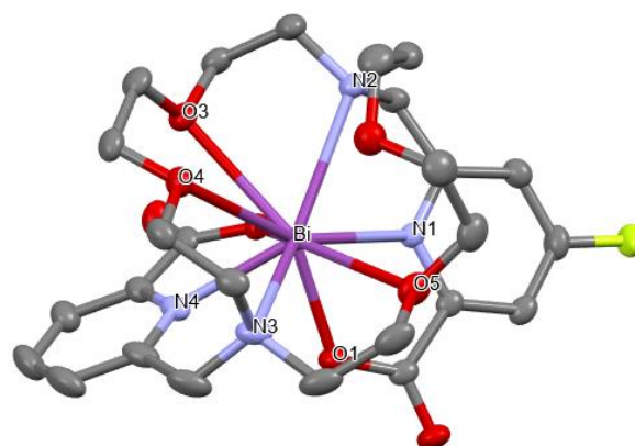
Figure 2: X-ray crystal structure of [Bi(macropa-F)] + . Ellipsoids are drawn at the 50% probability level. Hydrogen atoms, counter ions, and solvent molecules are excluded for clarity. Grey = C, red = O, yellow = F, blue = N, purple = Bi.
