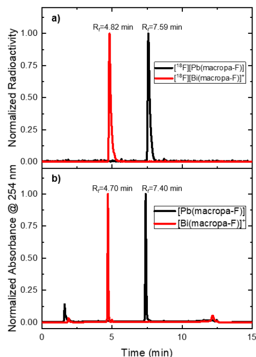
Figure 3: a) Normalized radio-HPLC traces of the independently injected radiofluorinated complexes [\text{}^{18}\text{F}][\text{Pb}(\text{macropa-F})] and [\text{}^{18}\text{F}][\text{Bi}(\text{macropa-F})]^+ . b) Analytical HPLC traces of the independently injected non-radioactive reference metal complexes [\text{Pb}(\text{macropa-F})] and [\text{Bi}(\text{macropa-F})]^+ for comparison.
