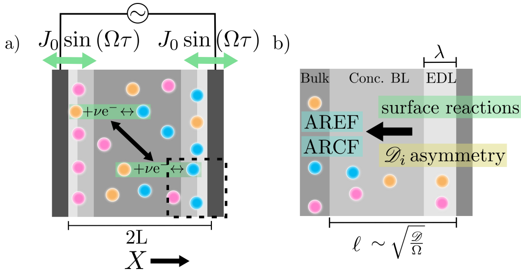
Fig. 2 Schematic of the model problem. a) We consider a cell of length 2L with an arbitrary number of ions. X is the spatial coordinate and J_0 \sin(\Omega\tau) is the charge flux due to surface reactions. b) Zoomed-in schematic of the dashed box. The cell consists of three spatial regions: the electrical double layer (EDL), a concentration boundary layer (conc. BL), and the bulk. The thickness of the EDL is denoted by \lambda and the thickness of the conc. BL is denoted by l . \mathcal{D}_i is the diffusivity of the i^{\text{th}} ion, \mathcal{D}_i is a characteristic diffusivity corresponding to the conc. BL length, and \Omega is the frequency of the applied field. We show that \mathcal{D}_i asymmetry and surface reactions can cause AREFs, and both attributes do so due to an imbalance in ionic strength. We also show that \mathcal{D}_i asymmetry can create an ARCF due to an imbalance in charge, and surface reactions can further enhance them.
