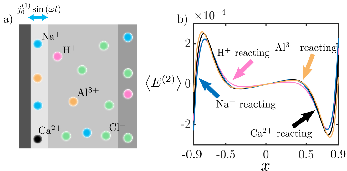
Fig. 8 Impact of the reactive ion on the AREF in an electrolyte solution with 5 ions. (a) Schematic of the model problem with H^+ , Na^+ , Ca^{2+} , Al^{3+} , and Cl^- , and a reactive charge flux j_0^{(1)} . (b) \langle E^{(2)} \rangle vs. x with H^+ (pink), Na^+ (blue), Ca^{2+} (black), and Al^{3+} (orange) reacting, respectively. j_0^{(1)} = -0.5 , \kappa = 100 , \omega = 100 , c_{Na0} = 1 , c_{H0} = 1 , c_{Ca0} = 1 , c_{Al0} = 1 , and c_{Cl0} = 7 in all cases. Results are obtained through numerical simulations.
