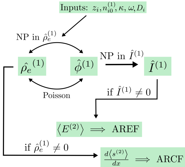
Fig. 3 Methodology for calculating the AREF and ARCF analytically in low-potential and thin-double-layer limits for multi-ion electrolytes. The key finding is that a nonzero first-order ionic strength is a sufficient criterion to observe an AREF and a nonzero first-order charge density outside EDLs is a sufficient condition to observe an ARCF.
