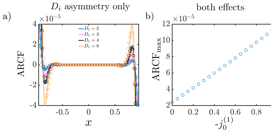
Fig. 9 Presence of ARCFs. (a) ARCF vs x for diffusivity asymmetry for D_1 = 2 (blue), D_1 = 3 (pink), D_1 = 4 (black), and D_1 = 8 (orange). D_2 = 1 in all cases. (b) ARCF_{\max} vs -j_0^{(1)} with both diffusivity asymmetry and surface reactions (only cation reactive). D_1 = 1 and D_2 = 4 . In all cases, analytical results are solid lines and numerical simulations are orbs. \kappa = 100 , \omega = 1000 , z_1 = 1 , and z_2 = -1 .
