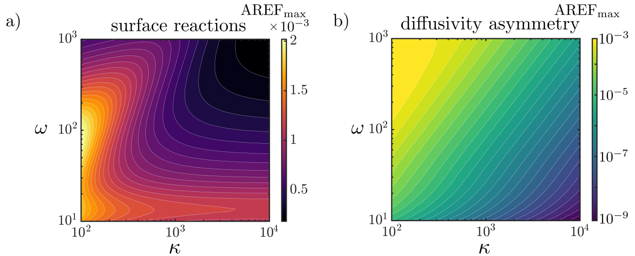
Fig. 5 Contour plot of the maximum AREF for binary electrolyte for (a) surface reactions only and (b) diffusivity asymmetry only. Panel (a) is simulated with j_0^{(1)} = -0.5 , D_1 = 1 , and D_2 = 1 , while panel (b) is simulated with D_1 = 2 , j_0^{(1)} = 0 , and D_2 = 1 . Both cases have two ions with valences of z_1 = 1 and z_2 = -1 , respectively. Variation of \text{AREF}_{\max} for the surface reactions case alone is less sensitive to changes in \kappa and \omega than the diffusivity asymmetry case alone.
