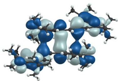
Figure 5. HOMO of the galvinoxyl dimer in the LT phase.
