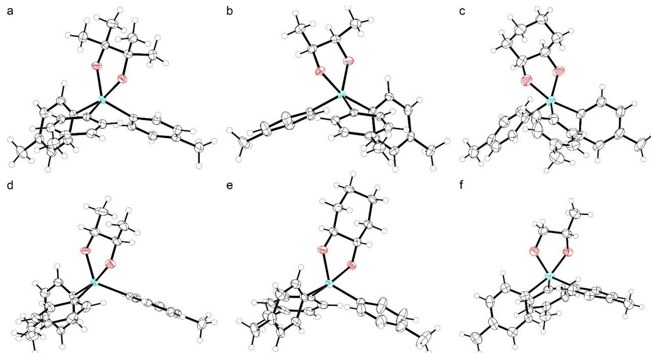
Figure 1. Thermal ellipsoid plots (50% probability) of 1-6 (a-f). Color code: Sb teal, O red, C
