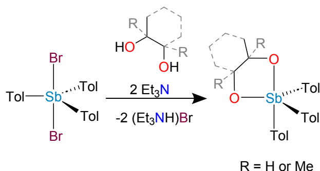
Scheme 4. Synthesis of 1-6.
