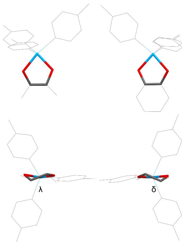
Figure 4. Crystallographically determined molecular structures of 4 ( left ) and 5 ( right ) shown with the five-membered chelate ring parallel ( top ) and perpendicular ( bottom ) to the page. The labels indicate the different ring conformations. The atoms forming the chelate ring are shown as sticks and all others as lines. Hydrogen atoms omitted for clarity. Color code: Sb teal, O red, C grey.
