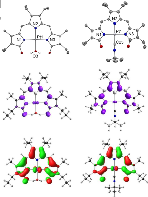
Figure 1. Crystallographic and computational analysis of [Pt(TD2*)(H 2 O)] and [Pt(TD2*)(tBuNC)] (CCDC: 2182030) in the crystal structures (top panels), the carbon-bound hydrogen atoms are omitted for clarity, and non-hydrogen atoms are displayed as thermal displacement ellipsoids set at the 50% probability level (CCDC: 2182028 and 2182030). The spin density distributions (middle) show the \alpha and \beta spin densities in purple and ivory, respectively.
