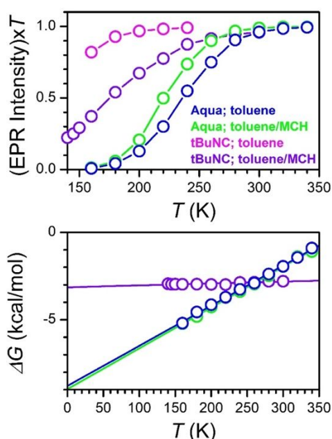
Figure 4. Temperature dependences of relative EPR intensity (top panel) and Gibbs free energy of dimerization (bottom panel) of [\text{Pt}(\text{TD2}^*)(\text{H}_2\text{O})] (blue, green) and [\text{Pt}(\text{TD2}^*)(\text{tBuNC})] (magenta, purple). The data were obtained by EPR measurements in toluene or in a 1:3 (v/v) mixture of toluene and methylcyclohexane (MCH). The complex concentrations were: 0.8 mM [\text{Pt}(\text{TD2}^*)(\text{H}_2\text{O})] in toluene, 0.2 mM [\text{Pt}(\text{TD2}^*)(\text{H}_2\text{O})] in toluene/MCH, 1 mM [\text{Pt}(\text{TD2}^*)(\text{tBuNC})] in toluene, and 0.2 mM [\text{Pt}(\text{TD2}^*)(\text{tBuNC})] in toluene/MCH. The free energy temperature dependence for [\text{Pt}(\text{TD2}^*)(\text{tBuNC})] in toluene is not
