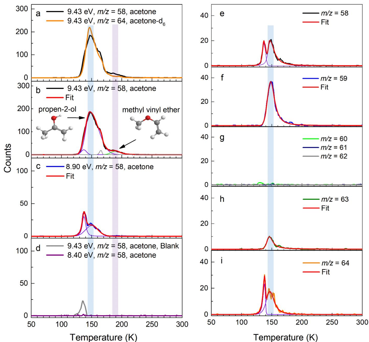
Fig. 4 PI-ReToF-MS data during the TPD phase measured for irradiated ( 0.34 \pm 0.05 eV molecule -1 ) acetone ice at m/z = 58 at photon energies of 9.43 eV (a and b), 8.90 eV (c) and 8.40 eV (d). Spectra of irradiated acetone- d_6 ice measured at m/z = 64 was recorded at 9.43 eV (a). The blank experiment acetone ice was recorded at 9.43 eV (d). Spectra of acetone-acetone- d_6 ice were recorded at 9.43 eV at m/z = 58 (e), m/z = 59 (f), m/z = 60 - 62 (g), m/z = 63 (h), and m/z = 64 (i) after lower dose irradiation ( 0.10 \pm 0.02 eV molecule -1 ). The blue and purple shaded regions indicate the peak positions corresponding to propen-2-ol ( 2 ) and methyl vinyl ether ( 4 ), respectively. The solid red lines indicate total fit of the spectra.
