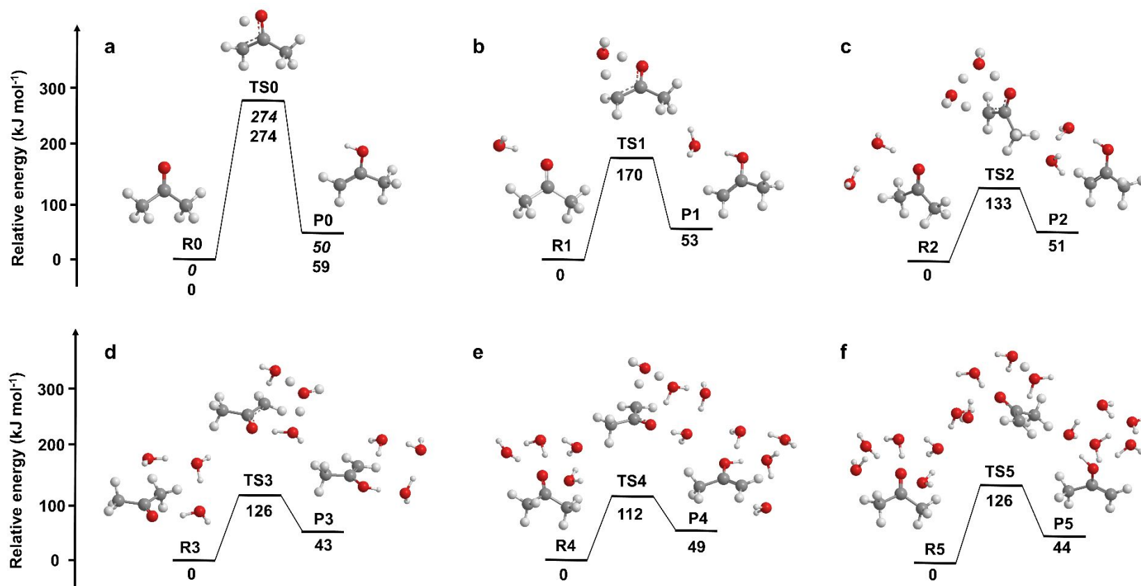
Fig. 5 Potential energy surfaces of reactions between acetone and water molecules leading to the formation of propen-2-ol (2). Panel a describes the gas-phase keto-enol tautomerization reaction of acetone (1). Panels b – f show the tautomerization reaction in the presence of 1 – 5 microsolvating water molecules with the inclusion of polarizable continuum model (PCM) solvent modeling to best replicate the condensed-phase environment of interstellar ices. Energies (kJ mol -1 ) are calculated at the \omega B97X-D/6-311G(d,p) level with CCSD(T)-F12/cc-pVTZ-F12 single-point corrected energies are in italics
