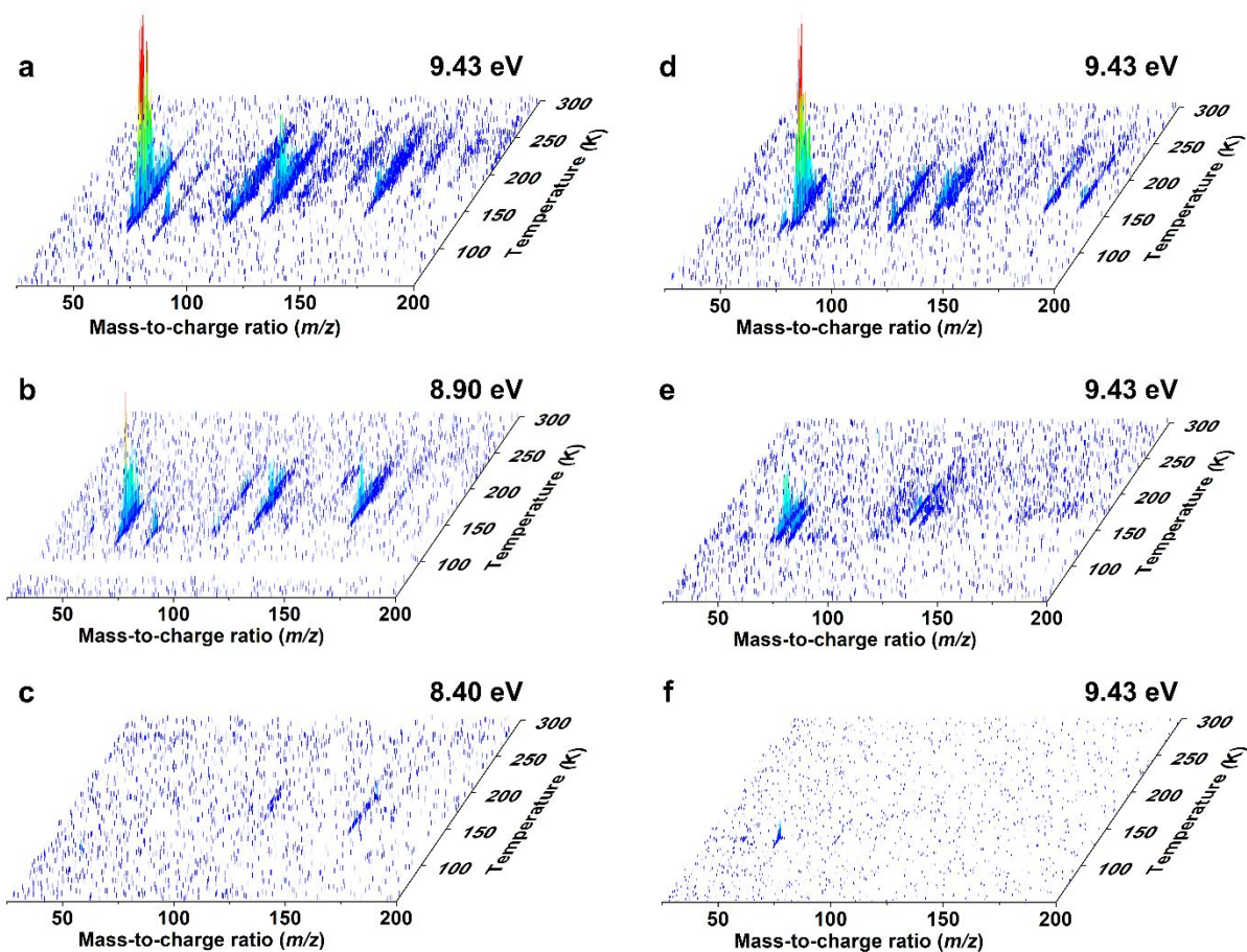
Fig. 3 PI-ReToF-MS mass spectra collected during the temperature-programmed desorption (TPD) of the irradiated ices. Data were recorded for the irradiated acetone ice at photon energies of 9.43 eV (a), 8.90 eV (b), and 8.40 eV (c), the irradiated acetone- d_6 ice at 9.43 eV (d) as well as the irradiated acetone-acetone- d_6 ice at 9.43 eV (e). The blank experiment of the acetone ice performed under identical conditions, but without irradiation, was recorded at 9.43 eV (f).
