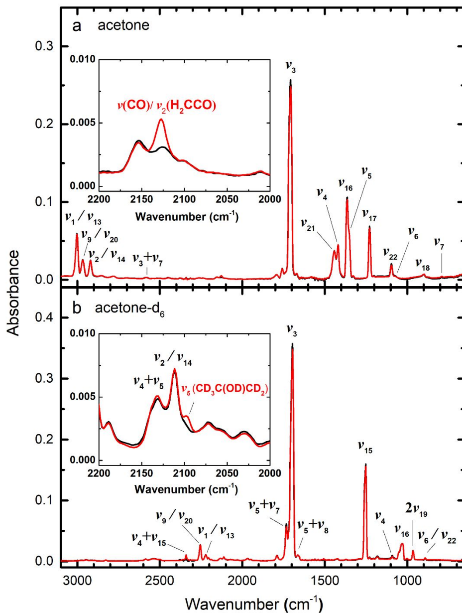
Fig. 2 FTIR spectra of acetone ices at 5 K before (black line) and after (red line) irradiation: (a) acetone, (b) acetone-d 6 . Detailed assignments are compiled in Tables S4-S5. Inset: magnified view of 2200 – 2000 cm -1 showing new peaks after irradiation corresponding to carbon monoxide and/or ketene at 2128 cm -1 (a) and tentatively assigned propen-2-ol-d 6 at 2096 cm -1 (b).
