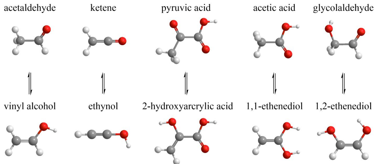
Scheme 1 Tautomer pairs observed in interstellar analog ices subjected to ionizing radiation.
