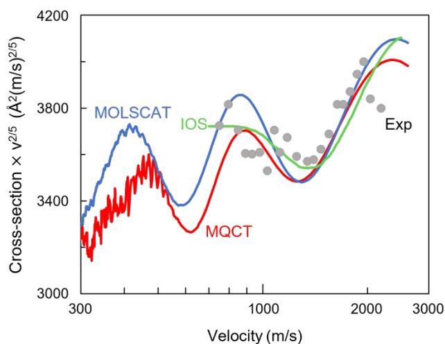
Figure 5: Velocity-scaled cross sections as a function of O-atom collision velocity. Red line is MQCT results, blue line is MOLSCAT results, green line is IOS approximation from literature, and black dots are experimental data.
