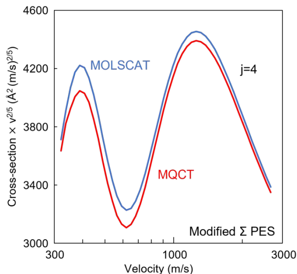
Figure 6: Velocity-scaled cross sections as a function of O-atom collision velocity calculated using a modified \Sigma PES for the initial state of N_2(j = 4) . Red line is MQCT results, blue line is MOLSCAT results.
