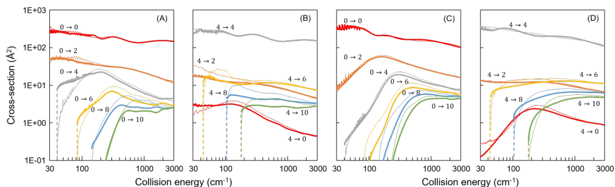
Figure 1: State-to-state transition cross sections from the initial states j = 0 and j = 4 to several final states j' using two PESs for \text{N}_2 + \text{O} system: \Pi PES (frames A, B) and \Sigma PES (frames C, D). Thick lines correspond to MQCT results, while thin lines are MOLSCAT results. Dashed lines are used to indicate threshold energies of excitation transitions.
