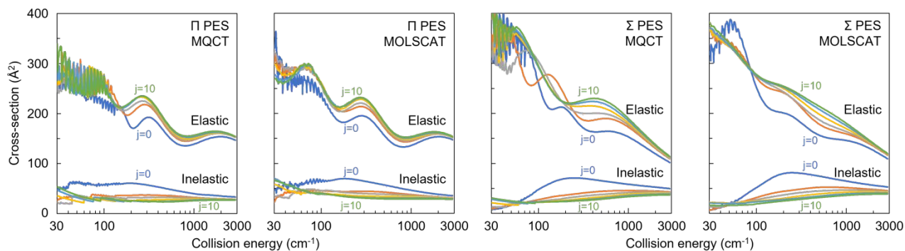
Figure 2: Elastic and inelastic cross sections as a function of collision energy obtained by MQCT and MOLSCAT methods for different initial states of N_2 + O system indicated by colors: j = 0 is blue, j = 2 is orange, j = 4 is gray, j = 6 is yellow, j = 8 is turquoise and j = 10 is green. Two left frames are obtained for \Pi PES, while two right frames correspond to \Sigma PES.
