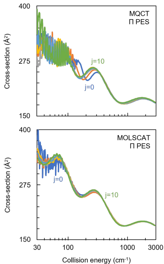
Figure 3: Total cross sections (elastic + inelastic) as a function of collision energy computed using MOLSCAT and MQCT for the initial states 0 \leq j \leq 10 of N_2 + O system using \Pi PES. Colors are the same as in Figure 2.
