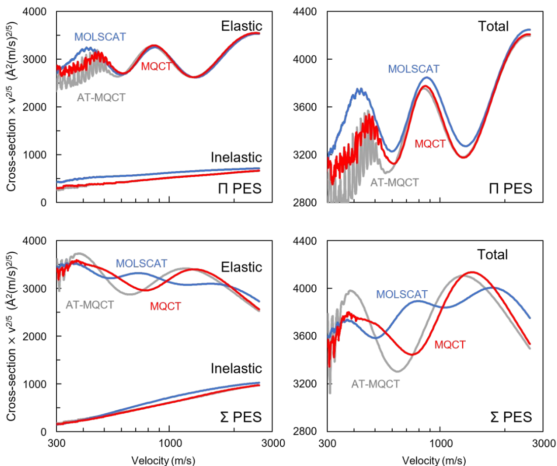
Figure 4: Velocity scaled cross sections as a function of average collision velocity obtained by three theory methods, as indicated by color. Left panels – elastic and inelastic cross-sections, right panels – total cross-sections. Upper and lower rows correspond to \Pi and \Sigma PESs of N_2 + O system, respectively.
