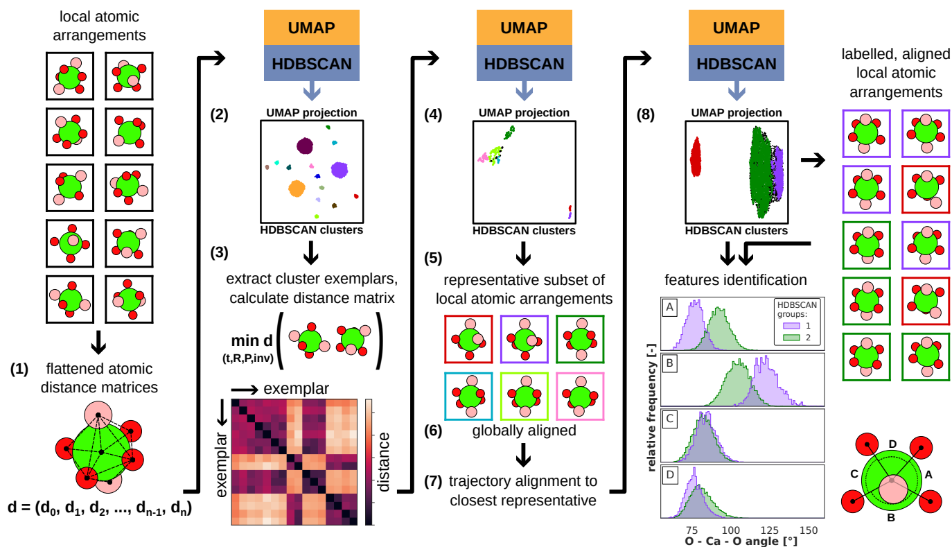
Fig. 1 Schematic described in the text highlighting the multi-step process by which local atomic arrangements for a given chemical formula are ultimately grouped into clusters of aligned atomic arrangements through successive application of dimensionality reduction (UMAP), hierarchical density-based clustering (HDBSCAN) and alignment via minimization of the root mean square deviation d while including translation (t), rotation (R), permutation (P), and inversion (inv) of the atomic coordinates (FASTOVERLAP), followed by specific distinguishing feature identification that helps to define interpretable labeling of the final clusters.
