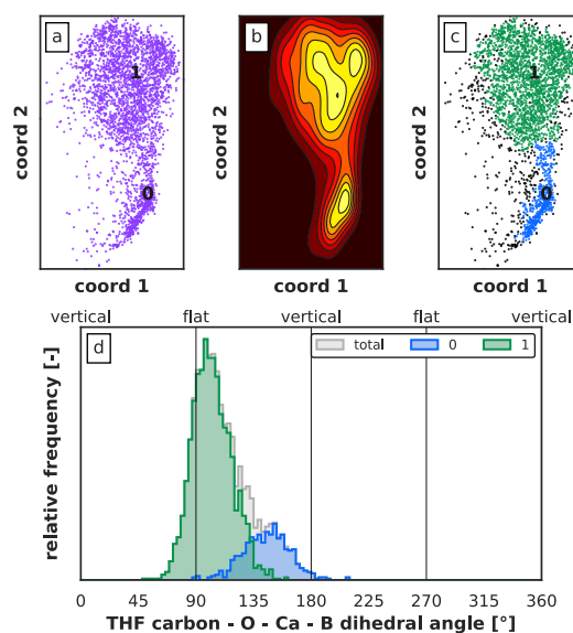
Fig. 8 (a) UMAP projection of group 1 from Figure 6. The labels 0 and 1 correspond to the peaks in density of the heatmap in (b). (c) Contribution of the two regions to the first dihedral angle of group 1 (F) in Figure 7. (d) Dihedral of the F THF molecule with contribution from the two high density regions.
