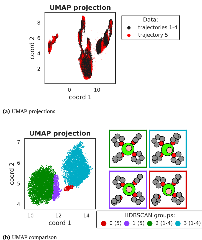
Fig. 12 (a) Projection of the data from trajectory 5 on the UMAP pipeline of trajectories 1-4. Most of the newly projected data lies at the ridges or between previously existing clusters. (b) Overlap of the UMAP projection of groups 2 and 3 from trajectories 1-4 (Figure 6a) and UMAP projection of data from trajectory 5 that is close to it and has been divided by HDBSCAN in two groups (0 and 1).
