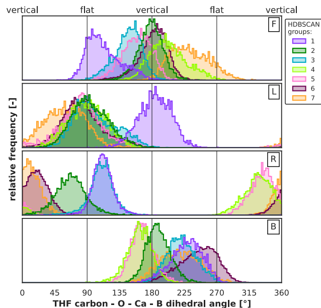
Fig. 7 Distribution of the dihedrals between the C atoms of the THF molecules and the axis spanned by the two B atoms in the case they are axially arranged (groups 1-7 in Figure 6). F: front, L: left, R: right, B: back THF molecule.
