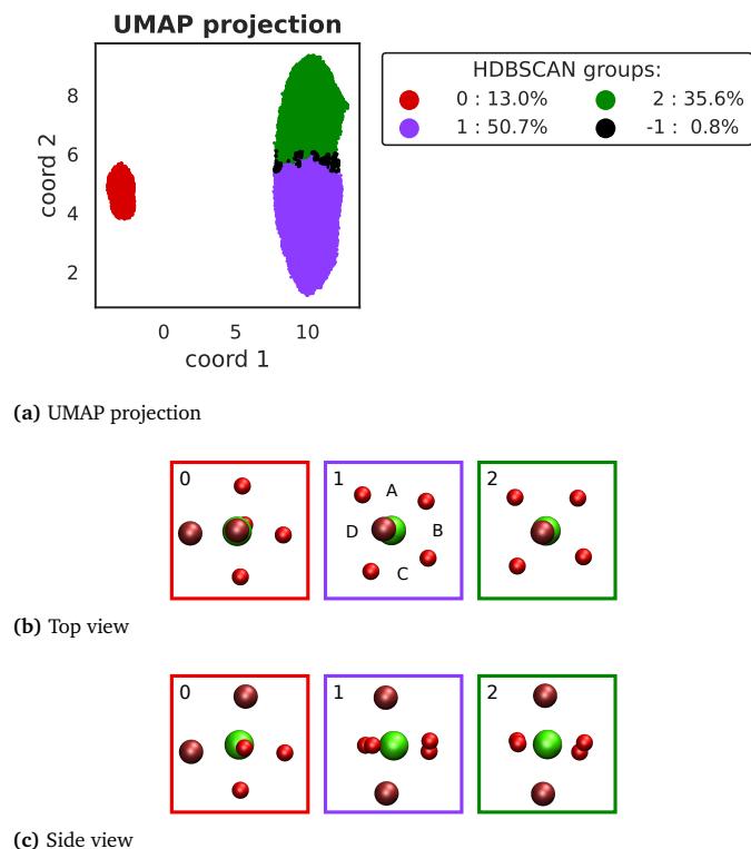
Fig. 3 (a) UMAP projection colored according to HDBSCAN labelling of \text{B}_2\text{CaO}_4 local atomic arrangements of trajectories 1-4. Points classified as noise are labelled -1 (black). (b) Top and (c) side view of the averaged local atomic arrangements for each HDBSCAN group.
