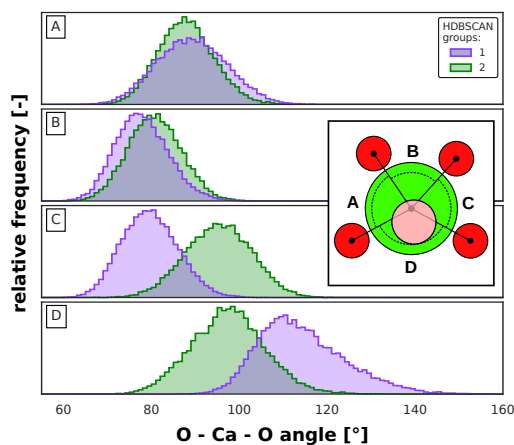
Fig. 4 Distribution of angles between neighbouring O atoms with center on the Ca for the groups 1 and 2. The detail within the figure shows the ordering of the angles A, B, C and D.
