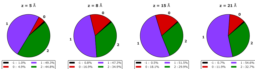
Fig. 5 Distribution of species of B 2 CaO 4 as a function of distance from the interface (z).
