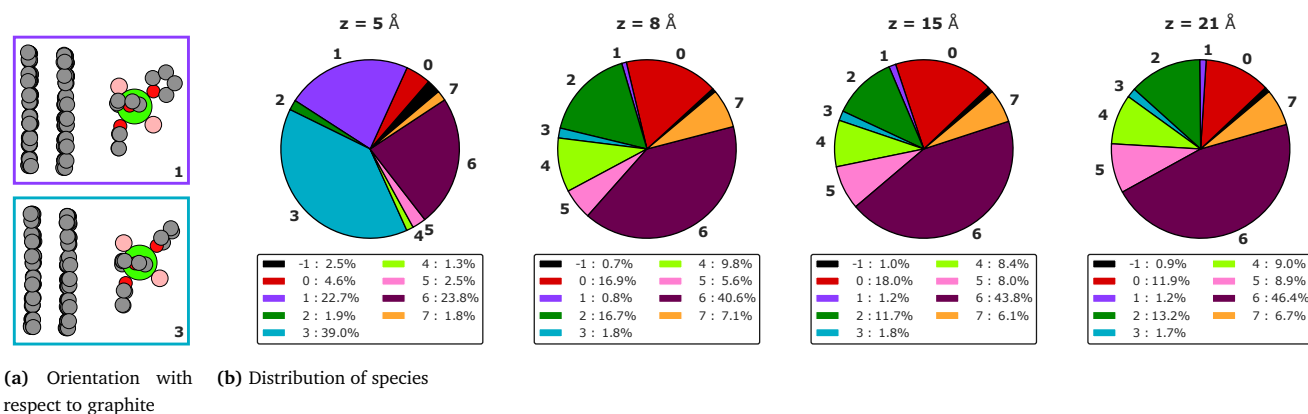
Fig. 9 (a) Orientation of local atomic arrangements of isomers 1 and 3 with respect to the graphite layer. (b) Distribution of species of B_2CaO_4 with THF carbons as a function of the distance to the interface ( z ). Note that isomers 1 and 3 appear almost uniquely closest to the surface.
