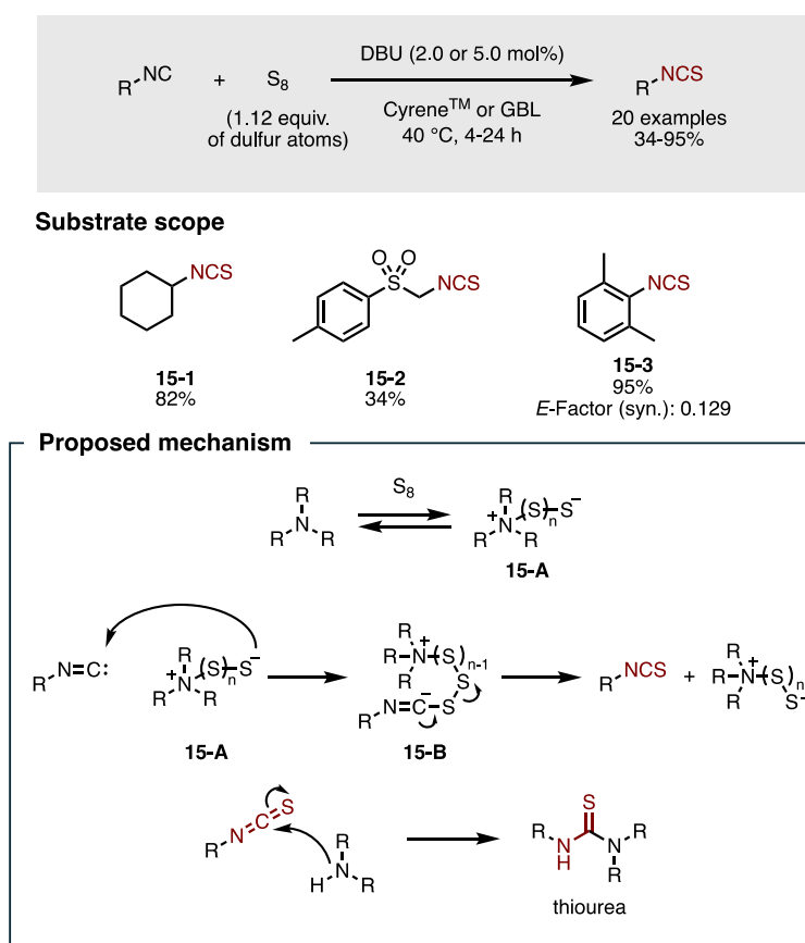
Figure 20. Sustainable isothiocyanation by amine-catalyzed sulfurization of isocyanide.
