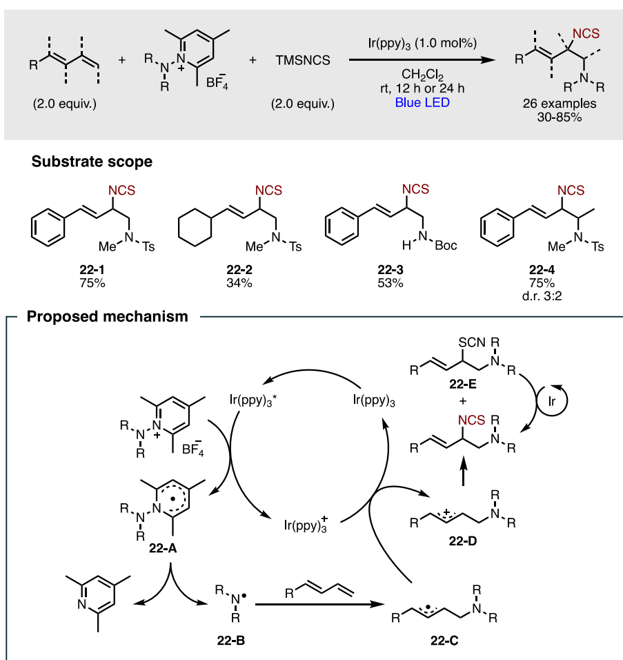
Figure 29. Photocatalyzed 1,2-aminoisothiocyanation of 1,3-dienes.
