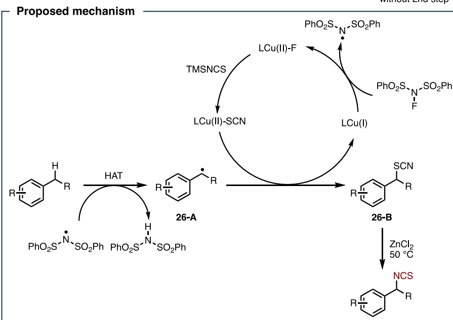
Figure 33. Copper-catalyzed C–H thiocyanation and one-pot isothiocyanation.
