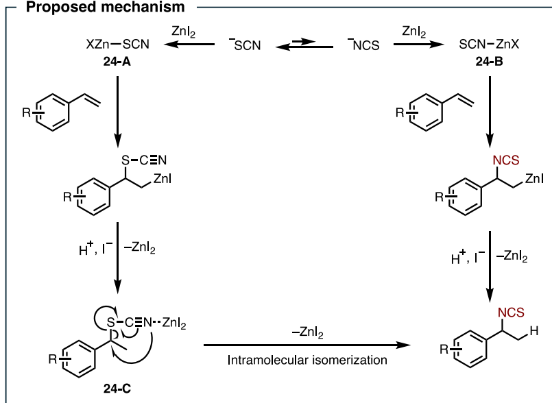
Figure 31. Hydroisothiocyanation of alkenes with ammonium thiocyanate.
