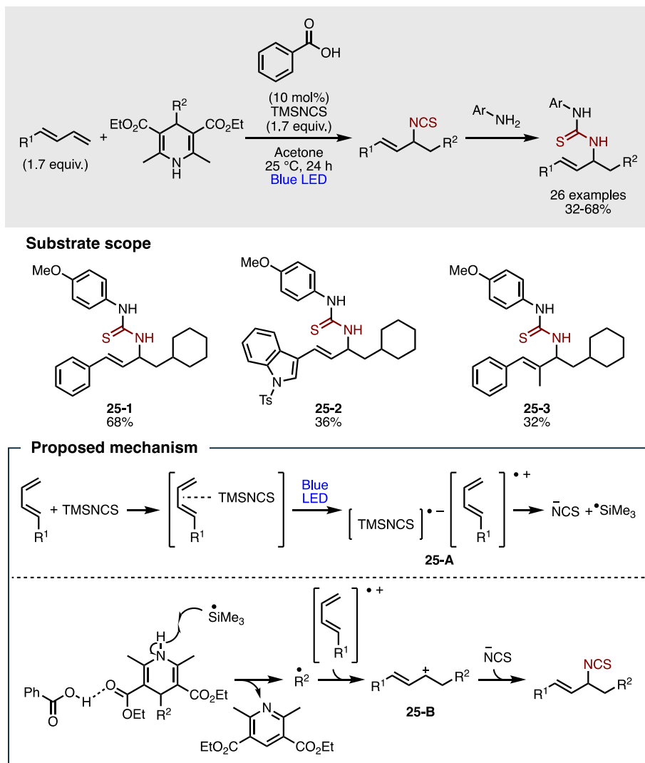
Figure 32. Photo-induced 1,2-carboisothiocyanation of dienes.
