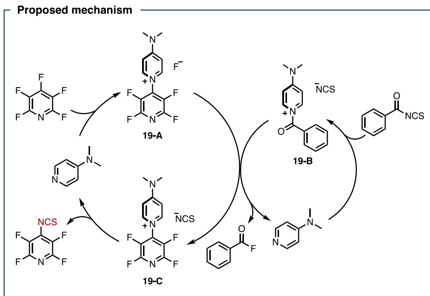
Figure 25. Synthesis of 4-isothiocyanato-tetrafluoropyridine by S_NAr .
