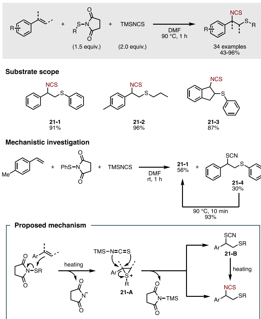
Figure 28. Catalyst-free isothiocyanatoalkylthiation of styrenes.
