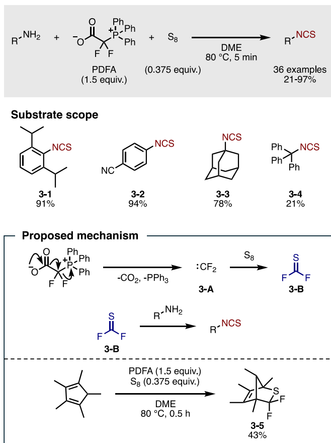
Figure 7. Isothiocyanation with PDFFA and S_8 .
