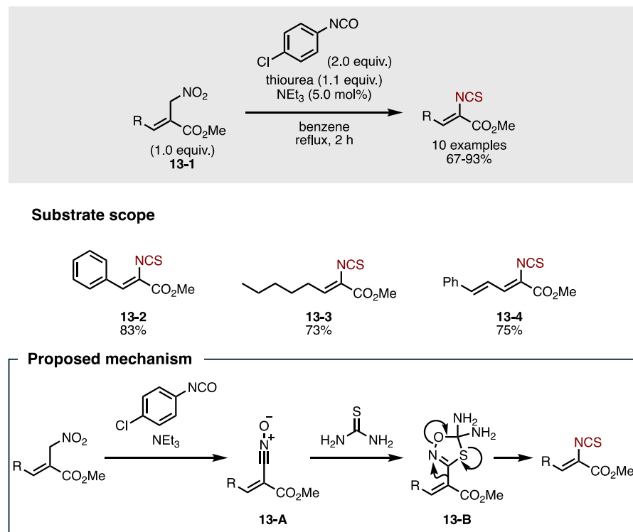
Figure 18. Synthesis of \alpha -isothiocyanato- \alpha,\beta -unsaturated esters.
