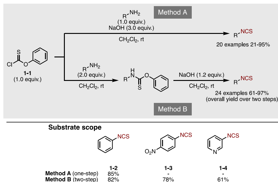
Figure 4. Synthesis of isothiocyanates with chlorothionoformate.
