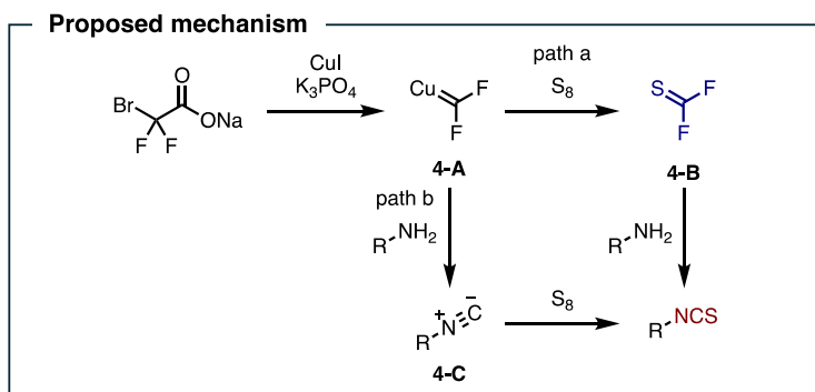
Figure 8. Copper-catalyzed isothiocyanation without organophosphine reagent.
