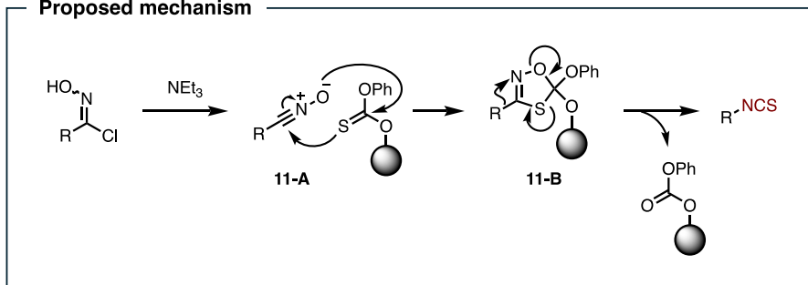
Figure 16. Purification-free isothiocyanation via fragmentation from polymer-supported 1,4,2-oxathiazoles.
