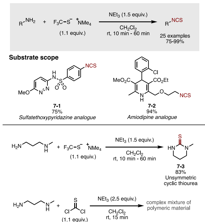
Figure 11. Isothiocyanation with (\text{Me}_4\text{N})\text{SCF}_3 .
