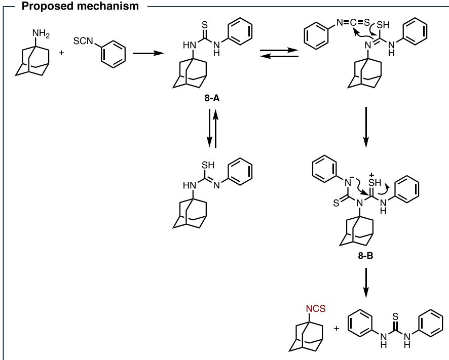
Figure 12. Synthesis of adamantyl isothiocyanate via a group metathesis.
