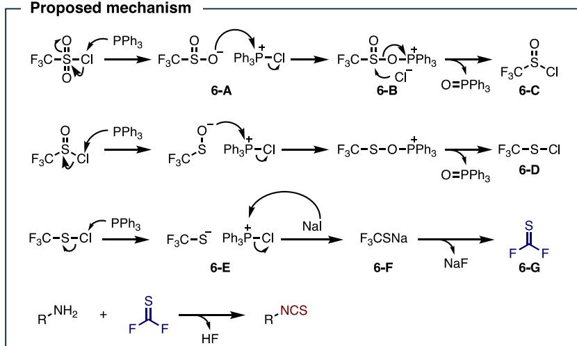
Figure 10. Isothiocyanation with utilizing CF_3SO_2Cl .
