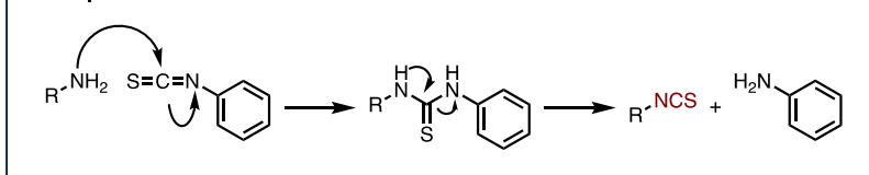
Figure 13. Isothiocyanation with phenyl isothiocyanate.
