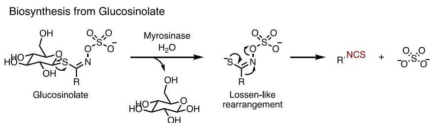
Figure 14. The mechanism of biosynthesis from glucosinolate.
