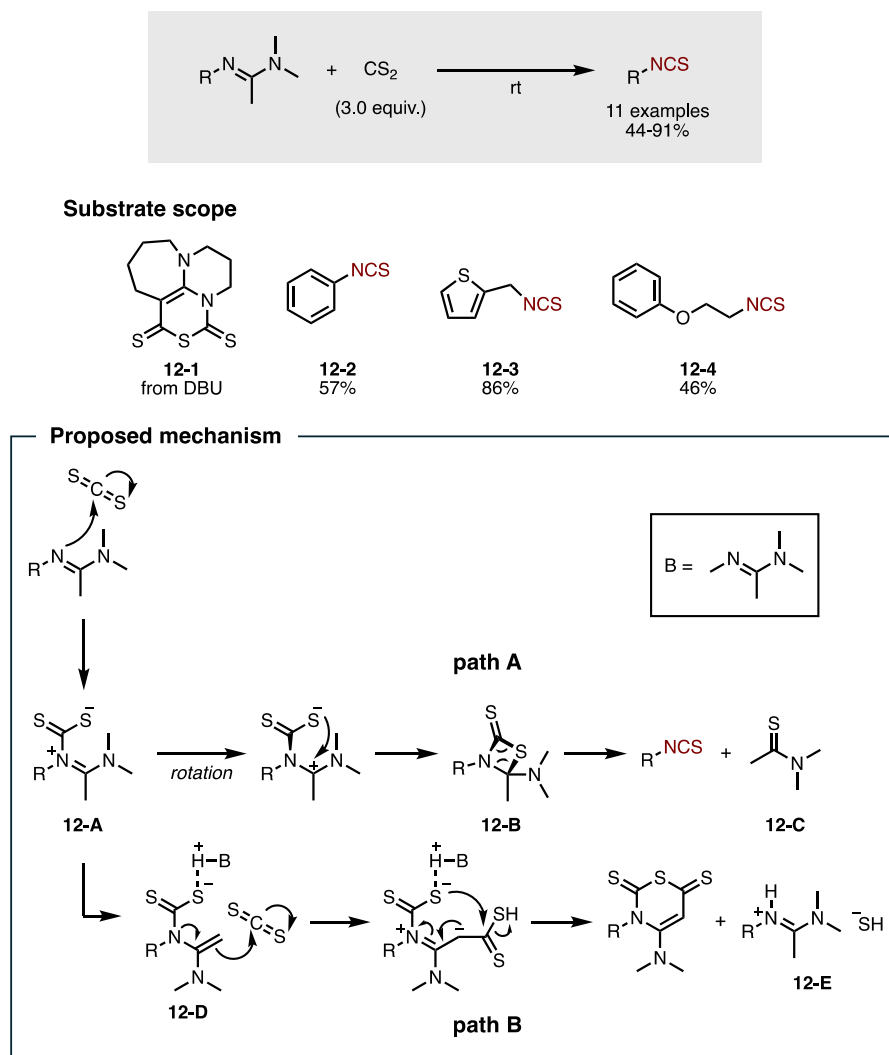
Figure 17. Isothiocyanation from acyclic amidines.
