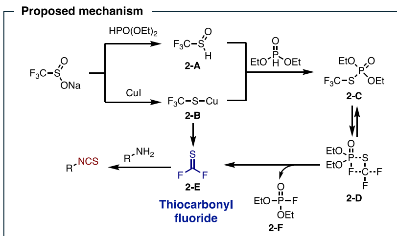
Figure 6. Copper-catalyzed isothiocyanation with the Langlois reagent.
