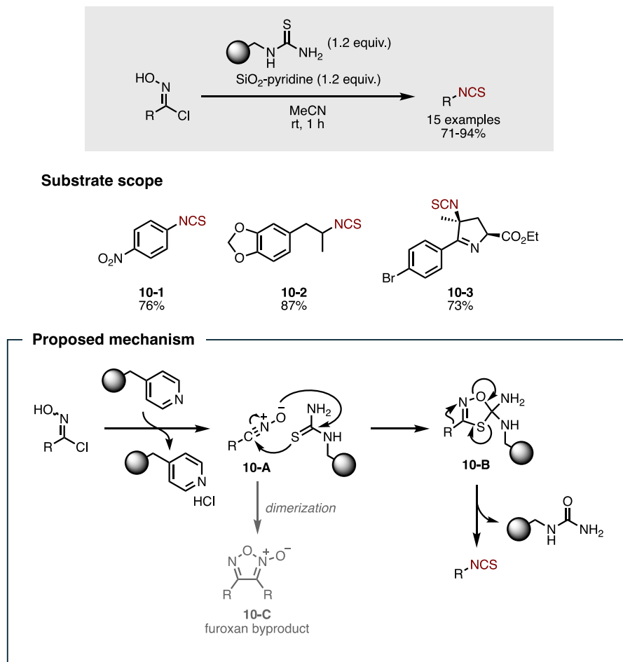
Figure 15. Isothiocyanation with an immobilized reagent.
