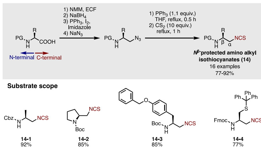
Figure 19. Synthesis of N β -protected amino alkyl isothiocyanates.
