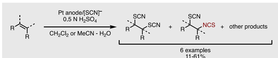
Figure 27. Electrochemical thiocyanation and isothiocyanation of alkenes.
