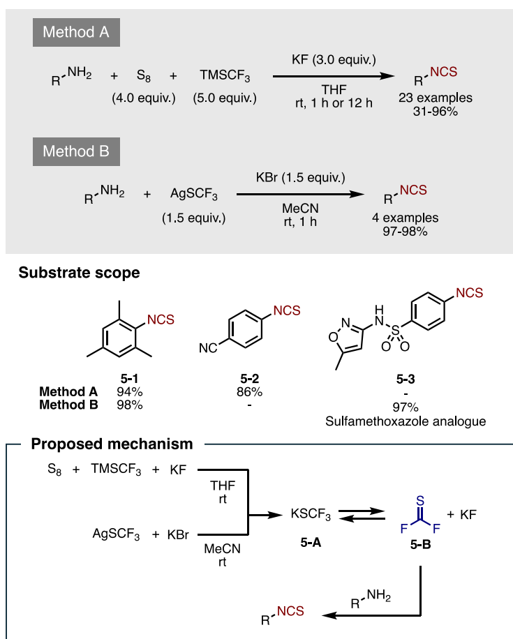
Figure 9. Isothiocyanation via thiocarbonyl fluoride from TMSCF 3 or AgSCF 3 .
