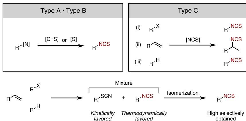
Figure 23. Examples of the starting materials in Type C.
