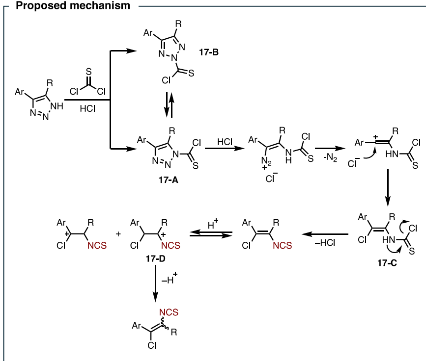
Figure 22. Synthesis of N -vinyl isothiocyanates from NH-1,2,3-triazoles.
