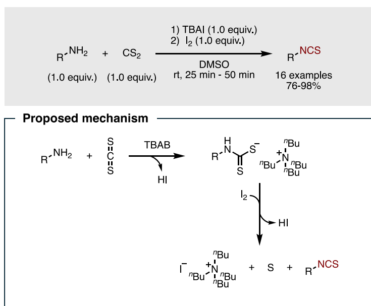
Figure 5. Synthesis of isothiocyanates with TBAI and iodine.
