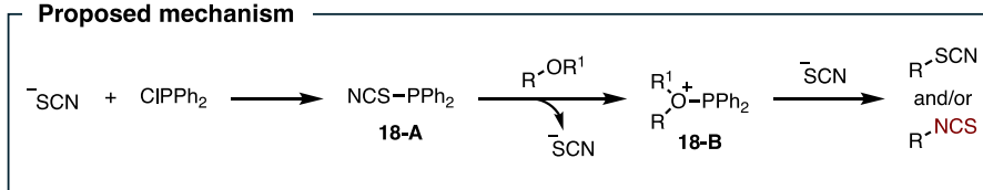
Figure 24. Isothiocyanation via substitution reaction.
