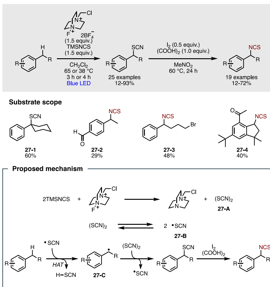
Figure 34. Photo-induced C–H thiocyanation and one-pot isothiocyanation.
