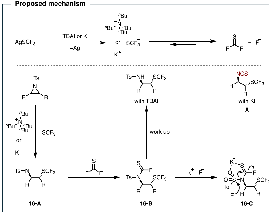
Figure 21. Synthesis of trifluoromethylthiolated isothiocyanates from aziridines.
