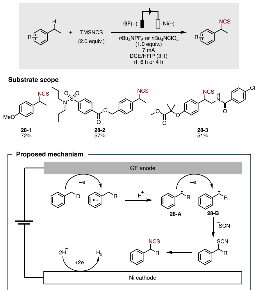
Figure 35. Electrochemical C–H isothiocyanation.
