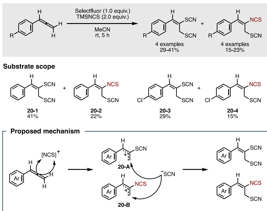
Figure 26. Difunctionalization of allenes by Selectfluor and TMSNCS.
