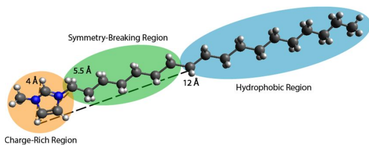
Figure 5. Structural domains that determine the T_m values of imidazolium-based ILs. Reproduced from Ref. 28 with permission from John Wiley and Sons.
