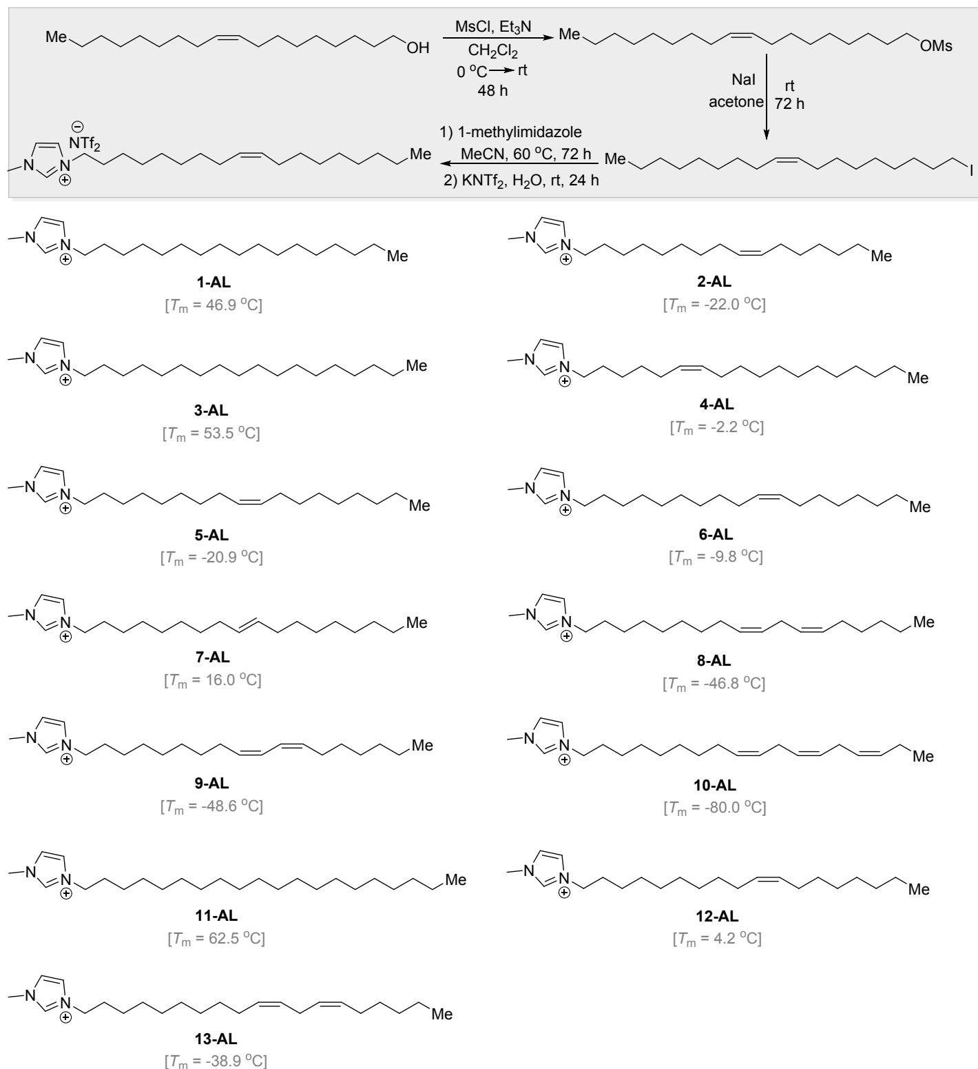
Figure 4. The four-step synthesis and structures of the ene-bearing lipid-like ILs along with their T_m values (The counter anion is \text{NTf}_2^- that was omitted for clarity). 19,20 Each of the ILs has a long alkyl appendage identical to that in a natural fatty acid.
