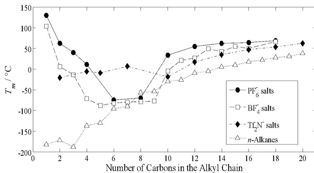
Figure 1. Effect of alkyl-chain length on melting point ( T_m ) in 1- n -alkyl-3-methylimidazolium salts and corresponding n -alkanes. Reproduced from Ref. 19 with permission from Jon Wiley and Sons.
