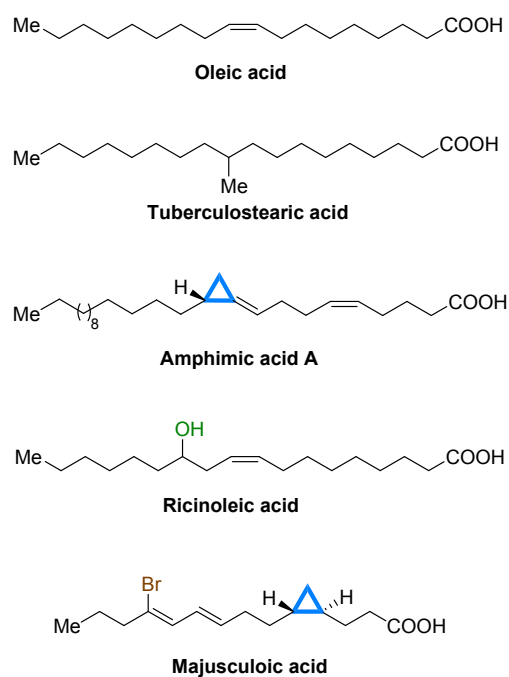
Figure 3. Examples of naturally occurring fatty acids containing mid-chain motifs that induce structural kinking. Kinking is responsible for the T_m depression effect.
