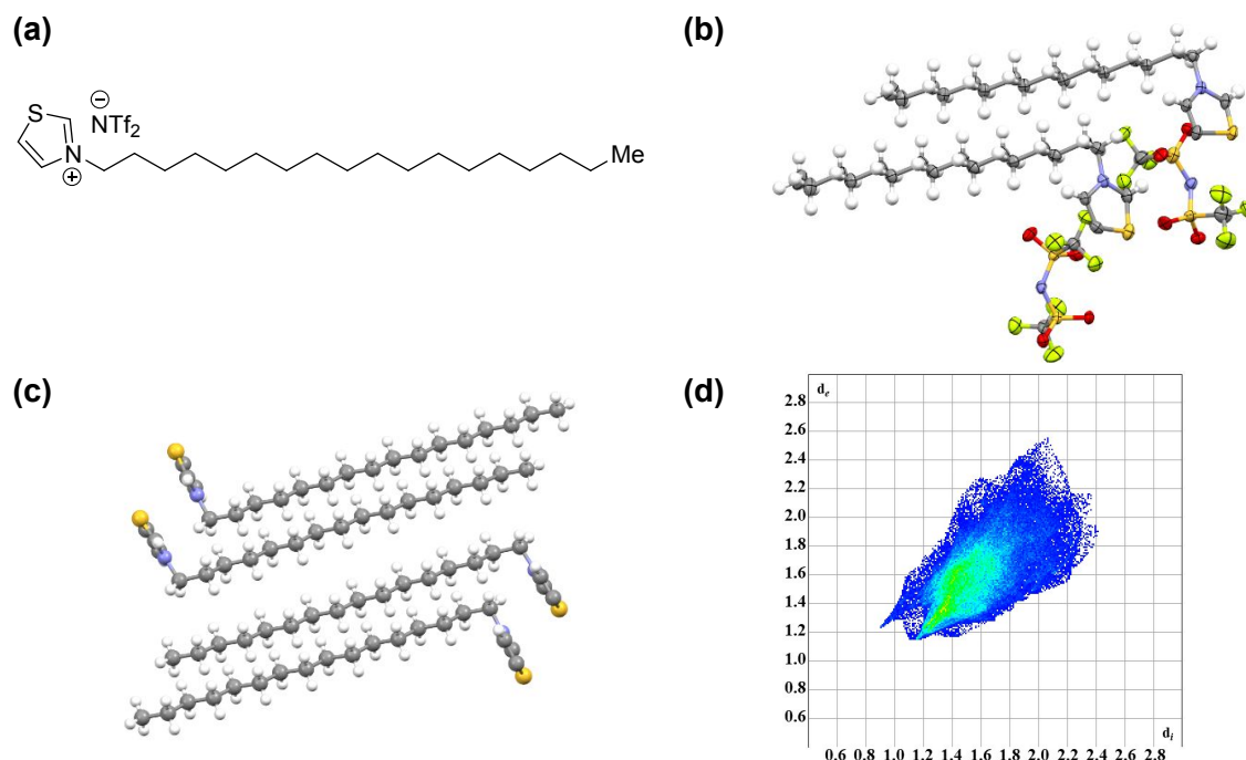
Figure 11. Structure and asymmetric unit of [C 16 -Thia][NTf 2 ] (a and b). Packing diagram of [C 16 -Thia][NTf 2 ] showing alkyl-alkyl stacking (c). Interaction fingerprint of [C 16 -Thia][NTf 2 ] showing a large percentage of H...H interactions (green portion) (d). Reprinted with from Ref. 83 with permission from the Elsevier.
