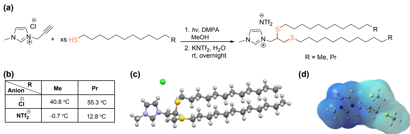
Figure 7. (a) Synthesis of the thioether-based ILs using the thiol–yne reaction. (b) Comparison of T_m of the ILs paired with Cl^- and NTf_2^- anions with an equivalent chain length of C_{16} and C_{18} . (c) Crystal structure of the thioether-based lipidic IL with chloride anion and C_{16} tails. (d) The electrostatic potential energy map of the thioether-based imidazolium cation. The boundary between hydrophilic/hydrophobic domains can be clearly observed, showing that sulfur atoms are located in the hydrophobic domain. Reprinted with from Ref. 43,44 with permission from the Royal Society of Chemistry and Elsevier.
