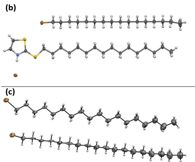
Figure 12. (a) the serendipitous discovery of ionic cocrystallization system using 2-mercaptobenzothiazolium-based lipid-like ILs, leading to the first report of crystal structures of long-chain 1-bromoalkanes. Asymmetric units of the IL crystallized with 1-bromohexadecane (b) and 1-bromooctadecane (c) shown with 50% probability ellipsoids. Reprinted with from Ref. 91 with permission from the Royal Society of Chemistry.
