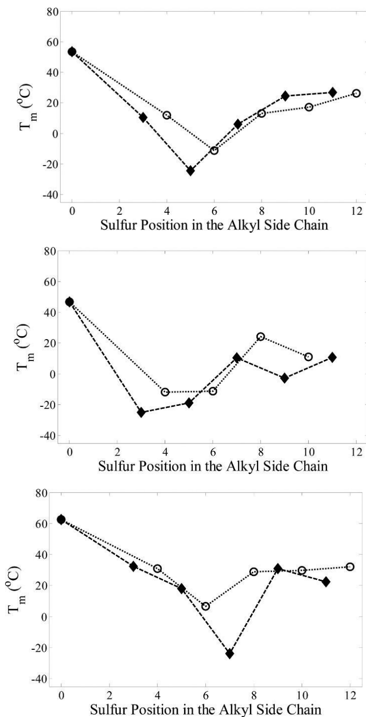
Figure 6. T_m values of the 1-thiaalkyl-3-methylimidazolium-based ILs with an equivalent chain length of C16 (top), C18 (middle) and C20 (bottom) as a function of the position of the sulfur in the chain. The odd ( \blacklozenge )/even ( \circ ) sulfur positions have been plotted separately to help distinguish trends. Reprinted from Ref. 39 with permission from American Chemical Society.
