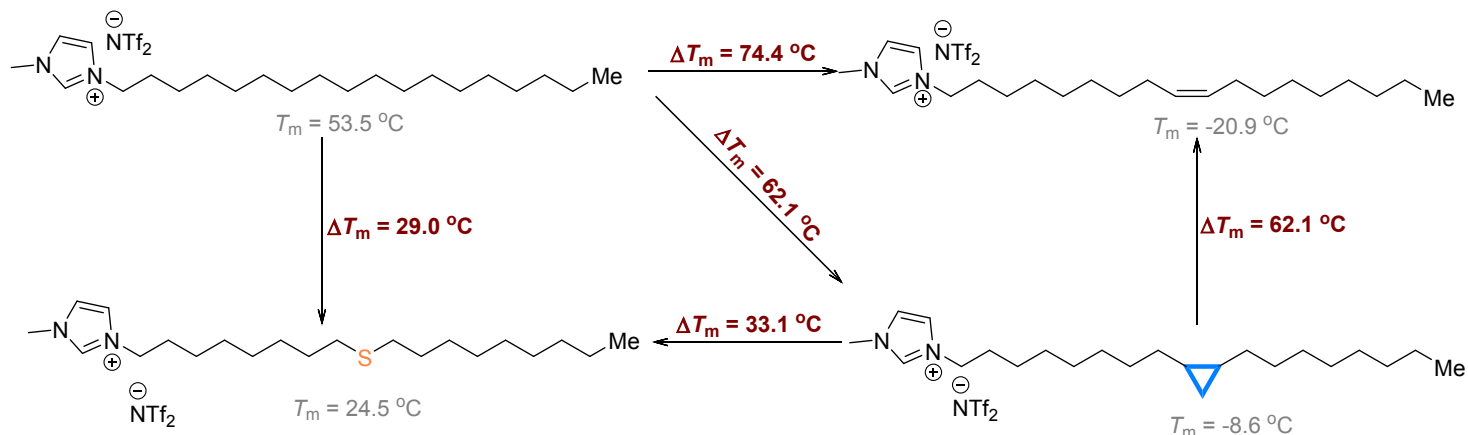
Figure 10. Comparative \Delta T_m values among three generations of lipid-like \text{C}_{18} -based ILs.
