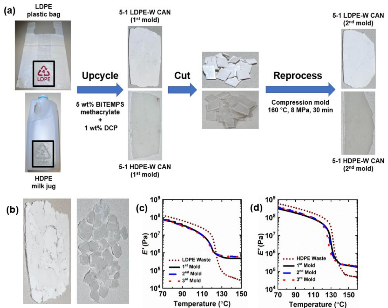
Figure 10. (a) Preparation route and reprocessing of PE-W CANs from plastic bags and a milk jug. (b) (left) Unhealed LDPEX-W film. (right) Unhealed HDPEX-W film. (c)/(d) Tensile storage modulus ( E' ) as a function of temperature of 1 st mold, 2 nd mold, and 3 rd mold (c) 5-1 LDPE-W CAN and (d) 5-1 HDPE-W CAN samples with their PE waste precursor counterparts.
