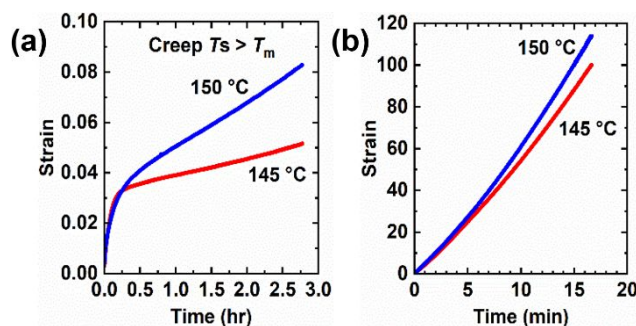
Figure 8. Creep curves at different temperatures above the melt transition of (a) 5-1 HDPE CANs and (b) HDPE under a constant shear stress of 3 kPa.
