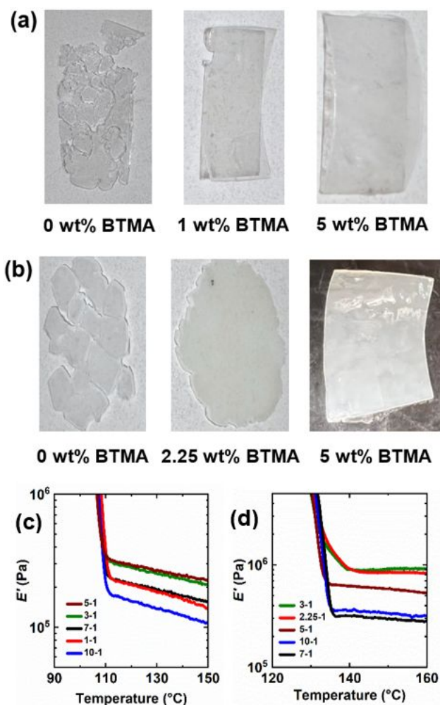
Figure 1. (a) Films of LDPE CANs synthesized with 1 wt% DCP and (left to right) 0 wt%, 1 wt%, and 5 wt% BiTEMPS methacrylate cross-linker. (b) Films of HDPE CANs synthesized with 1 wt% DCP and (left to right) 0 wt%, 2.25 wt%, and 5 wt% BiTEMPS methacrylate cross-linker. (c)/(d) Tensile storage modulus ( E' ) as a function of temperature and BiTEMPS methacrylate loading (wt%) for (c) LDPE CANs and (d) HDPE CANs. Legends are read as “BiTEMPS methacrylate wt%”-“DCP wt%”.
