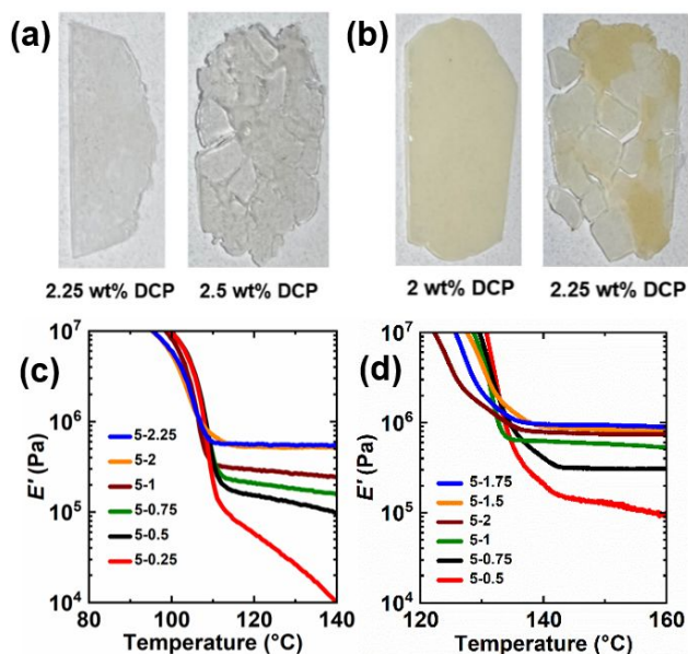
Figure 2. (a) Films of LDPE CANs synthesized with 5 wt% BiTEMPS methacrylate cross-linker and (left to right) 2.25 wt% and 2.5 wt% DCP. (b) Films of HDPE CANs synthesized with 5 wt% BiTEMPS methacrylate cross-linker and (left to right) 2 wt% and 2.25 wt% DCP. (c)/(d) Tensile storage modulus ( E' ) as a function of temperature and DCP loading (wt%) for (c) LDPE CANs and (d) HDPE CANs. Legends are read as “BiTEMPS methacrylate wt%”-“DCP wt%”.
