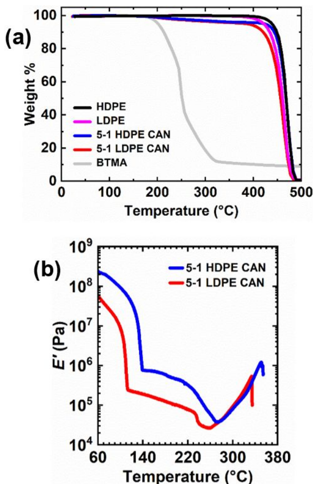
Figure 5. (a) Weight losses as a function of temperature given by TGA for BiTEMPS methacrylate (BTMA), PE, and 5-1 PE CANs. (b) E' as a function of temperature to monitor thermal stability and property degradation in 5-1 PE CANs at high temperatures.
