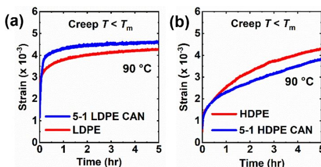
Figure 6. Creep curves of (a) LDPE and 5-1 LDPE CAN as well as (b) HDPE and 5-1 HDPE CAN at 90 °C under a constant shear stress of 3 kPa.
