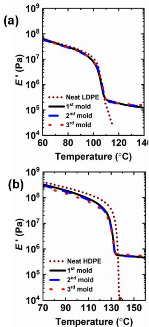
Figure 4. Tensile storage modulus ( E' ) as a function of temperature of 1 st mold, 2 nd mold, and 3 rd mold (a) 5-1 LDPE CAN and (b) 5-1 HDPE CAN samples with their neat counterparts.
