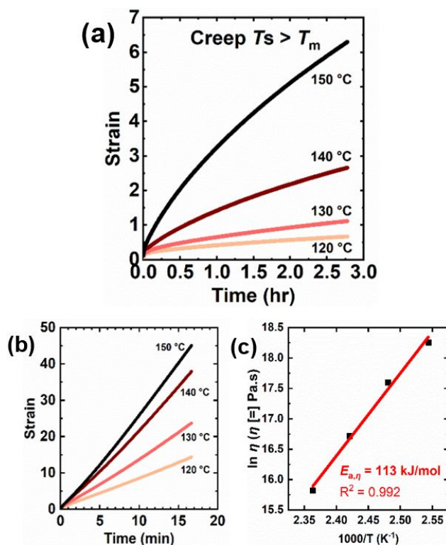
Figure 7. Creep curves at different temperatures above the melt transition of (a) 5-1 LDPE CANs and (b) LDPE under a constant shear stress of 3 kPa. (c) Arrhenius activation energy of viscosity for 5-1 LDPE CANs as calculated from creep data taken over a T -range of 120-150 °C.
