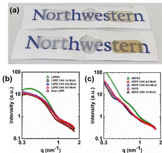
Figure 9. (a) Image of molten PE samples at 165 °C. Samples were placed on logos to aid visualization of transparency. Top row, left to right: Neat LDPE, LDPEX, LDPE CAN; Bottom row, left to right: Neat HDPE, HDPEX, HDPE CAN. (b) SAXS patterns of semi-crystalline LDPE-based samples. (c) SAXS patterns of semi-crystalline HDPE-based samples.
