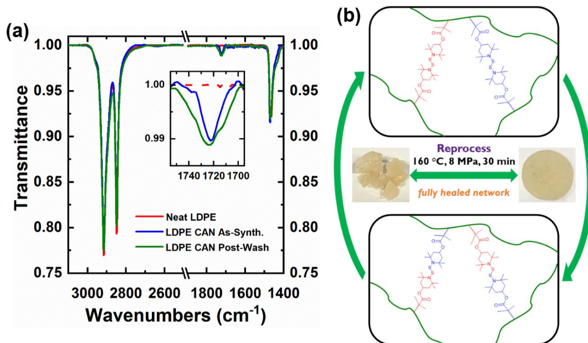
Figure 3. (a) FTIR spectrum of neat LDPE and 5-1 LDPE CANs before and after washing in boiling xylene. Carbonyl stretch at \sim 1725\text{ cm}^{-1} indicates successful grafting of BiTEMPS methacrylate during reactive processing. (b) Dissociative exchange of disulfide linkages during reprocessing of PE CANs.
