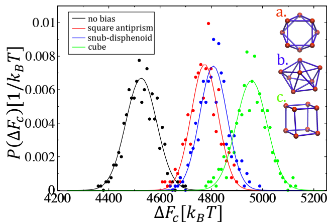
Fig. 6 Normalized distributions of the LVs excess curvature energy, \Delta F_c , defined in the text, for n = 8 . (a-c) correspond to the cases of an LV with JNPs adhering into an antiprism, snub-disphenoid and cubic nanocluster, respectively.
