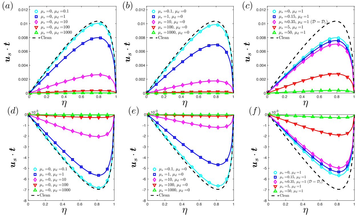
Fig. 10 Tangential component of the surface velocity u_s \cdot t as a function of the drop surface parameter \eta for the prolate 'A' drop in figure 3a with Ca_E = 0.3 (a-c), and for the prolate 'B' drop in figure 3b with Ca_E = 0.4 (d-f). (a, d) Sole influence of surface dilatational viscosity ( \mu_s = 0 ); (b, e) Sole influence of surface shear viscosity ( \mu_d = 0 ); (c, f) Combined influence of surface viscosities with \mu_d = 1 . In all panels, the dashed curves denote the clean drop case.
