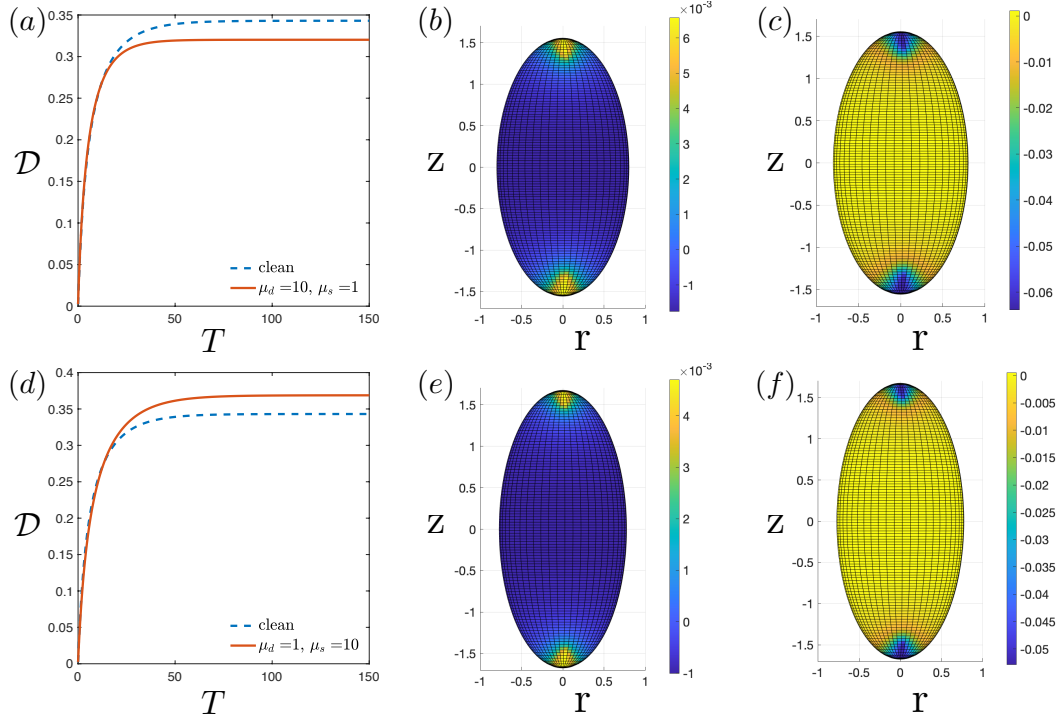
Fig. 8 (a, d) Deformation as a function of dimensionless time; (b, e) surface dilatation, \Theta = \nabla_s \cdot \mathbf{u}_s , and (c, f) surface deformation, T_{\xi\xi}^S for the prolate 'B' drop in figure 3b. The top row represents the case with \mu_d = 10, \mu_s = 1 ( \mathcal{D}/\mathcal{D}_c < 1 ), and the bottom row represents the case with \mu_d = 1, \mu_s = 10 ( \mathcal{D}/\mathcal{D}_c > 1 ). The colormaps show the magnitude and distribution of the surface dilatation and surface deformation. The electric capillary number Ca_E = 0.4 , and the surface dilatation and surface deformation correspond to T = 150 .
