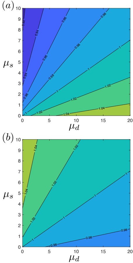
Fig. 4 Deformation phase plane for (a) the prolate 'A' and (b) prolate 'B' drops in figures 3(a,b). The contour line \mathcal{D}/\mathcal{D}_c = 1 denote the boundary between regions of higher and lower deformations compared to the clean drop. The electric capillary number Ca_E = 0.2 .
