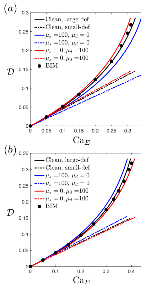
Fig. 3 Equilibrium deformation \mathcal{D} as a function of the electric capillary number for (a) a prolate 'A' drop with \mu_r = 1 , \sigma_r = 0.1 , \epsilon_r = 10 and (b) a prolate 'B' drop with \mu_r = 1 , \sigma_r = 0.04 , \epsilon_r = 1/50 . In (a,b), the solid curves represent results from the large deformation analysis (large-def), the dashed curves represent results from the small deformation analysis (small-def) in 47 , and the symbols denote boundary integral method simulations for a clean drop 12 . In both panels, the curves are color-coded to denote the sole-effect of dilatational viscosity (red), shear viscosity (blue) and the clean drop case (black).
