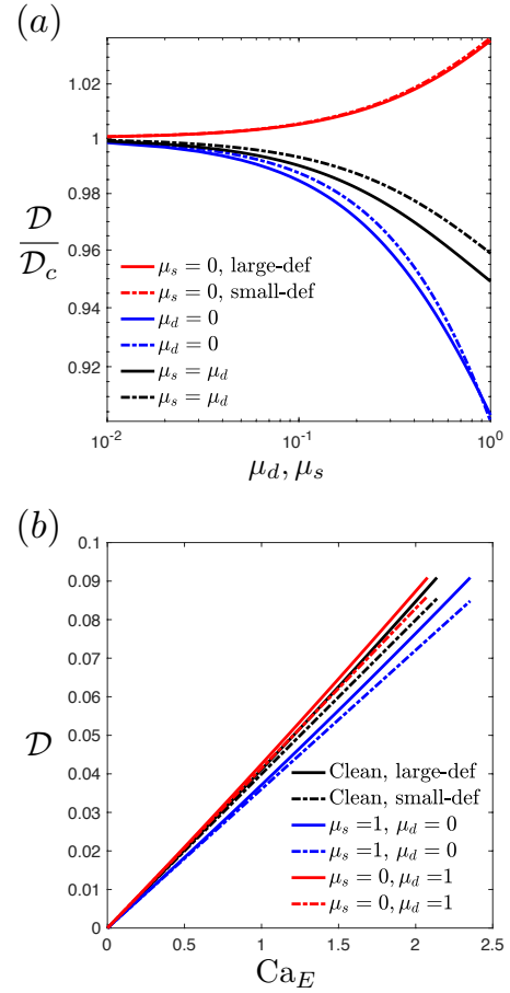
Fig. 2 (a) Equilibrium \mathcal{D} deformation scaled by the clean drop deformation \mathcal{D}_c as a function of the dilatational and shear viscosities for \text{Ca}_E = 0.2 . The curves are color-coded to denote the sole-effect of dilatational viscosity (red), shear viscosity (blue) and their combined effect (black). (b) Equilibrium deformation \mathcal{D} as a function of electric capillary number. The curves are color-coded to denote the sole-effect of dilatational viscosity (red), shear viscosity (blue) and the clean drop case (black). In both panels, the solid curves represent results from the large deformation analysis (large-def) and the dashed curves represent results from the small-deformation analysis (small-def) in 47 . Other parameters are: \mu_r = 1/1.4706 , \sigma_r = 1/1.25 , \varepsilon_r = 1/1.0566 .
