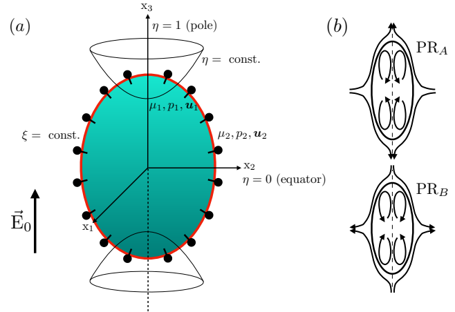
Fig. 1 (a) Sketch of the problem: An axisymmetric leaky dielectric viscous drop immersed in another dielectric fluid, with an external electric field \vec{E}_0 in the z direction. The bead-rod particles represent the rheological properties of the interface (shear and dilatation). (b) Two modes of prolate shape exist: prolate ‘A’ (PR A ) with a counterclockwise circulation in the first quadrant, and prolate ‘B’ (PR B ) with a clockwise circulation in the first quadrant.
