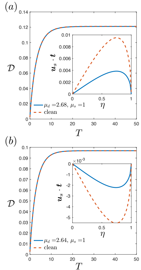
Fig. 5 Deformation number as a function of dimensionless time for (a) the prolate 'A' and (b) prolate 'B' drops in figures 3(a,b). The dashed and solid lines denote the clean and surface viscosities influenced drops, respectively. The insets show the tangential component of the surface velocity as a function of the drop surface parameter \eta . The electric capillary number Ca_E = 0.2 .
