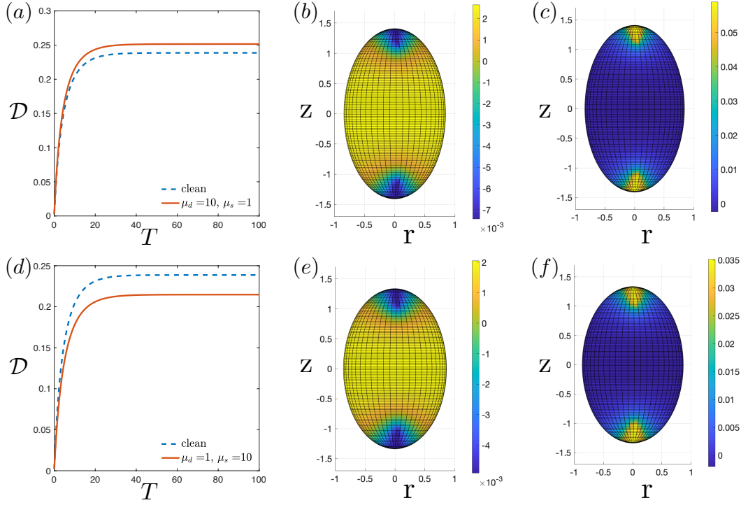
Fig. 7 (a, d) Deformation as a function of dimensionless time; (b, e) surface dilatation, \Theta = \nabla_s \cdot \mathbf{u}_s , and (c, f) surface deformation, T_{\xi\xi}^S for the prolate 'A' drop in figure 3a. The top row represents the case with \mu_d = 10, \mu_s = 1 ( \mathcal{D}/\mathcal{D}_c > 1 ), and the bottom row represents the case with \mu_d = 1, \mu_s = 10 ( \mathcal{D}/\mathcal{D}_c < 1 ). The colormaps show the magnitude and distribution of the surface dilatation and surface deformation. The electric capillary number Ca_E = 0.3 , and the surface dilatation and surface deformation correspond to T = 100 .
