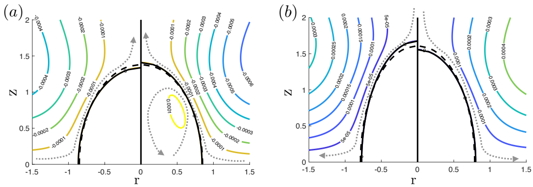
Fig. 9 Drop shapes and streamlines (a) for the prolate ‘A’ drop in figure 3a with Ca_E = 0.3 , and (b) for the prolate ‘B’ drop in figure 3b with Ca_E = 0.4 . In each panel, the left-half shows the shape with \mu_s = 10 , \mu_d = 1 , and the right-half shows the shape with \mu_s = 1 , \mu_d = 10 . In both panels, the dashed curve denotes the clean drop shape. Numbers on the streamline denote the magnitude of the flow, while the dotted lines show the direction of the flow.
