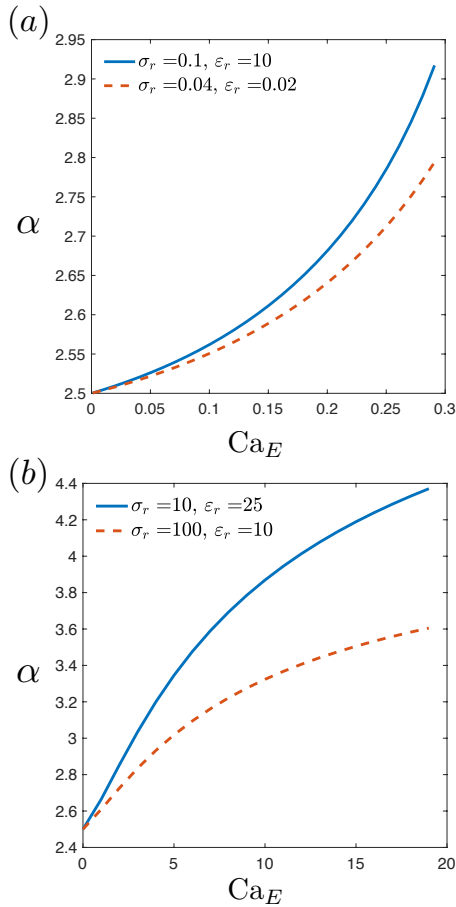
Fig. 11 Critical ratio \alpha from equation 42 as a function of the electric capillary Ca_E . Blue ( \diamond ) curves denote prolate 'A' drops, and red ( \circ ) curves denote prolate 'B' drops. The electric parameters are chosen such that the drops (a) ultimately breakup past a critical Ca_E or (b) keep deforming with larger values of Ca_E 12 . The viscosity ratio \mu_r = 1 .
