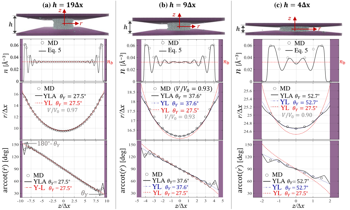
Fig. 2 Continuum descriptions and MD simulations of nanoscale water bridges: (a) h = 19\Delta x \simeq 6.65 nm ( V/V_0 = 0.97 ), (b) h = 9\Delta x \simeq 3.15 nm ( V/V_0 = 0.93 ), and (c) h = 4\Delta x \simeq 1.4 nm ( V/V_0 = 0.9 ). The MD simulations are performed with N = 12,000 water molecules, which corresponds to the reference volume V_0 = N/n_b = 0.37 zL with n_b = 0.0322 Å -3 . Top panels are time snapshots from MD simulations, the graphs report the number density n(z) , bridge radius r(z) , and interface angle \text{arccot}(\dot{r}) . Analytical estimates from eqn (5) are obtained using the model parameters reported in Table 1. Continuum model predictions (see legend) correspond to numerical solutions of eqns (1)-(2): the augmented model (YLA) and the conventional Y-L equation (YL) using a variable and fixed Young contact angle.
