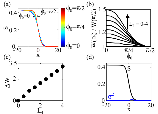
Fig. 1 Nematic-isotropic interface for varying anchoring angle, 0 < \phi_0 < \pi/2 . (a) Plots of nematic order parameter S versus position for L_4 = 4 and varying \phi_0 , represented by the different colors. As the anchoring angle goes from homeotropic to tangential, the width of the interface decreases. (b) Interface width as a function of anchoring angle, normalized by the width at \phi_0 = \pi/2 . Each curve represents a different value of L_4 , with L_4 increasing with width disparity. (c) Width difference \Delta W = W(\phi_0 = 0) - W(\phi_0 = \pi/2) versus L_4 . The linear relationship indicates that anchoring energy is proportional to L_4 . (d) Nematic order, S , and biaxiality parameter, \sigma^2 , across the interface for L_4 = 4 and \phi_0 = \pi/2 . There is some biaxiality at the interface, though not large in magnitude.
