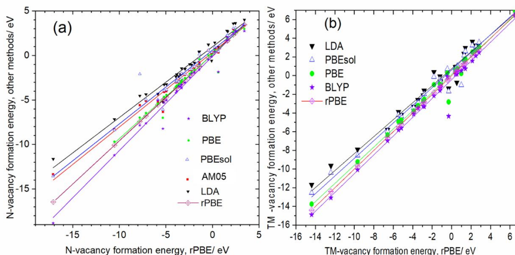
Figure 6. Correlation between (a) N-vacancy and (b) TM vacancy formation formation energy calculated using LDA, AM05, BLYP, PBE, and, PBEsol with those computed using the rPBE method.
