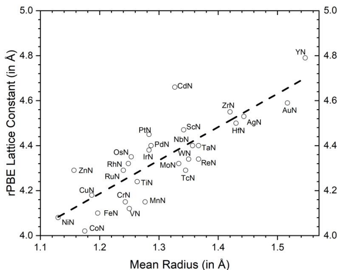
Figure 2. Correlation between the lattice constant of TMNs and mean radii of the corresponding TMs present in TMNs.
