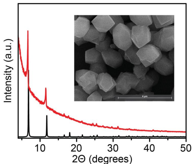
Figure 3 Powder X-ray diffractogram (PXRD) of Co-MOF-74 synthesized on the ATR chip (red) and simulated PXRD of Co-MOF-74 (black). The inset shows a Scanning electron microscopy image of \text{Co}_2(\text{dobdc}) of the same sample.
