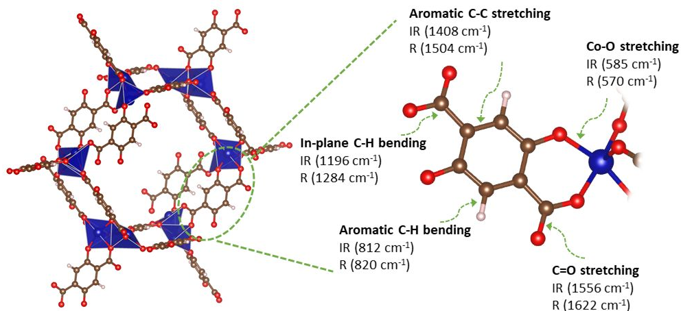
Figure 1 A molecular representation of the \text{Co}_2(\text{dobdc}) . The red balls represent oxygen atoms, brown for carbon atoms, pale pink for hydrogen atoms, and blue for cobalt atoms. Also shown are the linker molecule and the relevant vibrational modes for Raman and Infrared spectroscopy.
