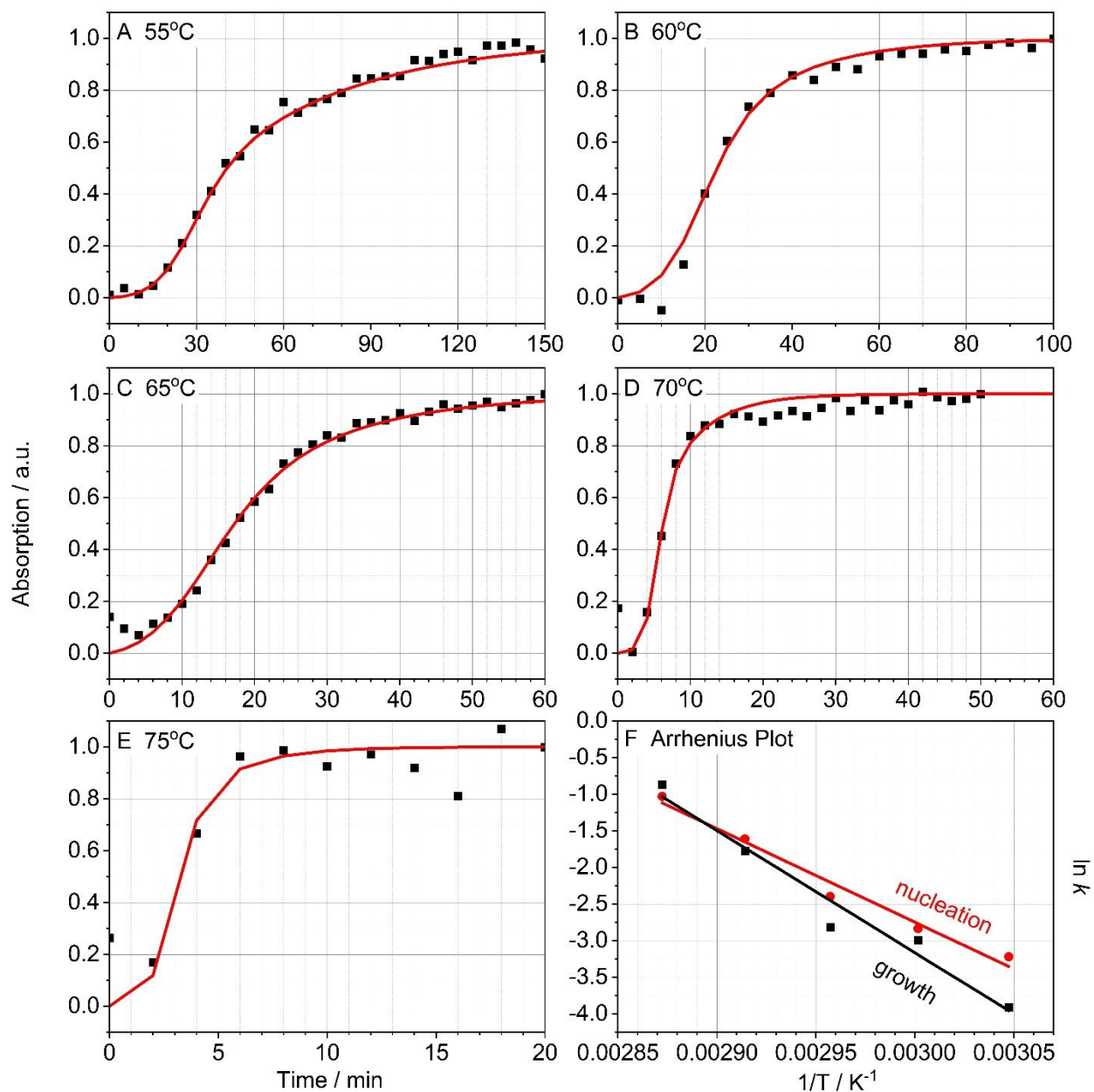
Figure 6 Gualtieri model fitting (red curves) for the reaction kinetics traced by absorption intensity of 580 cm^{-1} (black symbols) as a function of time at temperatures of (A) 55 °C, (B) 60 °C, (C) 65 °C, (D) 70 °C, (E) 75 °C. (F) Arrhenius Plots for nucleation (red) and growth (black) extracted from rate constants derived from the fitted parameters shown in (A) – (E).
