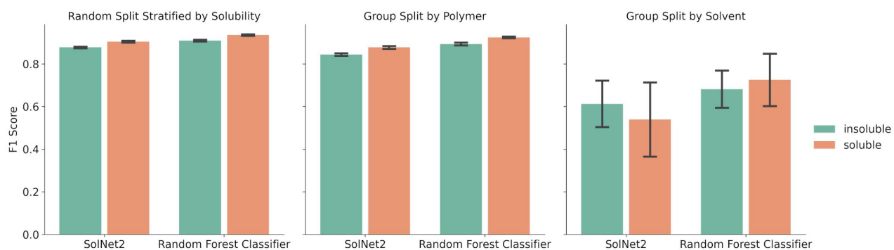
Fig. 3 Average F1 score of SolNet2 infrastructure neural network and Random Forest Classifier models for soluble and insoluble classification using structural fingerprint for solvents. Five-fold cross validation splits were chosen using either a random split stratified by solubility (left), group split by polymer (middle), or group split by solvent (right). Error bars represent the standard deviation for the F1 score of those splits.
