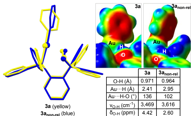
Fig. 5 Left: Structure overlay for 3a/3a non-rel . Right top: The insets show cropped ESP maps for 3a and 3a non-rel (color scale: red, -0.04 au; blue, 0.025 au; surface isovalue of 0.005 au). Right bottom: Table providing selected computational structural and spectral data.
