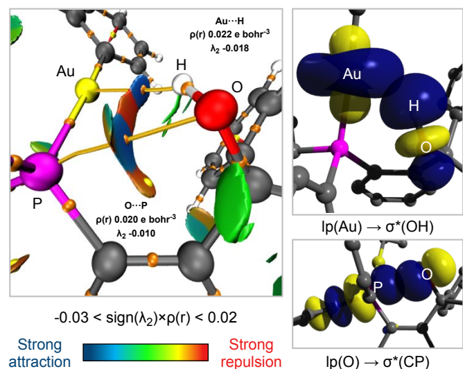
Fig. 4 Left: AIM/NCI plot of 3a with gradient isosurface of 0.3 au. Right: Selected NBOs for lp(\text{Au}) \rightarrow \sigma^*(\text{OH}) and lp(\text{O}) \rightarrow \sigma^*(\text{CP}) interactions in 3a .
