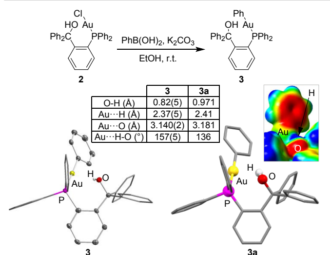
Fig. 3 Top: Reaction scheme for synthesis of 3 . Bottom: Crystal structure of 3 and its optimized geometry ( 3a ). Hydrogens other than OH omitted for clarity. Thermal ellipsoids drawn at 50% probability, and phenyl groups drawn as thin lines. Inset shows cropped ESP map for 3a (color scale: red, -0.04 au; blue, 0.025 au; surface isovalue of 0.005 au).
