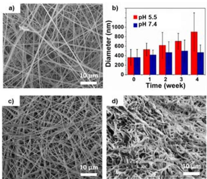
Fig. 3 (a) SEM image of nanofibers prior to incubation in aqueous solution. (b) Change in fiber diameter as a function of time and buffer pH (N=3). (c) SEM image of nanofibers after incubation for four weeks in pH 7.4 PBS and (d) after four weeks in pH 5.5 aqueous buffer.
