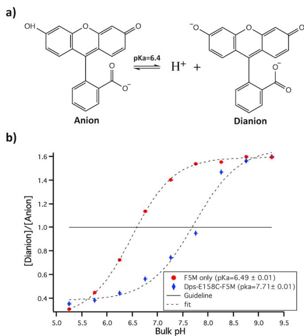
Figure 5. a) Scheme showing the acid dissociation of the pH sensitive dye fluorescein to form the anion and dianion forms. b) The ratio of absorbance at 490 nm (dianion) and 453 nm (anion) at varying pH was used to determine the pKa of free fluorescein-5-maleimide dye (F5M) and F5M conjugated at E158C residue of Dps interior cavity. A calculated pKa of 6.49 \pm 0.01 was obtained for free F5M dye whereas pKa of 7.71 \pm 0.01 was obtained for Dps-E158C-F5M cage suggesting local pH inside Dps is significantly different than bulk pH.
