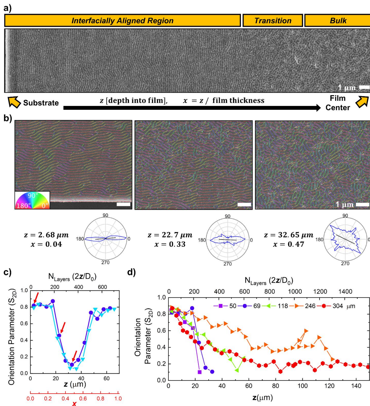
Fig. 3 Analysis of lamellar orientation from cross-sectional SEM images for a series of thick PS-b-PLA BBCP films. (a) From left to right edge: a stitched series of contrast-enhanced cross-sectional SEM images spanning the region from the film surface (substrate interface) to the film center (bulk) for a 69 \mu\text{m} thick film. (b) Individual SEM images taken at different depths into the film, overlaid with colored fibers indicating local domain orientation. Each SEM image covers a region of 8.47 \mu\text{m} \times 6.35 \mu\text{m} and is aligned such that the bottom boundary of the image is parallel to the substrate interface. Film depth is labeled in terms of distance from the substrate interface to the center of the image in both microns ( z ) and dimensionless units ( x = z/\text{film thickness} ). Pole figures are plotted from the orientation distribution of the colored fibers shown. (c) Calculated 2D orientation parameter plotted versus scan depth for non-overlapping cross-sectional scan trajectories on the 69 \mu\text{m} thick film. The number of layers ( N_{\text{Layers}} ) labeled above is determined with respect to the average lamellar d-spacing ( D_0 ) determined by SAXS. (d) Orientation parameter versus scan depth for a series of samples with varying film thickness. For visual clarity, data are shown only until the midpoint of each film and connected by straight lines.
