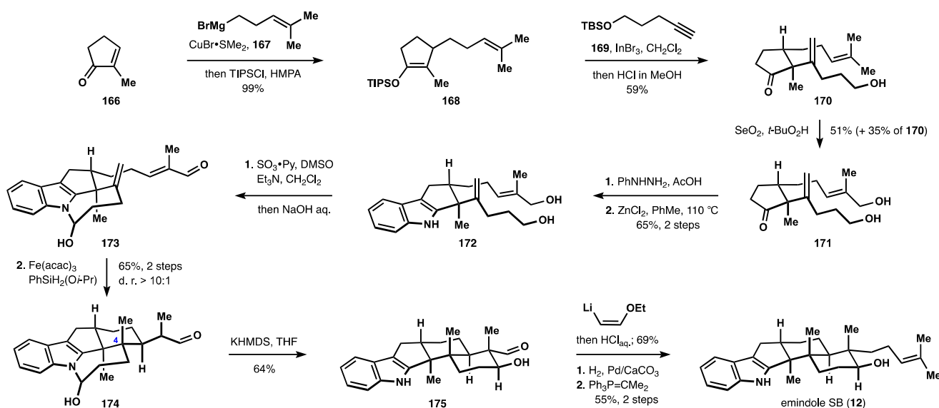
Scheme 18. The Pronin synthesis of emindole SB (12).
