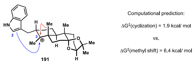
Figure 2. Computational evaluation of a biomimetic Friedel-Crafts cyclization.
