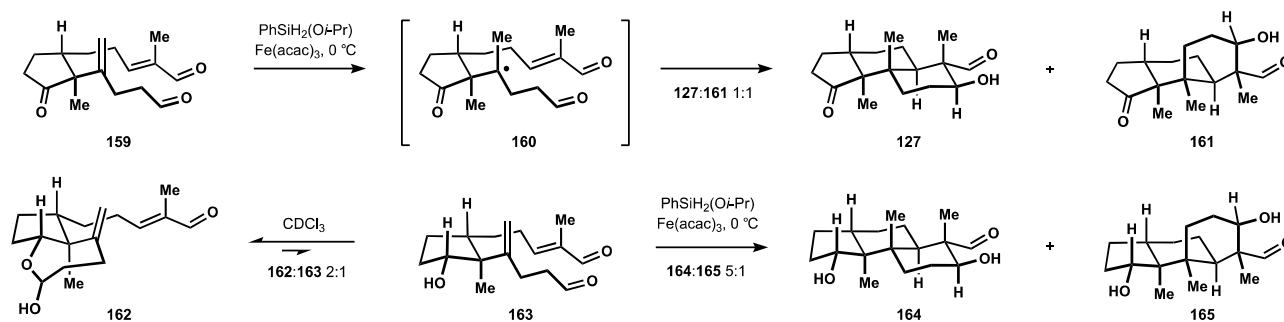
Scheme 17. HAT-initiated polycyclization en route to the tricyclic terpenoid core.
