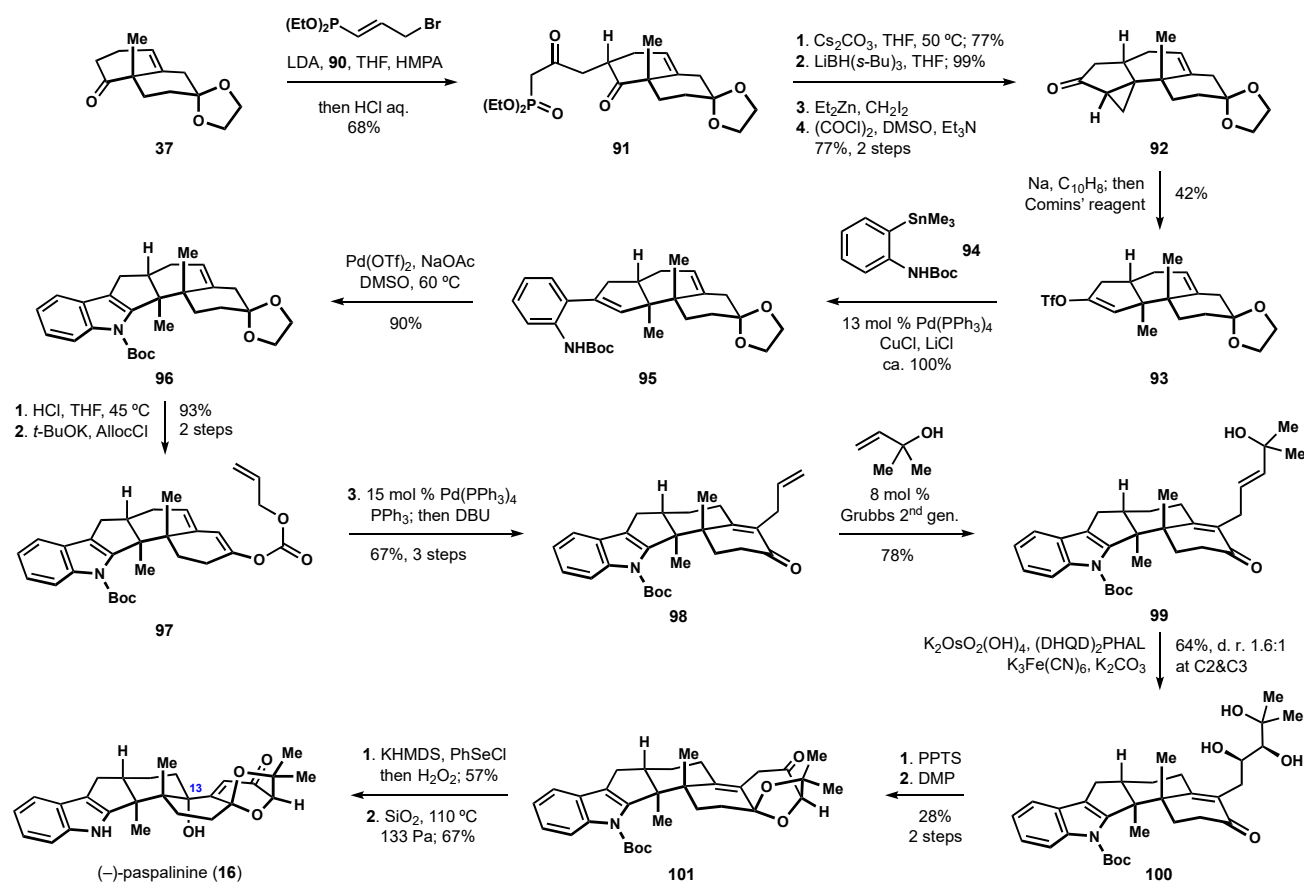
Scheme 10. The Kuwahara synthesis of (-)-paspalinine ( 16 ).
