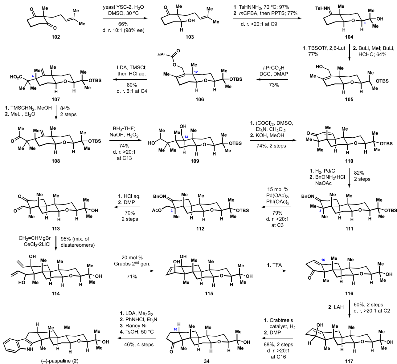
Scheme 11. The Johnson synthesis of (-)-paspaline (2).
