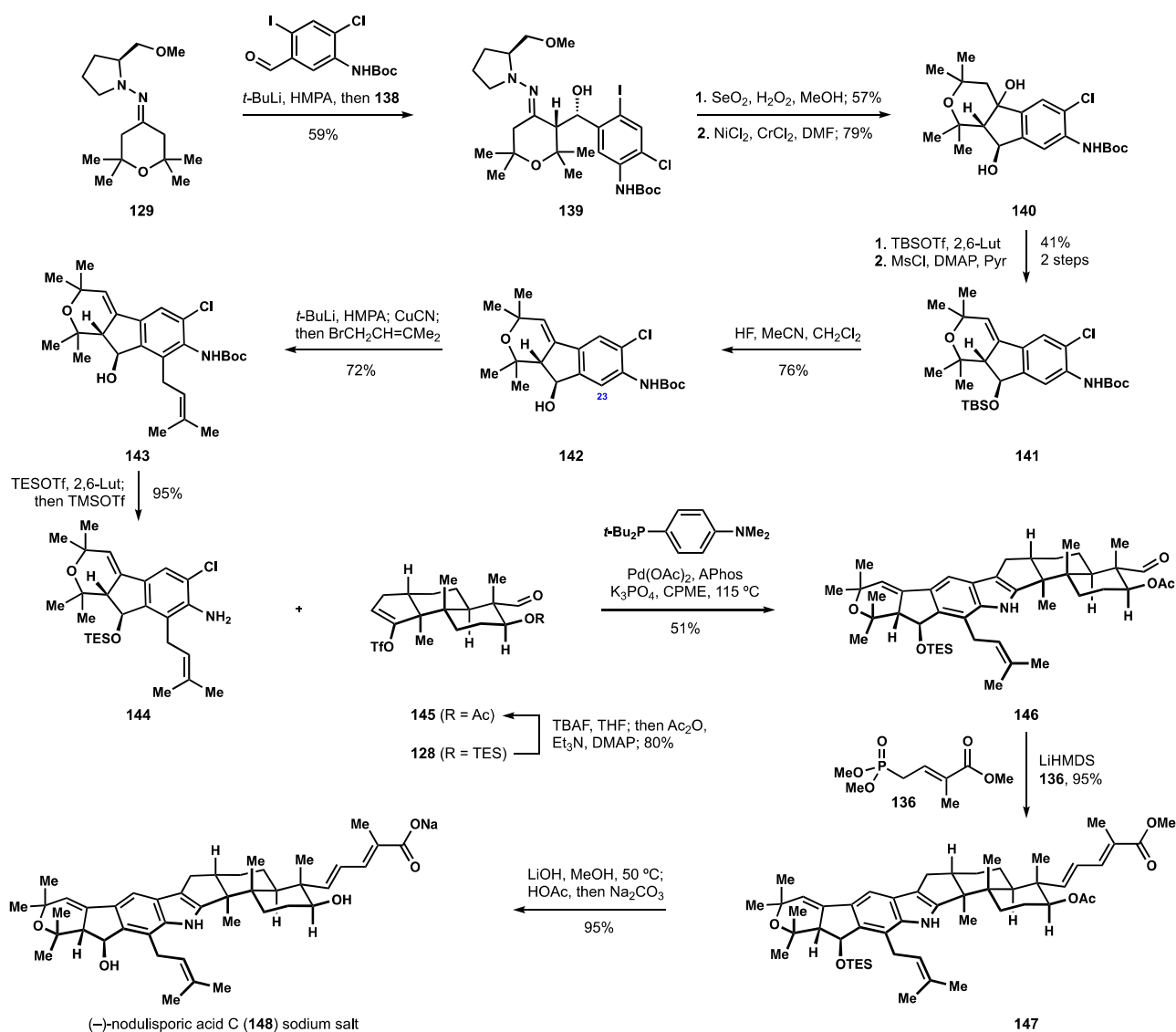
Scheme 15. The Smith synthesis of (-)-nodulisporic acid C ( 148 ).
