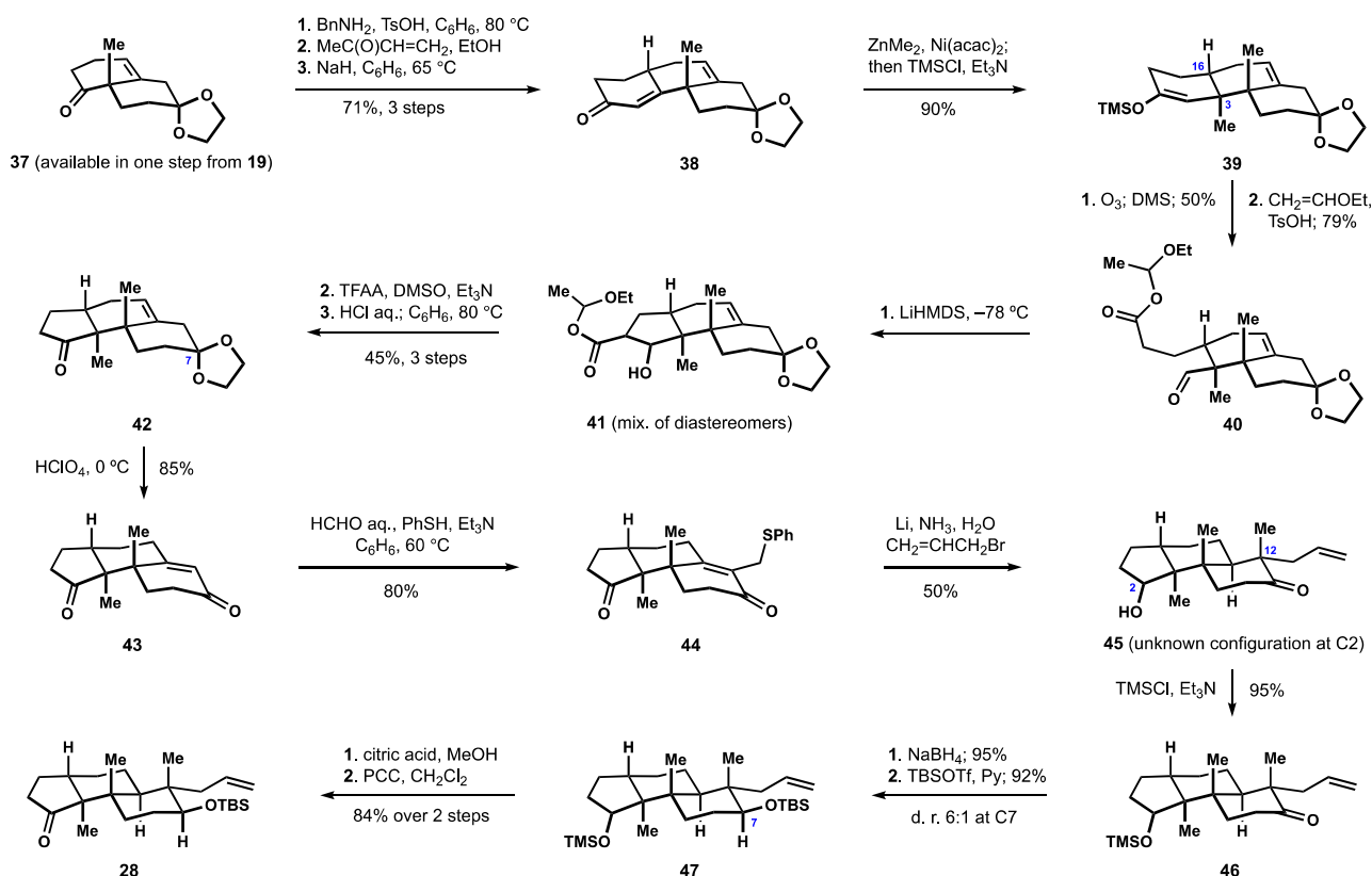
Scheme 4. Revised synthesis of the tricyclic terpenoid motif by the Smith group.
