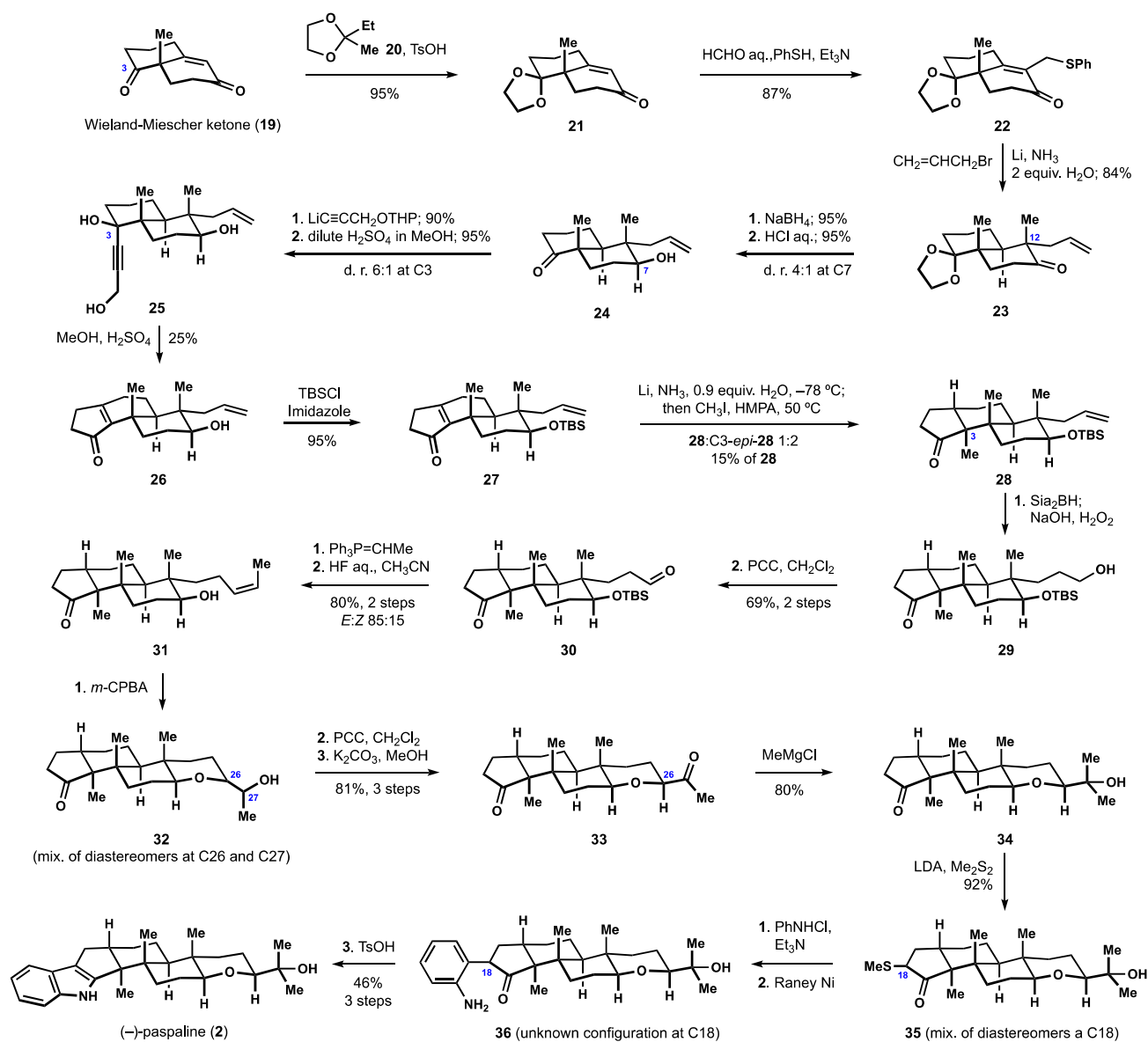
Scheme 3. The Smith synthesis of (-)-paspaline (2).
