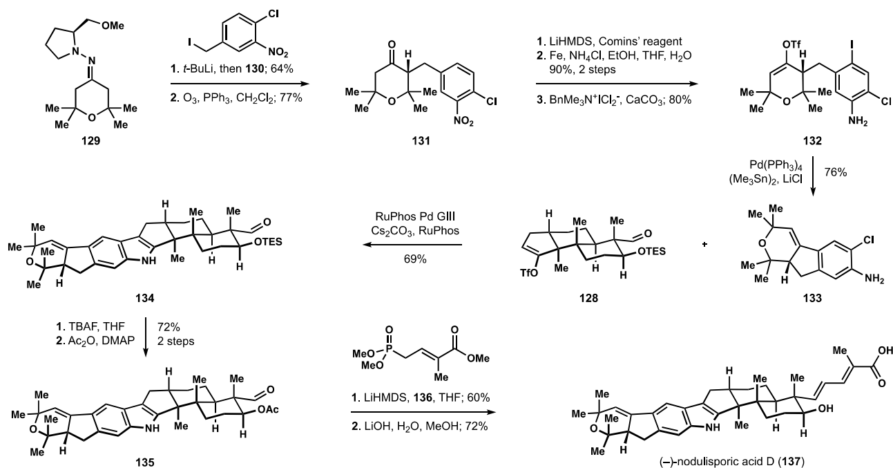
Scheme 14. The Smith synthesis of (-)-nodulisporic acid D (137).
