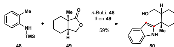
Scheme 5. The new indole synthesis developed by the Smith group.
