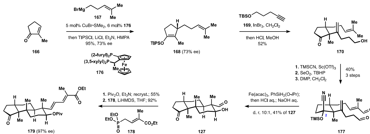
Scheme 19. Synthesis of the dienoic acid fragment by the Pronin group.
