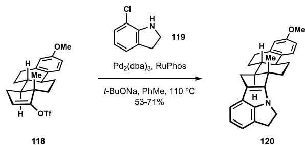
Scheme 12. Fragment coupling en route to nodulisporic acids.
