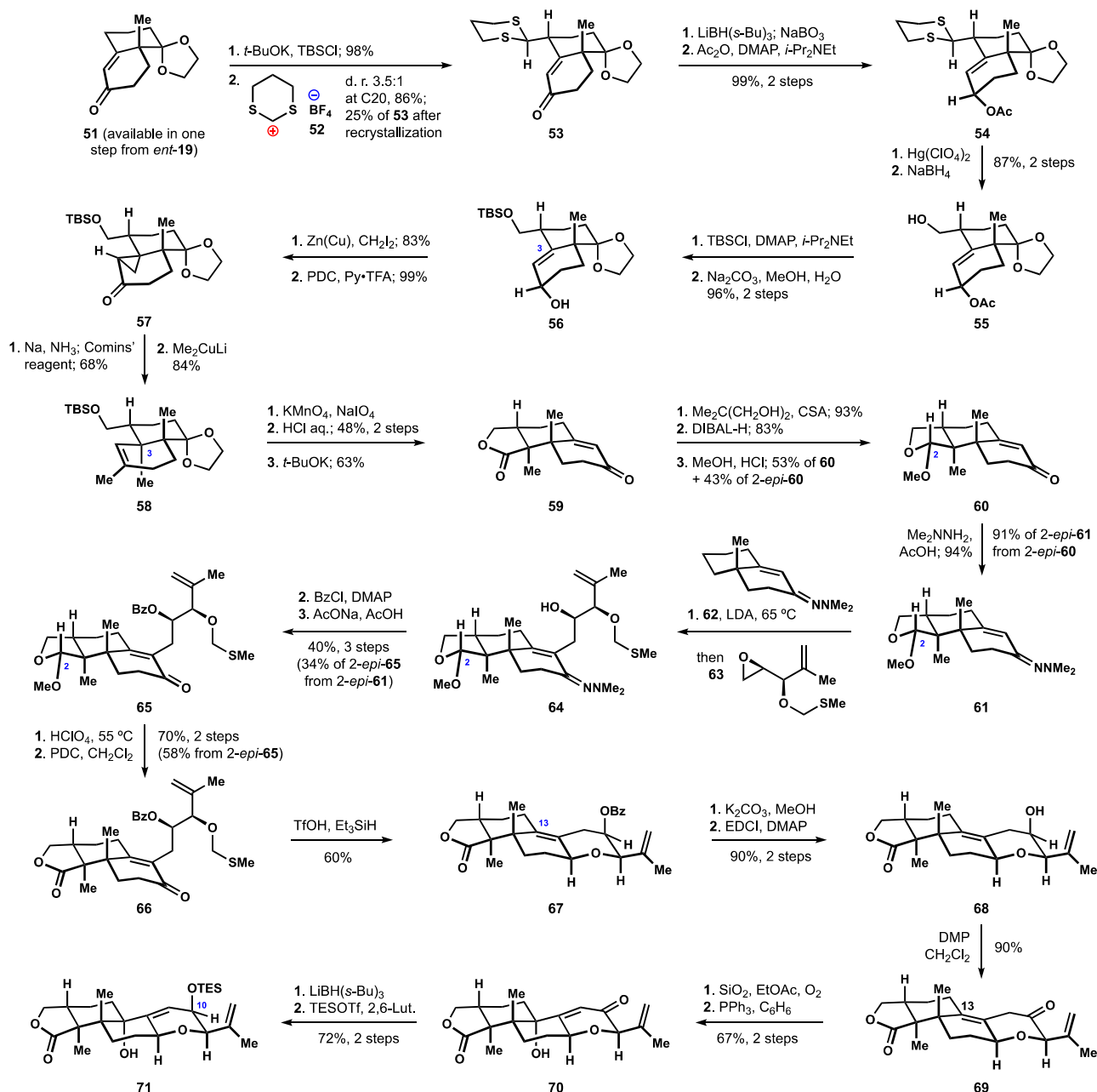
Scheme 6. Synthesis of the polycyclic terpenoid motif of penitrem A by the Smith group.
