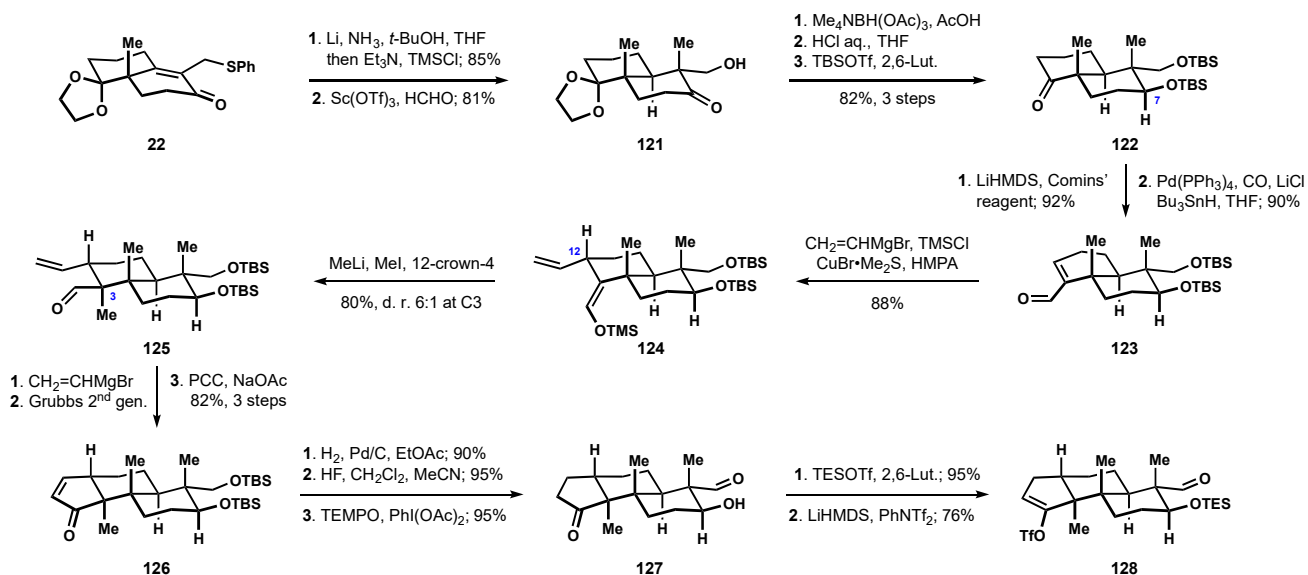
Scheme 13. Refined and abbreviated construction of the tricyclic terpenoid motif by the Smith group.
