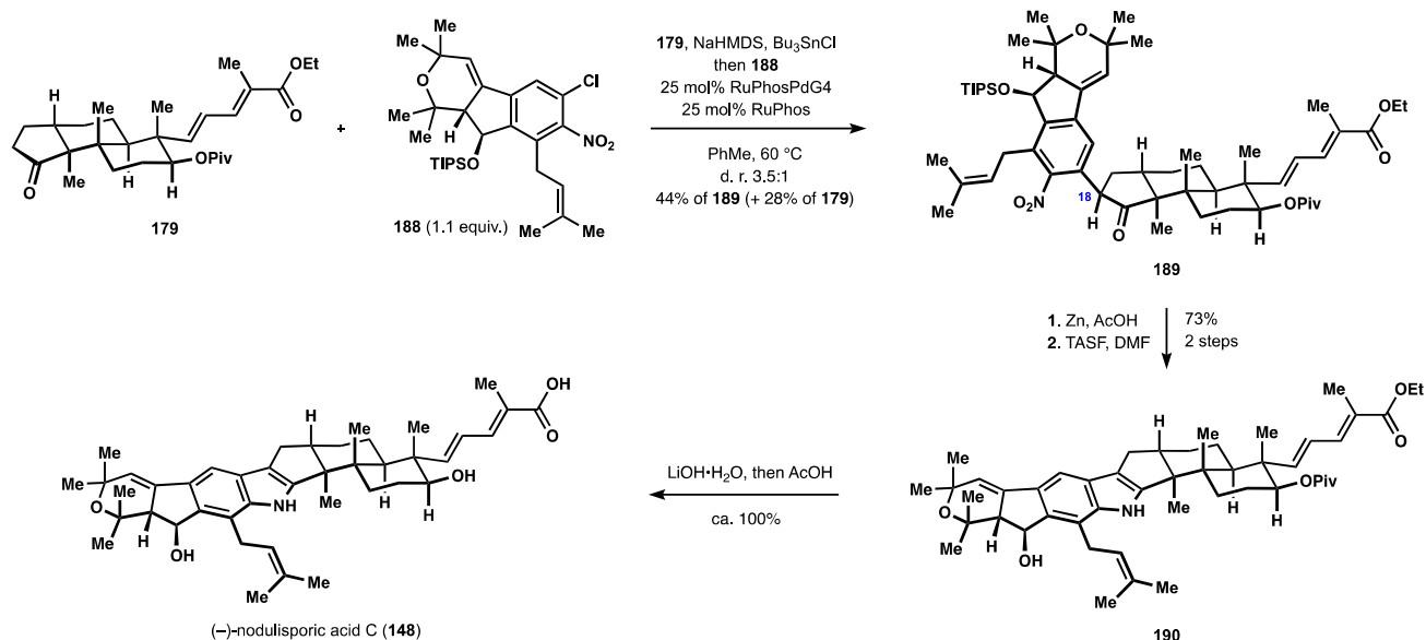
Scheme 21. The Pronin synthesis of (-)-nodulisporic acid C ( 148 ).
