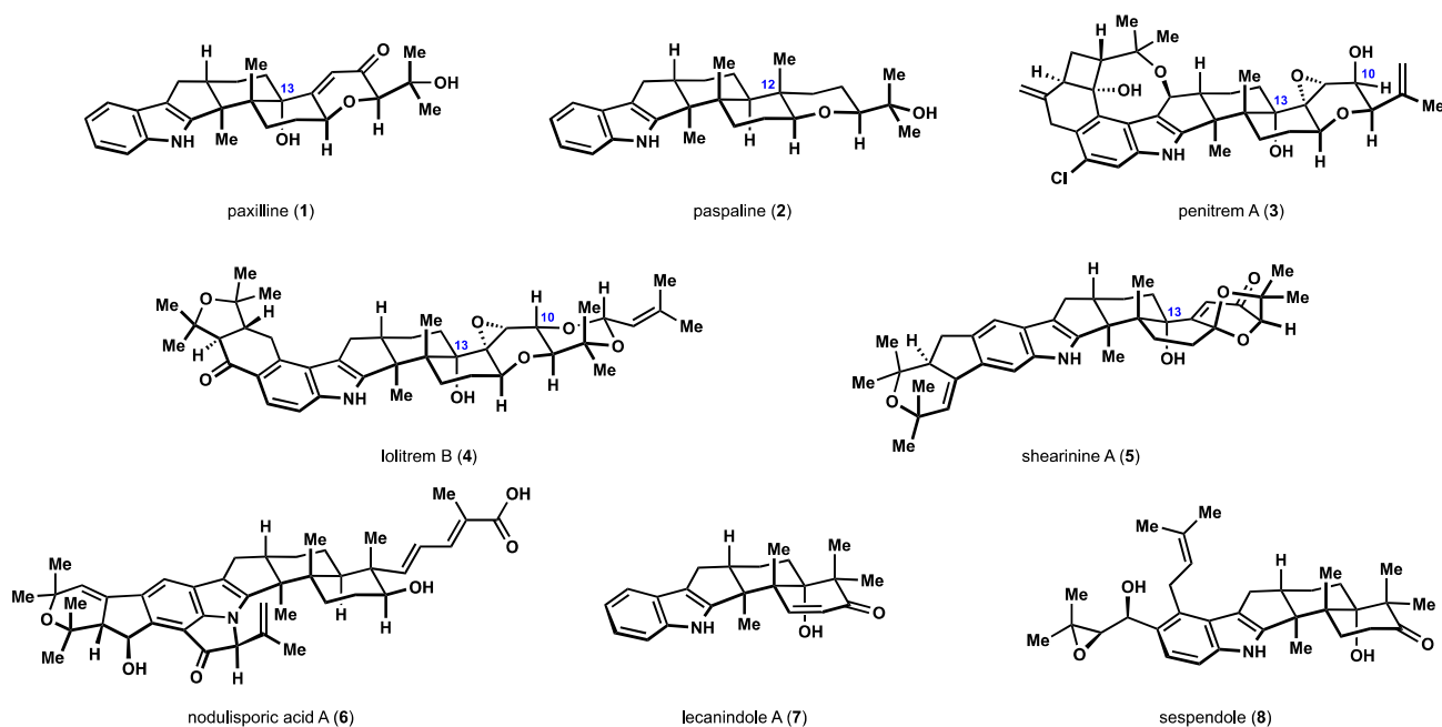
Figure 1. Representative natural products containing rearranged indoloterpenoid core.
