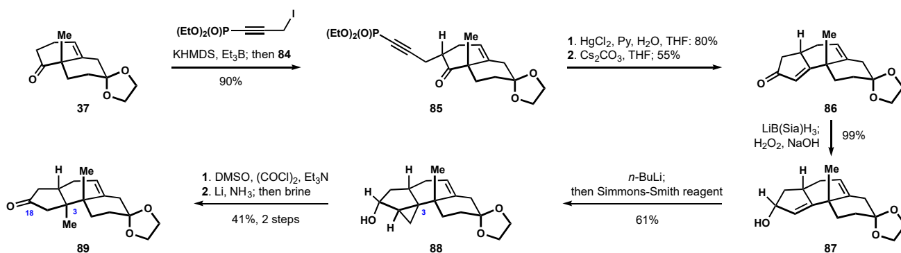
Scheme 9. The Saxton approach to the terpenoid core.
