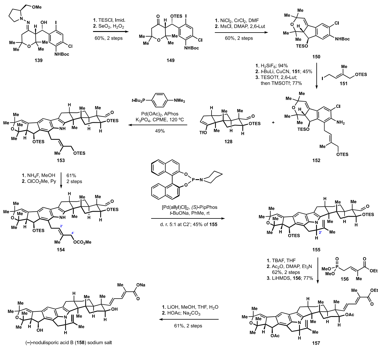
Scheme 16. The Smith synthesis of (-)-nodulisporic acid B ( 158 ).
