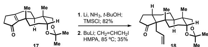
Scheme 2. Reductive allylation en route to aphidicolin.
