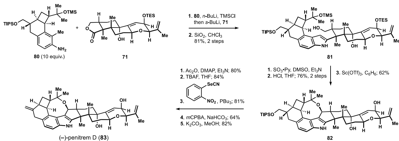
Scheme 8. The Smith synthesis of (-)-penitrem D ( 83 ).
