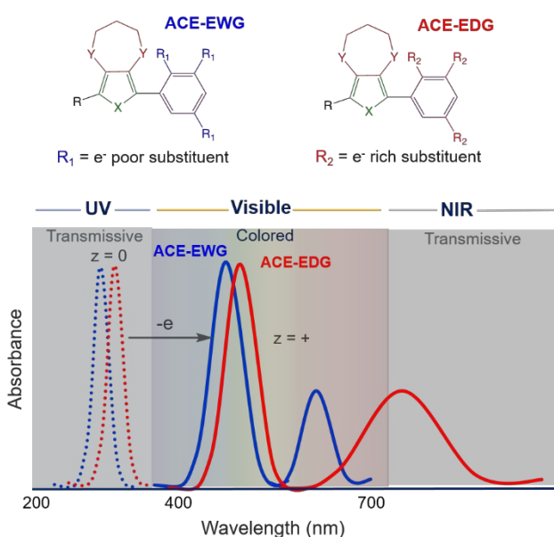
Figure 2. Illustration showing generic chemical structures of anodically coloring electrochromes, ACE-EWG and ACE-EDG and their absorbance profiles. In the neutral state, both molecules absorb in the UV (dashed lines) and in their oxidized states they absorb in the visible range, thereby appearing colored (solid lines). The position of the radical cation absorption can then be blue-shifted using electron withdrawing substituents (solid blue line) or red-shifted (solid red line) using electron donating substituents.
