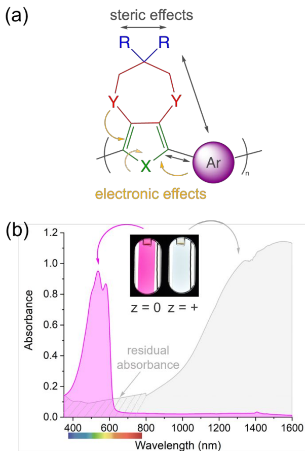
Figure 1. (a) Example of an organic, electrochromic subunit (where n can range from 1 to \infty ), (b) absorption spectra and photographs of the charge neutral (magenta) and electrochemically oxidized (grey) forms of a magenta-to-clear switching ECP film.
