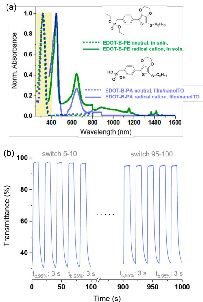
Figure 6. (a) Spectra of the neutral and radical cation states of EDOT-B-PE (dissolved in 0.5 M TBAPF 6 /dichloromethane, green traces) and EDOT-B-PA adsorbed on a nanoITO electrode and immersed in 0.5 M TBAPF 6 /dichloromethane (blue traces). Adapted with permission from Nhon, L. et al. J. Chem. Phys. , 2021, 154, 054110. Copyright 2021, AIP. (b) Transmittance at \lambda_{\text{max}} (447 nm) of EDOT-B-PA anchored onto a nanoITO switched between -0.4 and 0.7 V vs. Fc/Fc + in 0.1 M TBAPF 6 /propylene carbonate with 10 second intervals for 100 switches (only switches 5-10 and 95-100 are shown here for clarity). The nanoITO electrode was prepared via blade coating of a nanoITO dispersion onto a conventional ITO/glass slide using a speed of 10mm/s, and a blade-height of 100 \mu\text{m} . The electrode was then heat treated at 200 ^{\circ}\text{C} for 72 hours before soaking it
