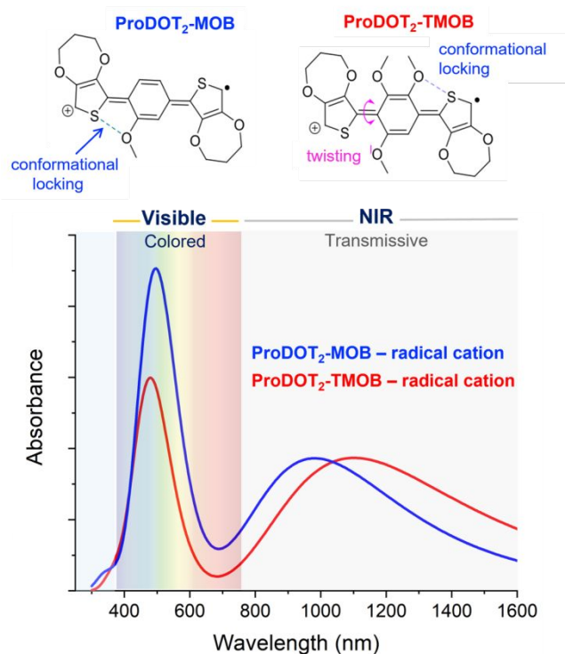
Figure 4. Structure of three-ring ACE systems, ProDOT 2 -MOB (blue) and ProDOT 2 -TMOB (red) in their radical cation states. The extended conjugation on these three-ring heteroaryl systems
