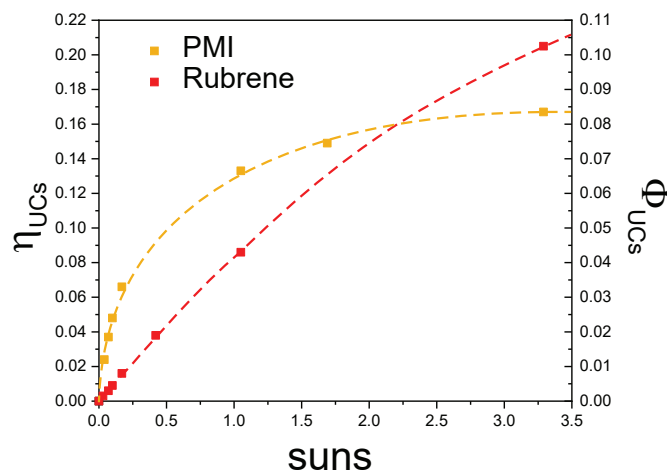
Fig. 7 (Normalized, left axis) upconversion state efficiencies for the \text{PQ}_4\text{Pd} sensitized upconvertors as a function of the bias intensity (in sun equivalence). The dashed lines are to guide the eye.
