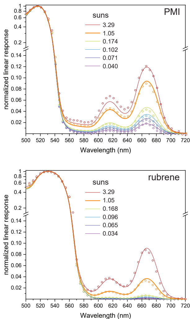
Fig. 6 Excitation-action spectra (symbols) of \text{PQ}_4\text{Pd} sensitized upconverters with PMI (top) and rubrene (bottom) annihilator. The solid lines represent fits to the experimental data using the broadband bias model, as described in the text. The fits to 1.05-sun data are plotted as thick lines.
