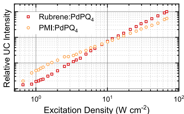
Fig. 5 Integrated steady-state upconversion intensity for PMI:PdPQ 4 and rubrene:PdPQ 4 blends as a function of excitation power, from external quantum yield measurements. Both upconverter blends were excited at 670 nm. The intensity axis has rescaled to allow for a relative comparison, as described in the text.
