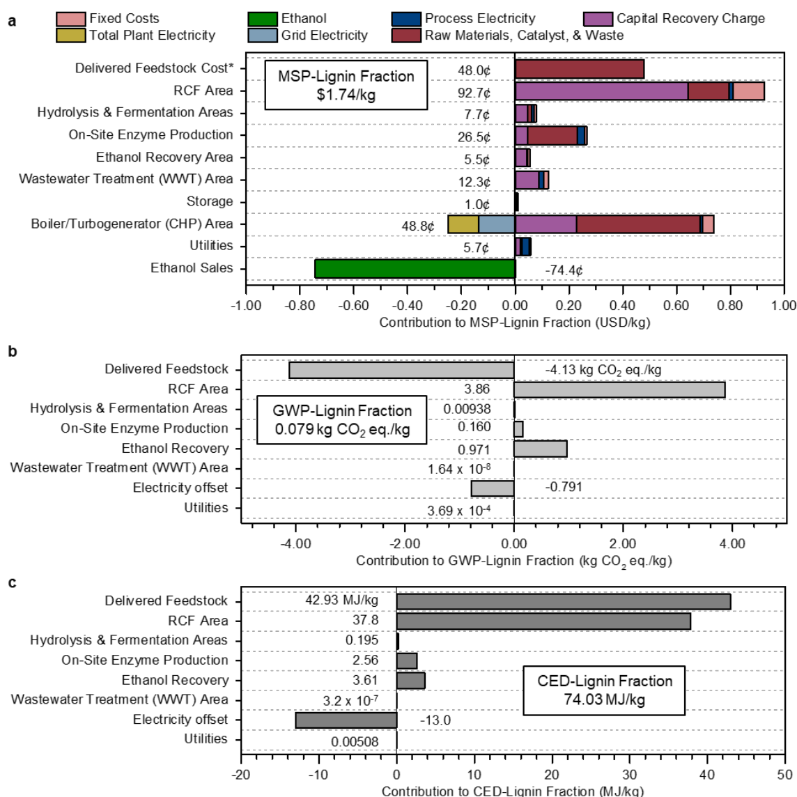
Fig. 2 Methanol case economics, GWP, and CED. (a) Contributions to the MSP of the lignin portion of RCF oil (MSP-Lignin Fraction). Fixed costs include labor and overhead. Grid electricity is excess generated electricity sold to the grid, process electricity is the electricity needs for that process area, and total plant electricity is electricity generated to offset process electricity. Raw materials include biomass feedstock and process inputs such as makeup solvent, hydrogen, glucose for enzyme production, and natural gas. Capital recovery charge accounts for capital depreciation (capital costs), annual income tax, and return on investment. The cost categories on the y-axis are organized by process area, corresponding to the block flow diagram in Fig. 1, along with input and output costs such as feedstock, enzyme production, utilities, and ethanol sales that are not encompassed in a specific area. The sum of all individual contributions is the MSP-Lignin Fraction, or MSP of the lignin portion of the RCF oil product, at $1.74/kg. *Cost of feedstock includes all upstream feedstock logistics, handling, and pre-processing steps up to the reactor. (b) Breakdown of contributions to GWP-Lignin Fraction. The results shown are normalized to the production of 1 kg lignin fraction and allocated according to mass. Economic allocation results are given in Table S5. Delivered feedstock includes CO 2 uptake by growing poplar. The boiler/turbogenerator (CHP) area is not shown in (b) or (c) because impacts for that area have been divided between process areas with steam demand according to the fraction of total steam used by each area: RCF area (89.6%), hydrolysis & fermentation areas (10.2%), and on-site enzyme production (0.2%). Because GHG emissions are attributed to different process sections, the CHP area is not explicitly included in Figures B and C. Electricity offset is emissions credits assigned to the biorefinery from displacement of grid electricity. The total GWP, including the electricity offset and CO 2 uptake by growing poplar, is 0.079 kg CO 2 -eq/kg lignin fraction under mass allocation and 0.131 kg CO 2 -eq/kg lignin fraction under economic allocation. (c) Breakdown of contributions to CED-Lignin Fraction. Results shown are normalized to 1 kg lignin fraction and allocated according to mass. Economic allocation results are given in Table S6. As was done for GWP, CED for the CHP area was divided between steam-using process areas, and the CHP area is not shown separately in the figure. Electricity offset is the energy credit from displacement of grid electricity. The total CED is 74.03 MJ/kg lignin fraction under mass allocation and 122.04 MJ/kg lignin fraction economic allocation. All data shown in Fig. 2 are included in numerical form in Table S6 for Fig. 2a and Table S7 for Fig. 2b-c.
