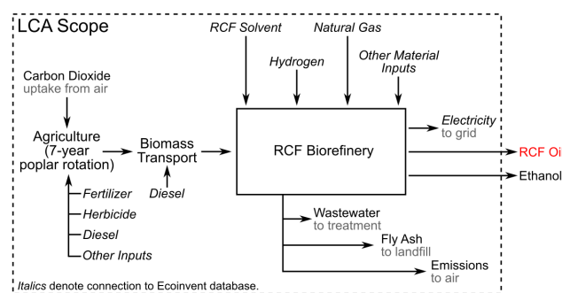
Fig. 9. System boundary diagram for the LCA, with connections to the background LCI database indicated with italics.
