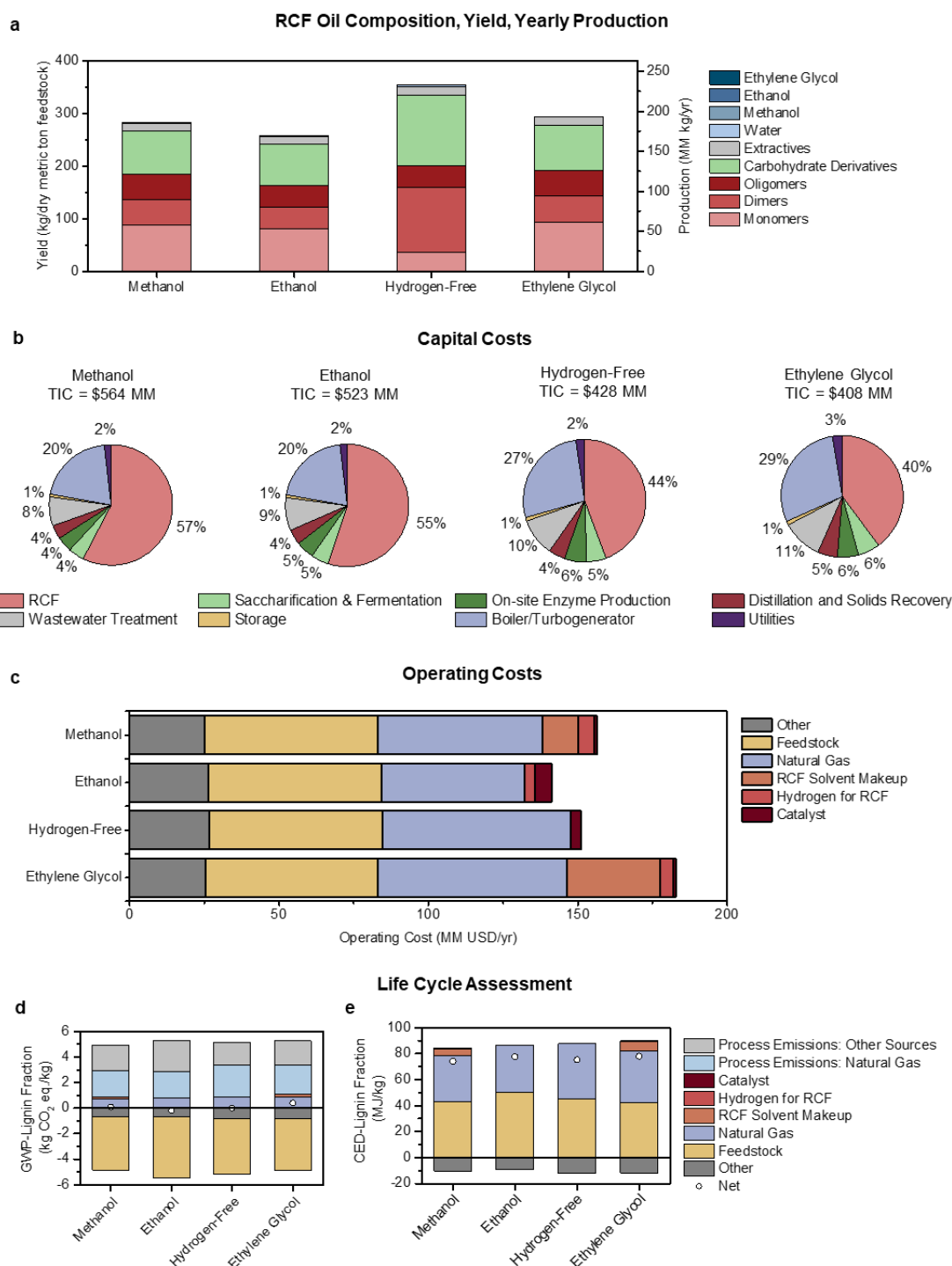
Fig. 5. Economic and life cycle comparison of RCF process configurations. Methanol utilizes methanol solvent and hydrogen gas, Ethanol uses solvent generated in the biorefinery, Hydrogen-Free generates hydrogen in situ from hemicellulose, and Ethylene Glycol uses hydrogen gas and ethylene glycol solvent. (a) A summary of RCF oil composition, yield, and productivity. The composition was based on literature values for similar processes at the bench-scale. Yield and productivity values were outputs of the process model at a 2000 dry metric tons feedstock/day throughput. (b) Capital cost breakdown by area for each process configuration, with the total installed capital cost (TIC) included above the pie charts. (c) Yearly operating costs for each process configuration. "Other" costs are associated with carbohydrate conversion to 7ethanol downstream of the RCF area. (d) GWP-Lignin Fraction for each configuration shows categories that contribute to carbon emission and carbon uptake, with net GWP-Lignin Fraction indicated with a white circle. (e) CED-Lignin Fraction for each configuration shows categories that contribute to energy consumption and energy generation (in the form of excess electricity to the grid), with net CED-Lignin Fraction indicated with a black circle. See Fig. 1 and Fig. S3-S5 for diagrams of each configuration, Table 2 for a complete list of assumptions for each case, and ESI Tables S17-S21 for full tabulated data shown in this figure. GWP-Lignin Fraction and CED-Lignin Fraction under economic allocation for each configuration are given in Table S22.
