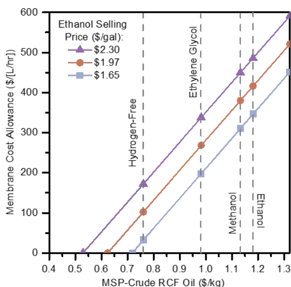
Fig. 6: Membrane cost allowance. Sensitivity scan of maximum membrane capital cost allowance per throughput volume in order to achieve a given RCF oil MSP at the fuel selling price target. See Table S23 for tabulated data shown in this figure.
