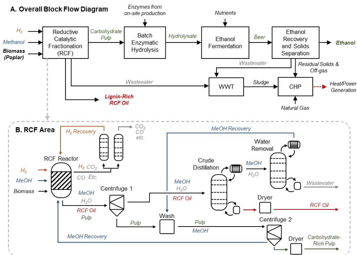
Fig. 1. RCF biorefinery design. (a) Block flow diagram of an RCF-based cellulosic ethanol biorefinery. This process follows a configuration similar to that described by Humbird et al. , with the dilute-acid pretreatment area replaced with RCF. The RCF area produces a lignin-rich RCF oil as a co-product and a carbohydrate-rich pulp. Carbohydrate pulp, the residual biomass solids after the lignin is removed during RCF, is isolated and saccharified to C 5 and C 6 sugars via enzymatic hydrolysis, fermented to ethanol, and recovered to produce fuel-grade ethanol. WWT is the wastewater treatment area. CHP is the combined heat and power area where a combination of natural gas, sludge from WWT, and residual solids from ethanol production are burned to generate steam for process heat and electricity. Excess electricity is sold to the grid as a co-product. (b) The process diagram highlighting major unit operations in the RCF area of the biorefinery for the methanol case. The solvent pump-around RCF reactor design is shown in Fig. S2. The gaseous products are sent to a PSA unit to recover H 2 to be recycled to the reactor, and the liquid and solid products are separated via centrifugation to isolate dilute RCF oil, which is concentrated in a crude distillation column, and water is removed from methanol in the water removal distillation column. After washing with methanol to recover additional lignin oil, the carbohydrate-rich pulp is isolated via a second centrifuge and the methanol rinse is recycled back to the RCF reactor. Major heating and cooling duties were heat integrated to reduce overall energy demand. A process flow diagram with labeled streams and a corresponding table of stream compositions is included in Fig. S1 and Table S2.
