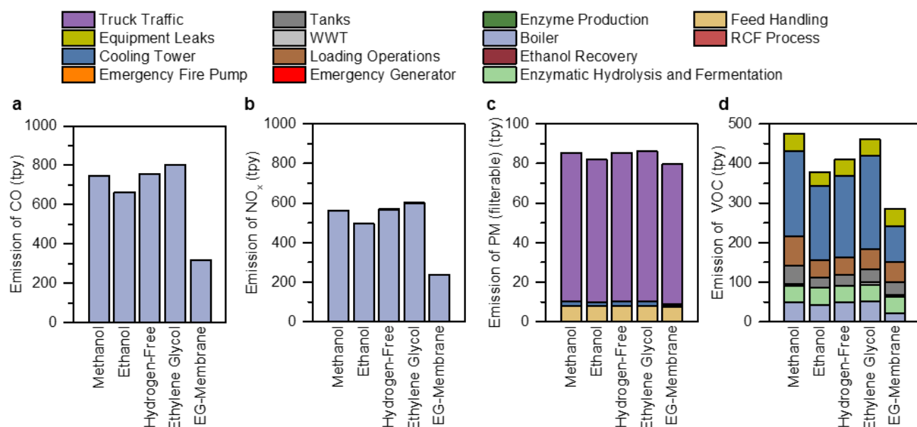
Fig. 7: Non-GHG Air Pollutant Emissions. Overview of (a) CO, (b) NO x , (c) PM, and (d) VOCs for each of the RCF process design cases and the hypothetical membrane separation case, broken down by the source of the emission. The assumptions and methods used for this analysis are summarized in materials and methods . The raw tabulated data is included in Table S24-S28 . Bar charts for other air pollutants analyzed in this study (PM10, PM2.5, SO 2 , and hazardous air pollutants) are included in Fig. S7 .
