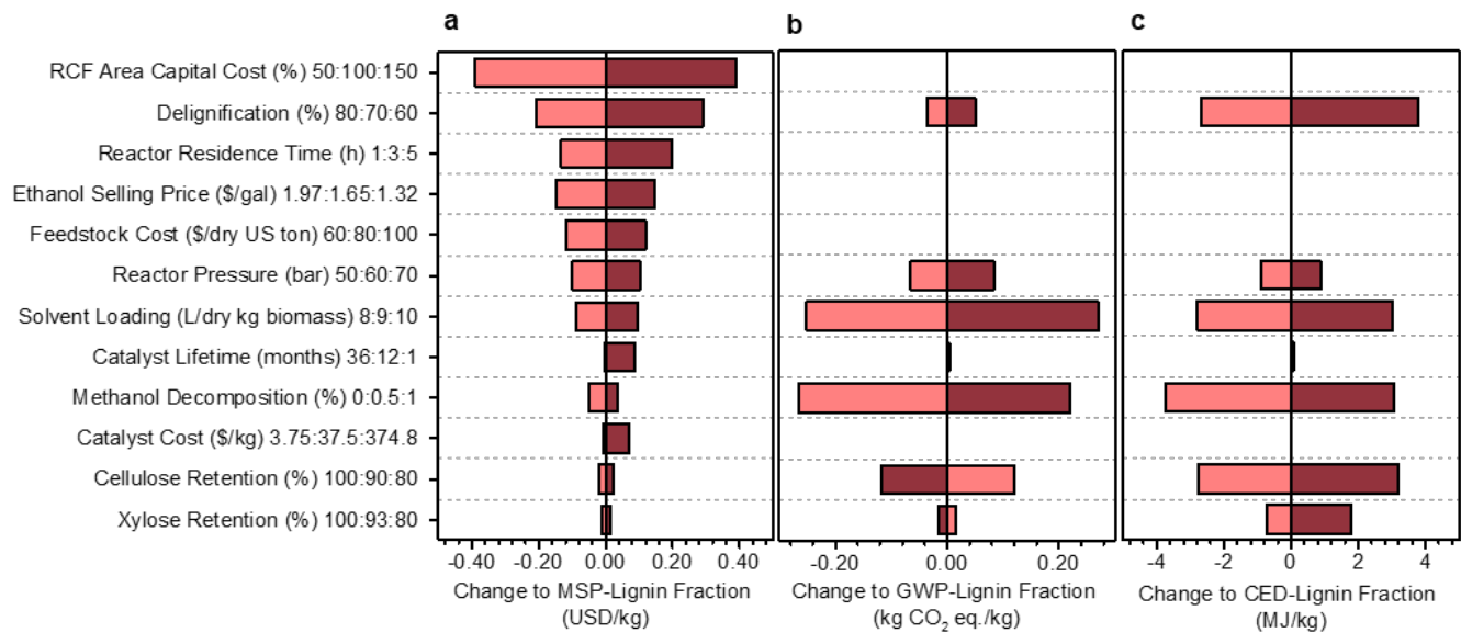
Fig. 3 Sensitivity analysis of the methanol case. Results of single point sensitivity analyses for change to the (a) MSP-Lignin fraction, or MSP of the lignin constituents in RCF oil (base normalized price = $1.74/kg), (b) GWP-Lignin Fraction under mass allocation, and (c) CED-Lignin Fraction under mass allocation. For each sensitivity case, the key variable was modified to either its minima or maxima while holding all other variables constant to the methanol case. The minima and maxima values used in this analysis are shown in the vertical axis labels as Low Cost (light red):Base:High Cost (dark red). Low Cost and High Cost indicate variable modifications which led to respective net reductions or increases in the MSP-Lignin Oil. Reasonable minima and maxima were chosen to understand quantitative impacts based on expected uncertainty, prospective process modifications, or potential limits of each variable, and were then used to evaluate the change in MSP-Lignin Fraction, GWP-Lignin Fraction, and CED-Lignin Fraction. Full rationale for selection of minima and maxima is given in Table S8 . All data shown in Fig. 3 is included in numerical form in Table S9 . Sensitivity results for change to MSP-Crude RCF Oil are given in Table S10 . Sensitivity results for GWP and CED under economic allocation are given in Table S11 .
