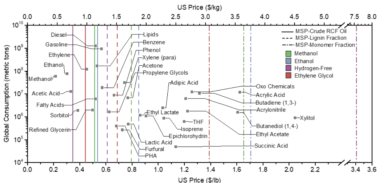
Fig. 8. Minimum RCF oil selling prices with the US price and global consumption of various chemicals for reference. The US Price and Global Consumption data were sourced from a 2016 report by Biddy et al. and are 3-5 year averages. 76 Tabulated data are summarized in Table S34 .
