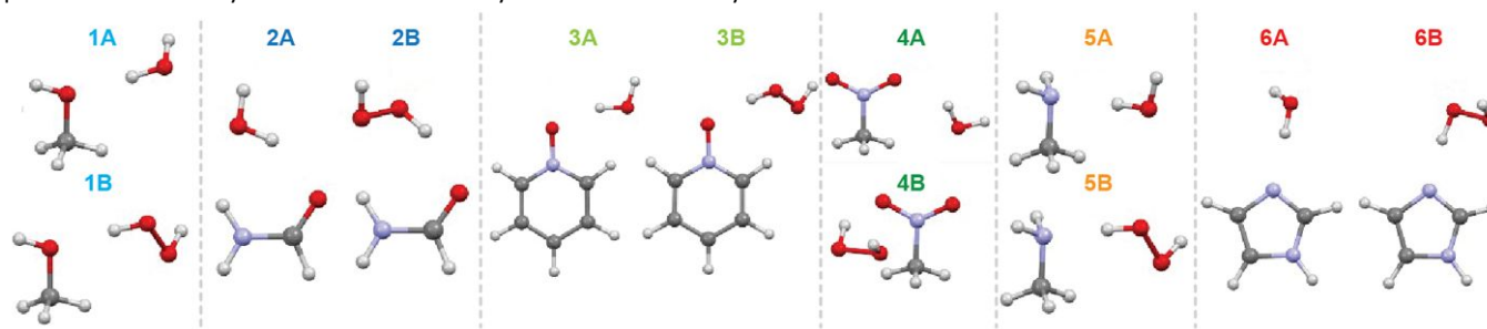
Figure 2. PES global minimum geometries for heterodimers formed between water (A) or hydrogen peroxide (B) and the model small molecules methanol (1), formamide (2), pyridine oxide (3), nitromethane (4), methylamine (5), and imidazole (6).
