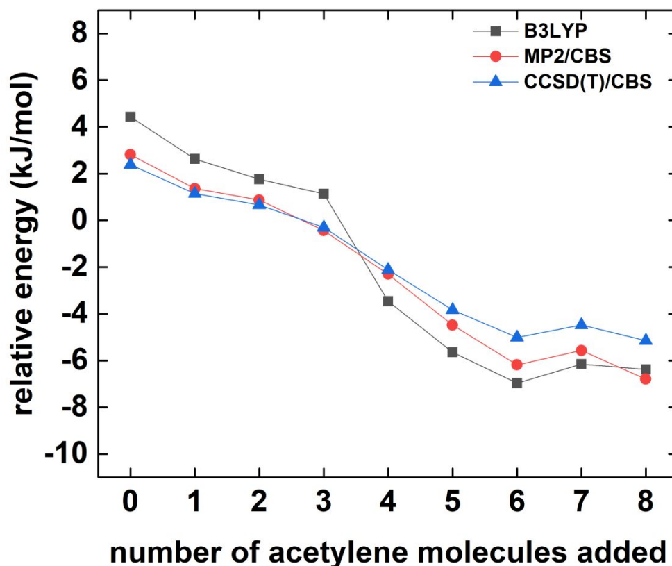
Figure 9. Relative energies of the first transition state and/or van der Waals complex on the T_1 surface with increased number of acetylenes surrounding the benzene trimer reaction center. Energies are referenced to the initial complex as a function of the number of acetylene molecules ( n ) in the C_6H_6/(C_2H_2)_n cluster. The energy of the initial complex is defined as zero.
