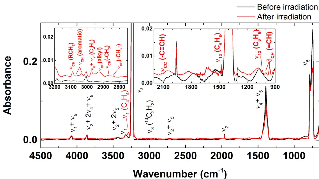
Figure 3. Infrared spectra of acetylene ices at 5 K. Spectra were taken before (black line) and after (red line) irradiation with 222 nm photons at a dose of 8.4 \pm 1.2 eV molecule -1 . The insets show details of the new IR bands after irradiation.
