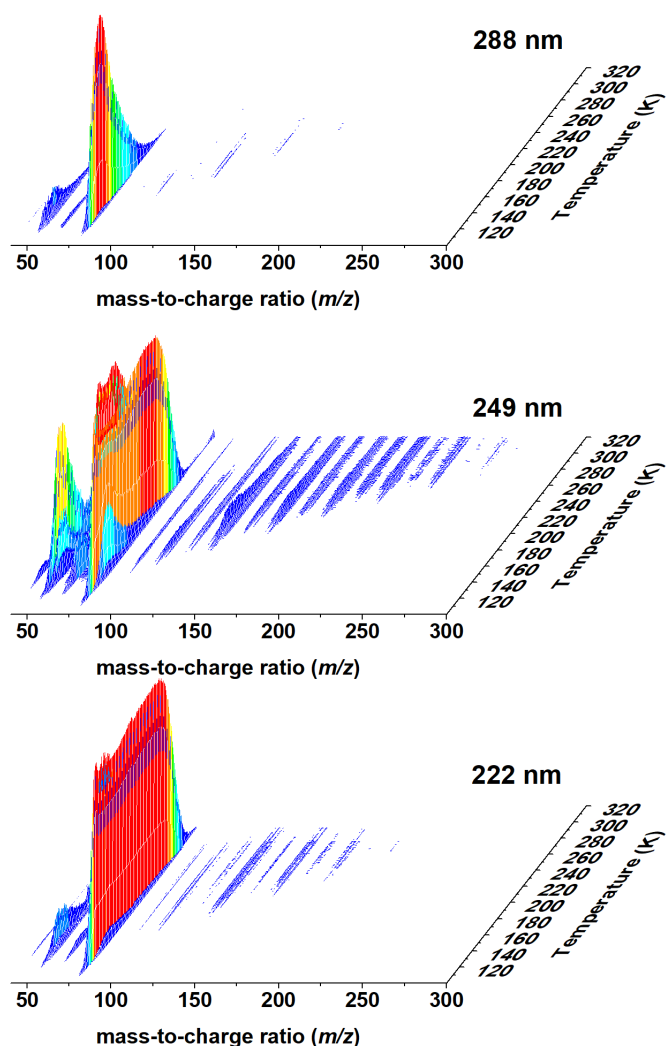
Figure 4. Temperature-dependent mass spectra. Spectra were recorded at 259.003 nm of acetylene ices irradiated with 288 nm (top), 249 nm (middle), and 222 nm (bottom) photons. absorption followed by a second photon, which then ionizes the molecule. As the S_n \leftarrow S_0 transitions of substituted benzenes and more complex PAHs can be accessed between 266 nm
