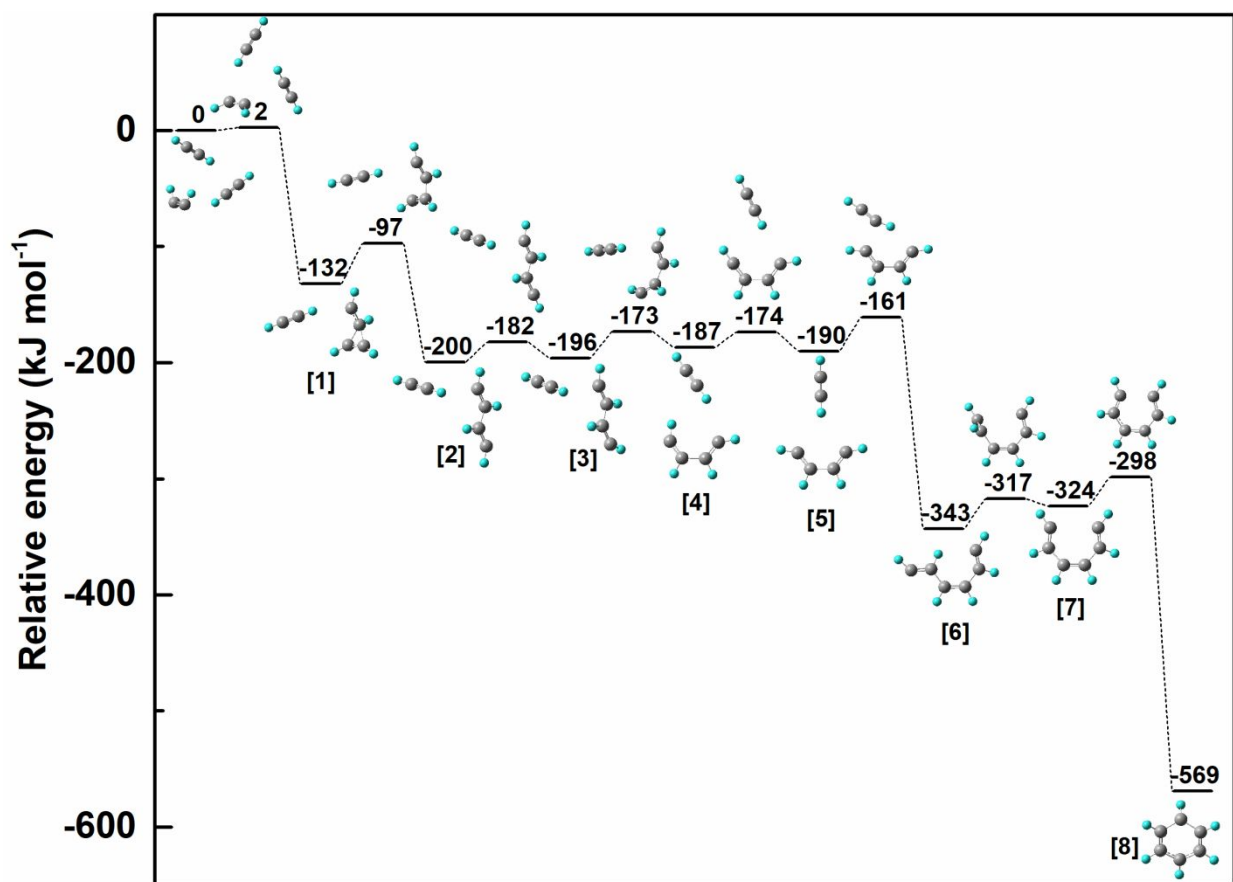
Figure 6. The T_1 C_6H_6 potential energy surface involved in the formation of triplet benzene via acetylene reactions. Energies are given in \text{kJ mol}^{-1} . Geometries were optimized at the B3LYP/6-311G** level. Single-point electronic energies were calculated at the CCSD(T)/CBS level. Zero-point energies were corrected using B3LYP/6-311G**, and the solvation energy was calculated by the CPCM model with B3LYP/6-311G** (Methods Section).
