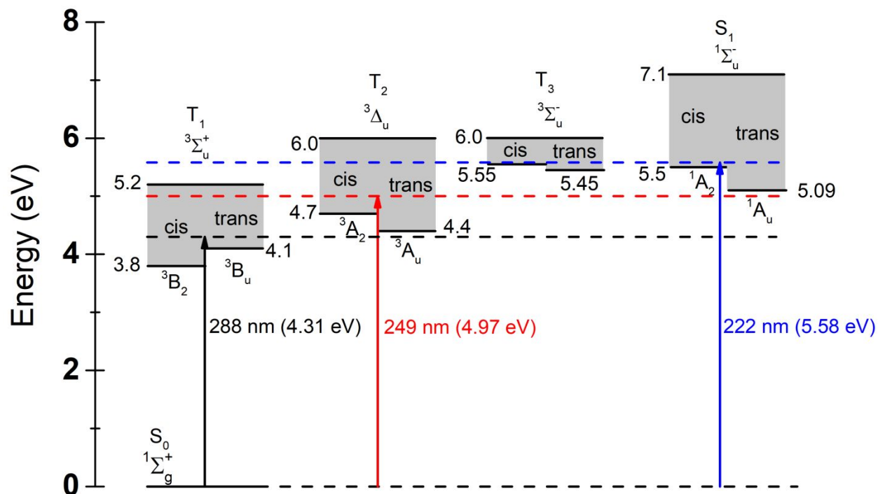
Figure 1. Energy level diagram of the four lowest energy excited states. The upper energy limit of each state corresponds to the linear symmetry (vertical excitation), the lower lines to the adiabatic transitions to the cis and trans geometries. Arrows and dashed lines correspond to the excitation energies used in this study.
