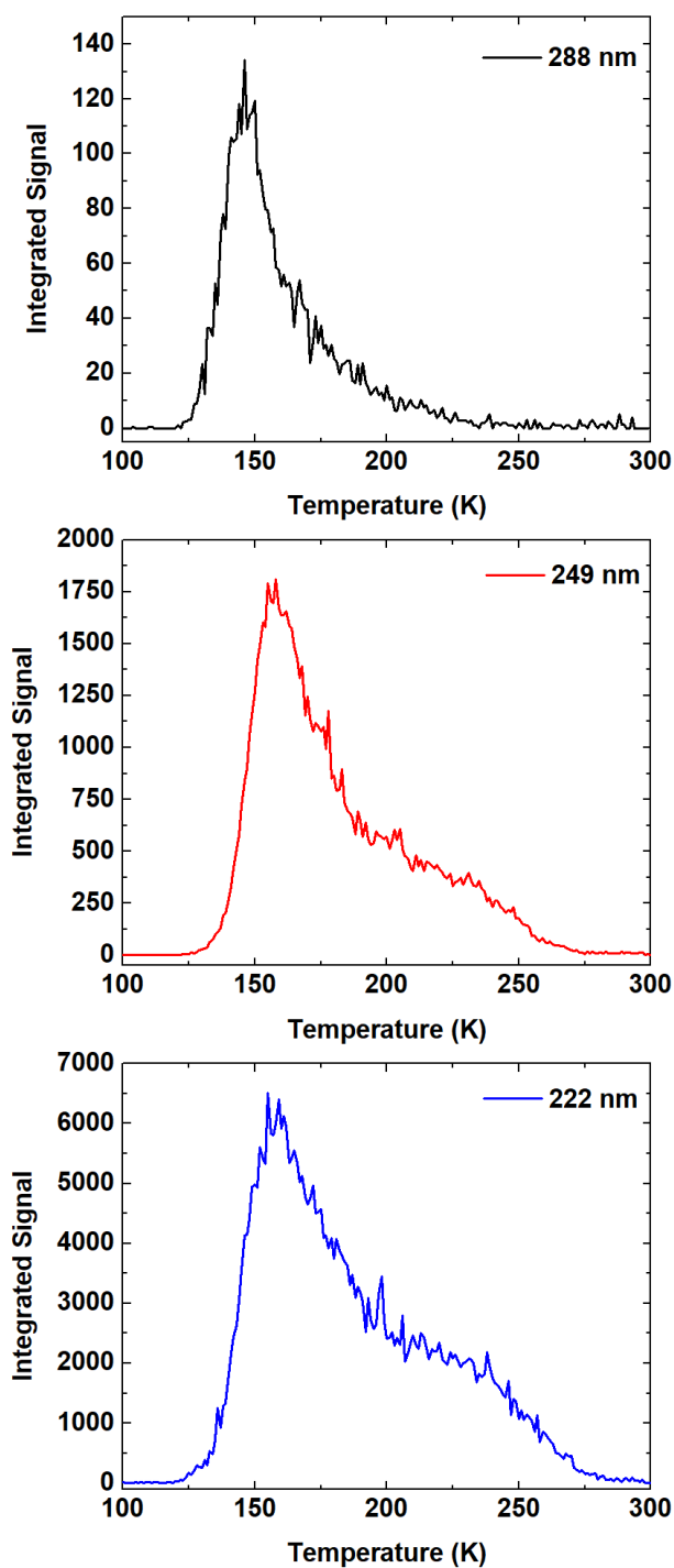
Figure 5. TPD profiles of m/z = 79 (Benzene- 13 C 1 ). Spectra were recorded at 259.003 nm for acetylene ices irradiated with 288 nm (top), 249 nm (middle), and 222 nm (bottom) photons. The measurement of the ice photolyzed at 222 nm was recorded at a lower MCP voltage and lower ice thickness to prevent saturation and has been scaled accordingly.
