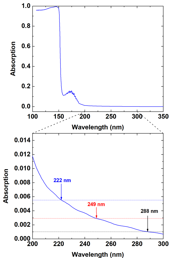
Figure 2. Absorption spectrum of solid acetylene from 107 to 350 nm. The bottom panel shows an enlarged view of the wavelength range from 200 to 300 nm. Arrows indicate the wavelengths used in this study.
