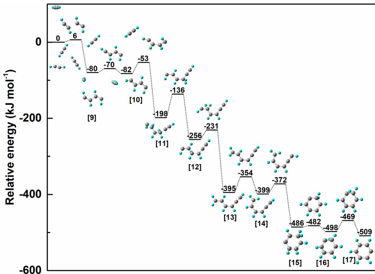
Figure 7. The T_2 C_6H_6 potential energy surface involved in the formation of triplet benzene via acetylene reactions. Energies are given in \text{kJ mol}^{-1} . Geometries were optimized at the TD-B3LYP/6-311G** level. Single-point electronic energies were calculated at the CASPT2/aug-cc-pVTZ level. Zero point energies were corrected using TD-B3LYP/6-311G**, and the solvation energy was calculated by the CPCM model with TD-B3LYP/6-311G** (Methods Section).
