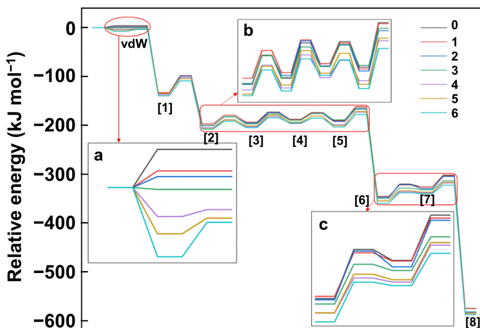
Figure 8. Potential energy surfaces of the reaction for the formation of triplet benzene on the T_1 surface with increased number of acetylenes surrounding the benzene trimer reaction center. Relative electronic energies were calculated at the CCSD(T)/CBS level (Methods Section). The legend indicates the number of additional acetylene molecules surrounding the reaction center and the transition from an entrance barrier to a submerged barrier as the number of acetylene molecules in the solvation shell increases.
