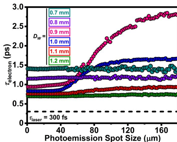
Figure 4. Single-electron packet duration ( \tau_{\text{electron}} , fwhm) as a function of photoemission spot size for D_W ranging 0.7-1.2 mm. The \text{LaB}_6 D_{\text{tip}} was 180 \mu\text{m} . The horizontal black dashed line ( \tau_{\text{laser}} ) represents the selected probe laser-pulse duration of 300 fs (fwhm). The h\nu = 4.81 -eV distribution in Figure 1d was used as the E_0 .
