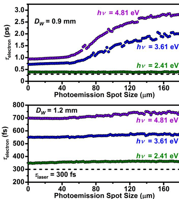
Figure 5. Single-electron packet duration ( \tau_{\text{electron}} , fwhm) as a function of photoemission spot size for discrete laser photon energies ( h\nu = 2.41, 3.61, and 4.81 eV) for D_W = 0.9 mm (top) and 1.2 mm (bottom). The \text{LaB}_6 D_{\text{tip}} was 180 \mu\text{m} . The horizontal black dashed line ( \tau_{\text{laser}} ) in each panel represents the selected probe laser-pulse duration of 300 fs (fwhm). The E_0 distributions shown in Figure 1d were used for each corresponding photon energy.
