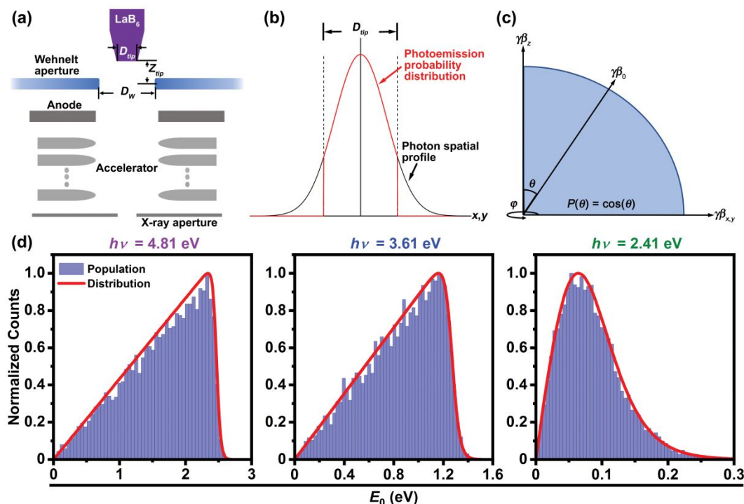
Figure 1. Elements of the simulations. (a) Simplified schematic of the FEI Tecnai Femto electron gun and accelerator with key components and dimensions labeled. D_{tip} is the diameter of the LaB 6 emitting surface, Z_{tip} is the distance from the LaB 6 surface to the plane of the Wehnelt aperture (here, fixed at 0.35 mm), and D_w is the diameter of the Wehnelt aperture. (b) Spatial photoelectron emission probability (red curve) from the LaB 6 emitting surface for a Gaussian laser-spot shape (black curve). The probability is set to zero for x,y > D_{tip} . (c) Photoelectron emission probability ( P ) as a function of emission angle ( \theta ) relative to the center of the illuminated LaB 6 surface. The full probability distribution subtended by the LaB 6 emitting surface parallel to the x,y plane is generated by sweeping azimuthally over \varphi to establish cylindrical symmetry. \gamma and \beta are the Lorentz factor and the normalized relativistic velocity,
