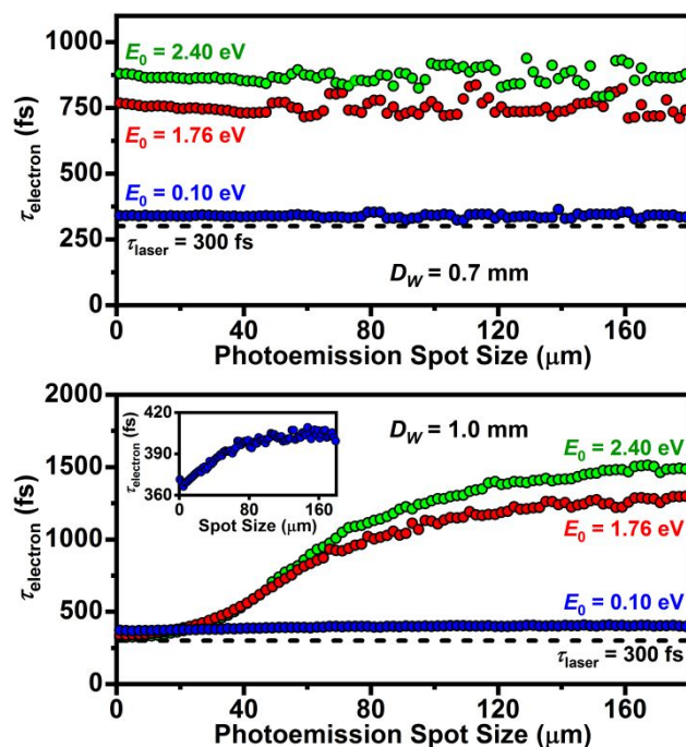
Figure 2. Single-electron-packet duration ( \tau_{\text{electron}} ; fwhm) as a function of LaB 6 photoemission spot size for D_W = 0.7 mm (top) and D_W = 1.0 mm (bottom). Note that three discrete initial photoelectron kinetic energies ( E_0 = 0.10 , 1.76, and 2.40 eV) were compared ( i.e. , here, the full distributions shown in Figure 1d were not yet used in order to first focus on the effect of photoemission spot size and D_W ). The horizontal black dashed line in each panel ( \tau_{\text{laser}} ) represents the selected probe laser-pulse duration of 300 fs (fwhm) typical of the current system at Minnesota. The inset (bottom panel) is the 0.10-eV plot for D_W = 1.0 mm with the y -axis rescaled to visualize the subtle response of \tau_{\text{electron}} .
