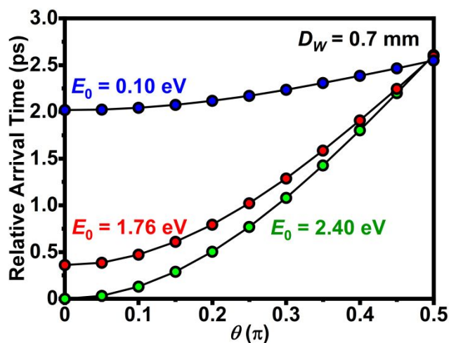
Figure 3. Relative photoelectron arrival time at a fixed position after the final electron-gun element as a function of initial photoemission angle from the LaB 6 surface ( \theta ) for D_W = 0.7 mm and E_0 = 0.10 , 1.76, and 2.40 eV. The photoemission spot size was fixed at 5- \mu m diameter for all data, and all photoelectrons had the same initial momentum. All arrival times are relative to \theta
