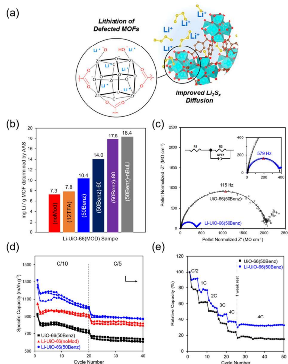
Figure 5. a) Scheme of lithiated defect sites in Zr-MOF, b) Li incorporation measured by AAS for Li-UiO-66 series at various synthetic conditions, c) Nyquist plots of UiO-66(50Benz) (black diamonds) and Li-UiO-66(50Benz) (blue circles), d) discharge capacity as a function of cycle number for lithiated and non-lithiated MOF coin cells, and e) rate capabilities for UiO-66(50Benz) (black square) and Li-UiO-66(50Benz) (blue circle). Adapted with permission from Ref. 40. Copyright 2019 American Chemical Society.
