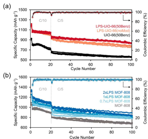
Figure 4. Cycling performance for coin cells containing a) UiO-66 and b) MOF-808 series, showing improvements in the maximum capacity and capacity retention upon LPS incorporation. Adapted with permission from Ref. 38. Copyright 2019 American Chemical Society.
