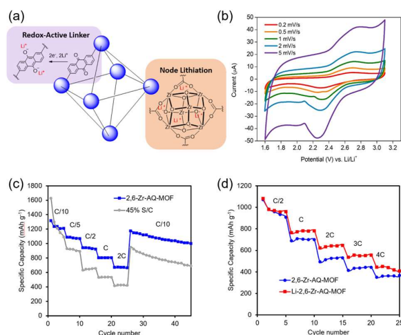
Figure 6. a) Scheme showing incorporation of AQ linkers in 2,6-Zr-AQ-MOF, b) CV of 2,6-Zr-AQ-MOF at scan rates from 0.2 to 5 \text{mV s}^{-1} , c) rate capabilities of 2,6-Zr-AQ-MOF and 45% S/C cells varied from C/10 to 2C, and d) rate capabilities of 2,6-Zr-AQ-MOF and Li-2,6-Zr-AQ-MOF cells varied from C/2 to 4C. Adapted from Ref. 42, Copyright 2019, with permission from Elsevier.
