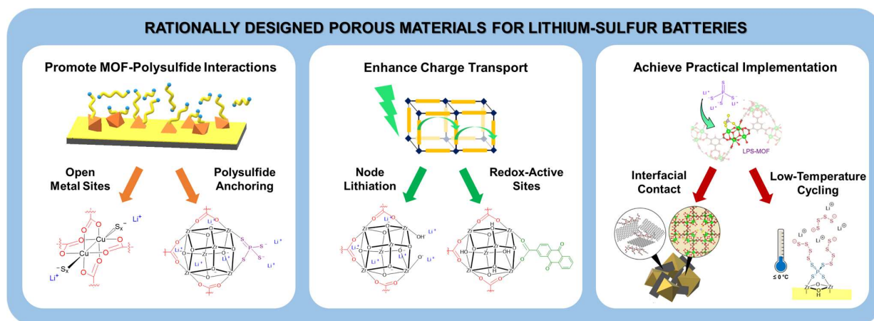
Scheme 1. Synthetic and Implementation Strategies employed for enhancing Li-S battery cycling performance.
