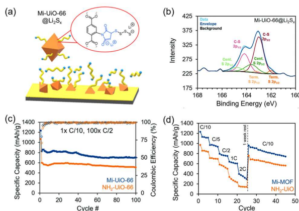
Figure 2. a) Depiction of Mi-UiO-66 upon the introduction of lithium polysulfides, b) XPS spectra of the S 2p region of Mi-UiO-66@Li 2 S x , c) specific capacity cycled at C/10 for 1 cycle and C/2 for 100 cycles, and d) rate capability of Mi-UiO-66 (blue) and NH 2 -UiO-66 (orange) cells. Reproduced from Ref. 35 with permission from the Royal Society of Chemistry.
