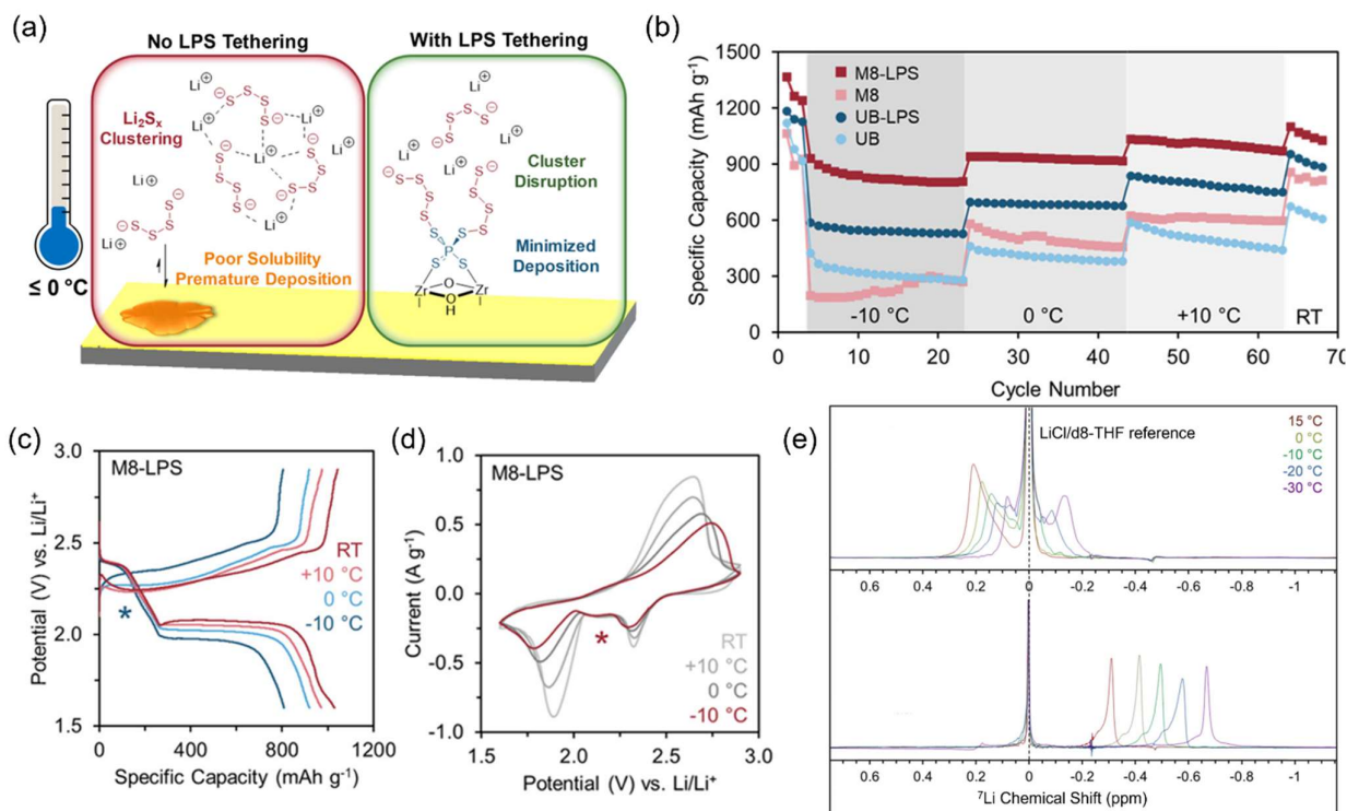
Figure 9. a) Scheme of chemical tethering via lithium thiophosphate improves electrochemical accessibility at low temperature, b) discharge capacity of cells at various temperatures at C/10, c) galvanostatic cycling curves of MOF-808-LPS at the final cycle for each temperature at C/10, d) CV for MOF-808-LPS at each temperature, and e) variable-temperature ^7\text{Li} NMR of 0.1 M \text{Li}_2\text{S}_4 (top) and 0.033 M \text{P}_2\text{S}_5 + 0.1 M \text{Li}_2\text{S}_4 (bottom) from 15 to -30^\circ\text{C} . Chemical shifts are calibrated to the \text{LiCl}/d_8\text{-THF} reference peak (dotted line). Adapted with permission from Ref. 48. Copyright 2021 American Chemical Society.
