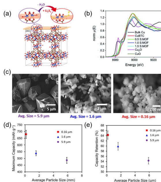
Figure 1. a) Solid-state structure of CuBTC and proposed polysulfide binding at surface Cu sites, b) XANES profiles, c) scanning electron micrographs showing CuBTC of different particle sizes, d) average maximum capacity and e) capacity retention (after 20 cycles) of CuBTC@S cells as a function of particle size. Reproduced from Ref. 33 with permission from the Royal Society of Chemistry.
