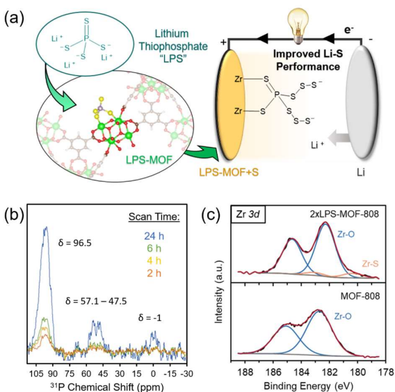
Figure 3. a) Illustration of thiophosphate-functionalized Zr-MOFs, b) solid-state 31 P NMR spectra of LPS-UiO-66(50Benz), and c) XPS of the Zr 3d region in MOF-808 and in 2xLPS-MOF-808. Adapted with permission from Ref. 38. Copyright 2019 American Chemical Society.
