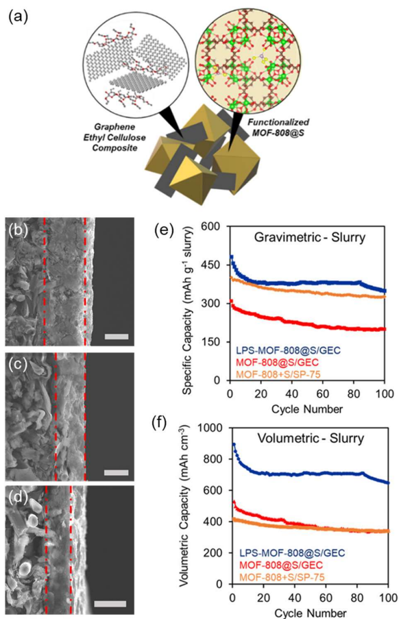
Figure 8. a) Depiction of MOF@S/GEC, cross-sectional profiles of carbon paper electrodes coated with b) MOF-808+S/SP-75, c) MOF-808@S/GEC, and d) LPS-MOF-808@S/GEC slurries (scale bar is 20 \mu\text{m} ), and e) gravimetric and f) volumetric capacity based on the slurry, highlighting the denser form factor of the MOF-808@S/GEC compared to MOF-808+S/SP-75 composite electrodes. Adapted with permission from Ref. 45. Copyright 2020 American Chemical Society.
