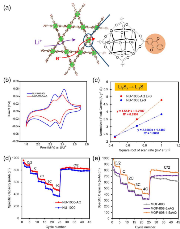
Figure 7. a) Illustration of charge transport in Zr-MOF-AQ, b) CV of NU-1000-AQ and MOF-808-3xAQ, c) sulfur mass-normalized peak current as a function of the square root of scan rate, and rate capabilities for d) NU-1000 series and e) MOF-808 series varied from C/2 to 4C. Adapted with permission from Ref. 44. Copyright 2020 American Chemical Society.
