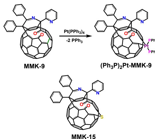
Scheme 1. Formation of (\text{Ph}_3\text{P})_2\text{Pt} -MMK-9 ( 1 ) by reaction of (\text{Ph}_3\text{P})_4\text{Pt} with MMK-9 and the structure of MMK-15.
