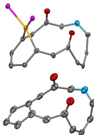
Figure 2. Comparison of the orifices in adduct (\text{Ph}_3\text{P})_2\text{Pt-MMK-9} (1) 19 at the top and MMK-9 at the bottom. Color code: carbon, grey; nitrogen, blue; oxygen, red; platinum, yellow; phosphorus, pink.
