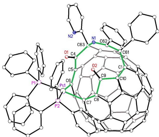
Figure 1. Crystallographic structure of one enantiomer of the adduct (\text{Ph}_3\text{P})_2\text{Pt-MMK-9} (1) obtained from a crystal of the solvate, (\text{Ph}_3\text{P})_2\text{Pt-MMK-9}\cdot n\text{-hexane}\cdot\text{methylcyclopentane} with the atoms shown as circles in order to simplify the drawing. The rim of the opening in the cage is shown with green bonds.
