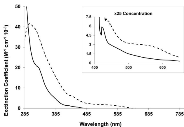
Figure 4. UV/vis spectra of MMK-9 (solid line) and (\text{Ph}_3\text{P})_2\text{Pt} -MMK-9 ( 1 ) (dotted line) taken in 0.025 mM solution.
