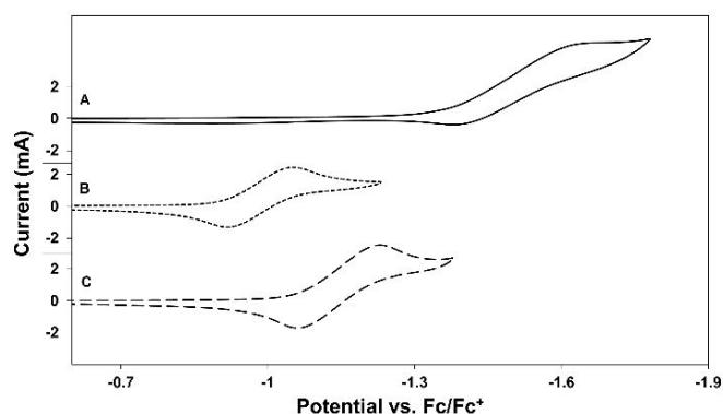
Figure 3. Cyclic voltammograms of A , (\text{Ph}_3\text{P})_2\text{Pt} -MMK-9 ( 1 ); B , MMK-9; C , C 60 using 1.0 mM solutions in o -dichlorobenzene solution with 50 mM tetra( n -butyl)ammonium hexafluorophosphate as supporting electrolyte at a scan rate of 0.01 V s -1 on a with a glassy carbon working electrode.
