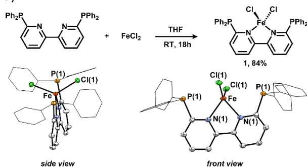
Figure 2. Synthesis and molecular structures (ORTEP, 50% probability level) of 1 . Hydrogen atoms have been omitted and phenyl groups on phosphorus depicted in wireframe for clarity. Note that this corresponds to one of two symmetry independent molecules from the unit cell. Selected bond distances ( \text{ \AA} ): \text{N}(1)\text{-Fe}(1) = 2.125(3) , \text{Cl}(1)\text{-Fe}(1) = 2.2504(8) . Selected bond angles ( ^\circ ): \text{Cl}(1)\text{-Fe}(1)\text{-Cl}(1) = 125.12(6) , \text{N}(1)\text{-Fe}(1)\text{-N}(1) = 77.34(16) .
