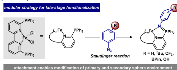
Figure 1. Conceptual design strategy for late-stage modification via the Staudinger reaction.
