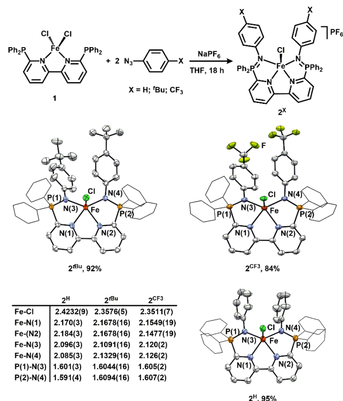
Figure 3. Synthesis of 2 X . (i) Treatment 1 with two equiv. aryl azide and one equiv. \text{NaPF}_6 , THF, RT, 18 h. Yields are based on 1 . Ellipsoids depicted at 50% probability. Hydrogen atoms have been omitted and phenyl groups on phosphorus depicted in wireframe for clarity.
