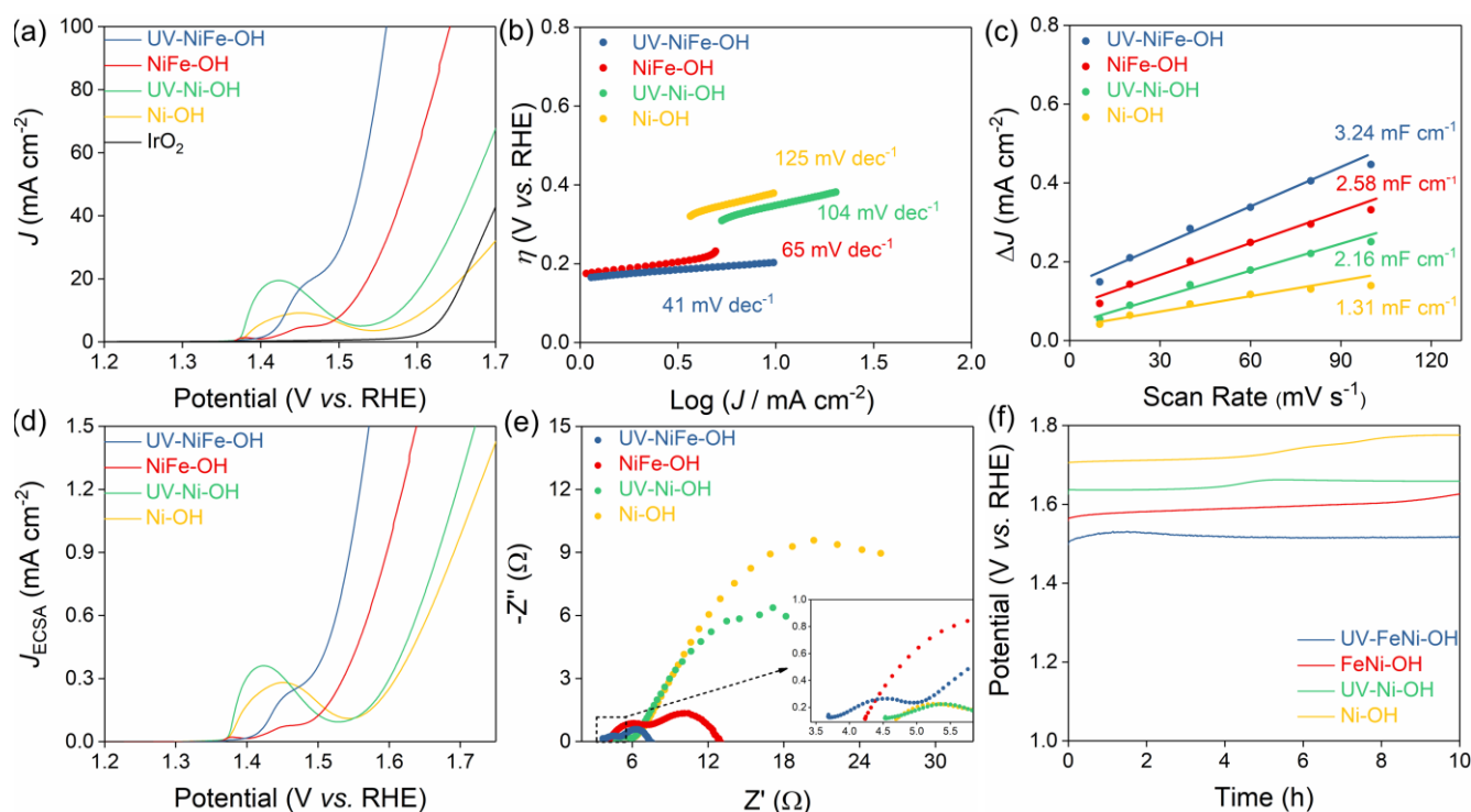
Fig. 5 (a) LSV curves of the catalysts for OER with 90% iR -compensation at a scan rate of 5 \text{ mV s}^{-1} . (b) Corresponding Tafel plots of the catalysts. (c) Double-layer capacitance ( C_{dl} ) as a function of scan rate from CV curves. (d) LSV curves normalized by ECSA from Fig. 5a. (e) EIS results tested with a frequency from 0.1 Hz to 10 kHz. (f) Chronopotentiometry durability measurement at a constant current density of 30 \text{ mA cm}^{-2} .
