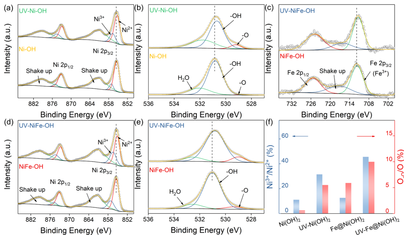
Fig. 3 High-resolution XPS spectra for the (a, d) Ni 2p, (b, e) O 1s and (c) Fe 2p regions of the catalysts. (f) Quantitative analysis of XPS results of the catalysts.
