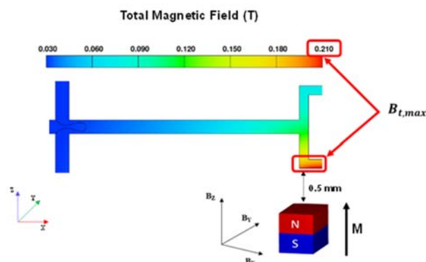
Fig. 2 Magnetic field distribution in the microfluidic device.
