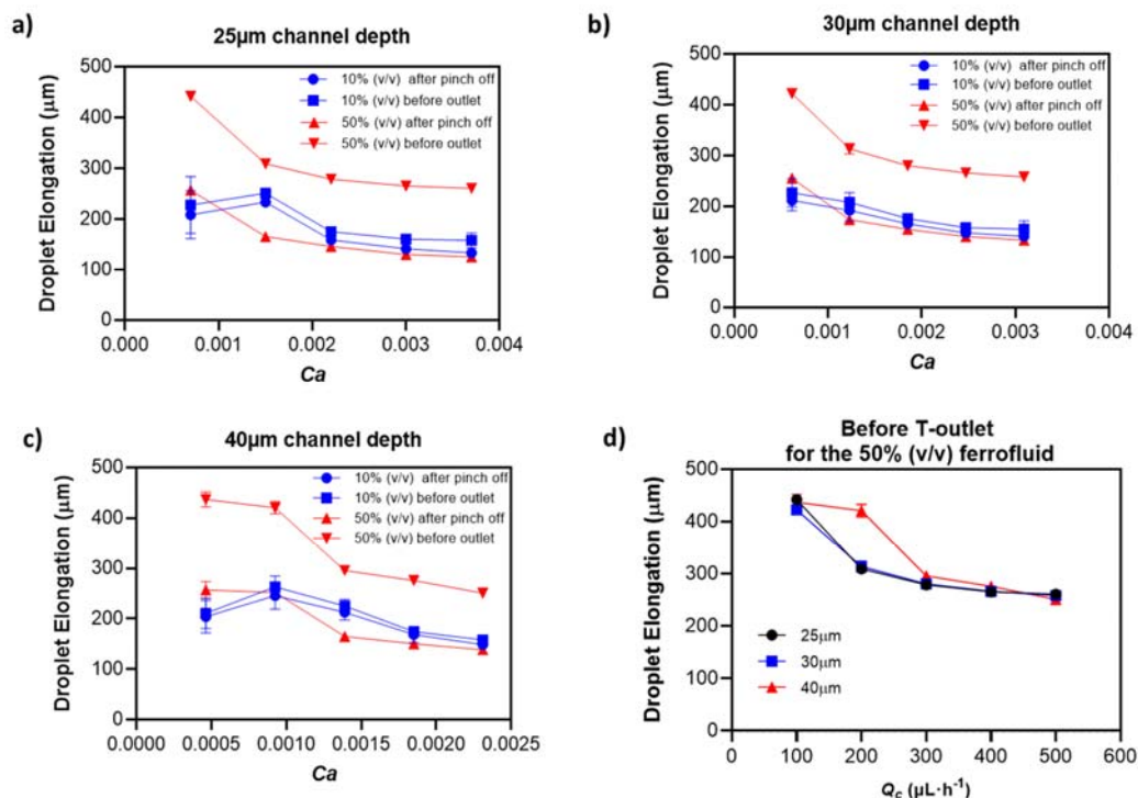
Fig. 11 Analysis of droplet elongation vs. Ca and Q_c . Droplet elongation vs. Ca for channel depths of a) 25 \mu\text{m} ; b) 30 \mu\text{m} ; and c) 40 \mu\text{m} depth under an applied magnetic field (elongation measured at the droplet formation region and at the end of the straight section of the microchannel; d) deformation of the droplet before reaching the outlet for the three channel depths vs. Q_c .
