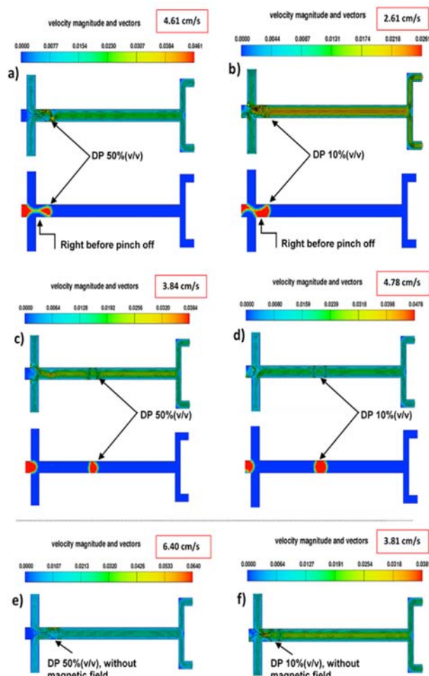
Fig. 4 Droplet generation visualization for the 25 \mu\text{m} deep channel at Q_c = 200 \mu\text{L}\cdot\text{h}^{-1} . a) and c) droplet generation for the 50% (v/v) ferrofluid under an applied magnetic field at different time points, before and after droplet pinch-off; b) and d) droplet generation for the 10% (v/v) ferrofluid under an applied magnetic field at different time points, before and after droplet pinch-off; e) droplet generation for the 50% (v/v) ferrofluid without magnetic field; and f) droplet generation for the 10% (v/v) ferrofluid without magnetic field.
