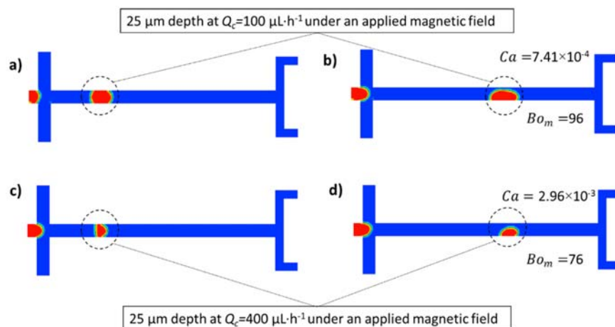
Fig. 10 Droplet shapes for 50% (v/v) of ferrofluid for 25 \mu\text{m} deep channels. a) and b) Q_c=100\text{ }\mu\text{L}\cdot\text{h}^{-1} under an applied magnetic field c) and d) Q_c=400\text{ }\mu\text{L}\cdot\text{h}^{-1} under an applied magnetic field.
