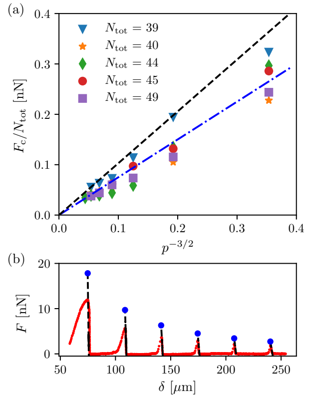
Fig. 4 (a) Evolution of the peak force, F_c normalized by N_{tot} , as a function of p^{-3/2} for five different compression experiments with different initial geometries. The size of the droplets is kept constant to R = 18.9 \pm 0.3 \mu\text{m} . The initial geometries are: ( \blacktriangledown ) 7 alternating rows of 6 and 5 droplets; ( \star ) p_{ini}=5; q_{ini}=8 ; ( \blacklozenge ) 8 alternating rows of 6 and 5 droplets; ( \bullet ) p_{ini}=5; q_{ini}=9 ; ( \blacksquare ) p_{ini}=7; q_{ini}=7 . The dash-dot line corresponds to the best fit of Eq. 2 to all the data with the energy per bond E_1 = 0.096 \text{ fJ} , while the dashed line ensures all measured maximal forces fall below the line with E_1 \approx 0.2 \text{ fJ} . (b) Measured force as a function of the distance between pipettes for a ( p_{ini}=7; q_{ini}=7 ) crystal. The blue data points correspond to the maximal forces, predicted from Eq. 2 with E_1 \approx 0.2 \text{ fJ} , which would be expected for an ideal experiment. The black dashed lines correspond to the theoretical predictions from Eq. 1 with k_1 \approx 1.46 \text{ mN/m} .
