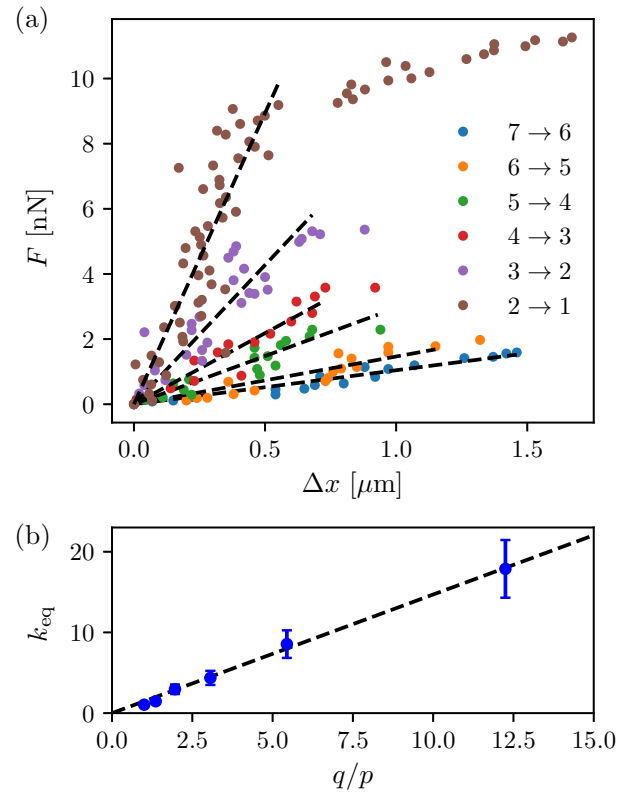
Fig. 3 (a) Force as a function of the compression \Delta x of the aggregate for the six different transitions. The part of the force shown is the rising one, that corresponds to the force between the black and blue dot in Fig. 2 (b), from onset to peak. The compression is defined to be equal to zero at the onset. The black dashed lines are linear best fits to the data. Each dashed line is only fitted to the elastic part of the compression. The slopes of these lines are the equivalent spring constants of the cluster, k_{\text{eq}} . (b) Evolution of k_{\text{eq}} with the aspect ratio q/p . The black dashed line is the best fit to Eq. 1. The error bars correspond to the uncertainty on the slopes of the linear fits in panel (a). Indeed, these linear fits are sensitive to the first and last data points included in the fit.
