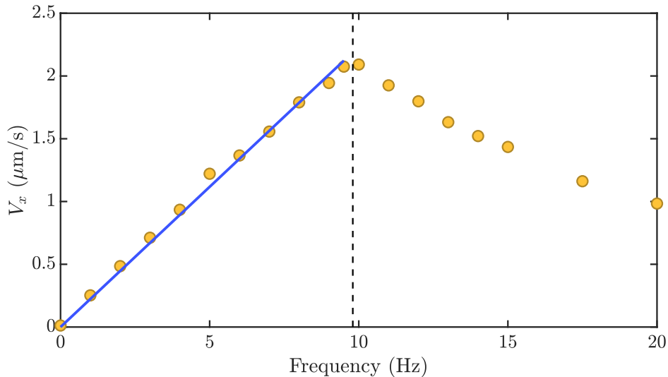
Figure 1: Measured velocity of dilute microrollers as a function of the frequency of the applied rotating magnetic field (40 G). Up to a frequency of \sim 9.8 Hz (vertical black dashed line), the velocity increases linearly with the frequency (blue line, slope = \bar{A}_f = 0.223 \mu\text{m} ). At higher frequencies the velocity decreases for increasing frequency, as the rollers cannot overcome the viscous torque of the surrounding liquid.
