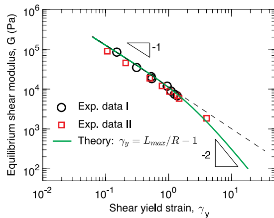
Figure 3. Dependence of stiffness on yield strain. The symbols are experimental data points extracted from Fig. 2a (circles) and Fig. 2b (squares). Solid line: Theoretical prediction for the dependence of network stiffness G on the shear yield strain \gamma_y calculated based on \gamma_y = L_{max}/R - 1 (eq. 1), where both L_{max} and R are determined by the G (eqs. 2, 3, 9, and 11).
