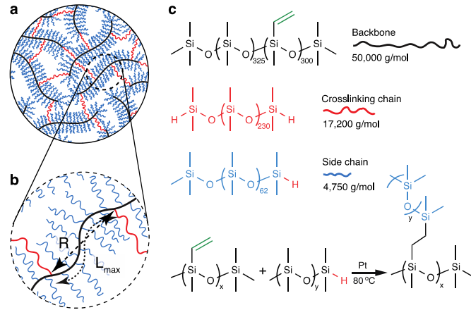
Figure 1. Molecular structure of soft bottlebrush elastomers. (a) A schematic view of a soft elastomer formed by crosslinking bottlebrush polymers: A multifunctional linear polymer chain acts as backbone (black); it is grafted by many side chains (blue), which are relatively short, mono-functional linear polymers carrying one reactive site, and crosslinking chains (red), which are di-functional linear polymers. (b) A schematic view of a section of the bottlebrush polymer between two neighboring chemical crosslinks. The section has an end-to-end distance of R and a contour length of L_{max} . (c) Three types of precursor reactive linear PDMS polymers form the structure illustrated by (a) through the hydrosilylation reaction between a hydride and a vinyl with the aid of platinum (Pt) catalyst at 80 °C.
