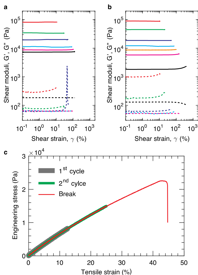
Figure 2. Mechanical properties of bottlebrush elastomers under large deformations.
