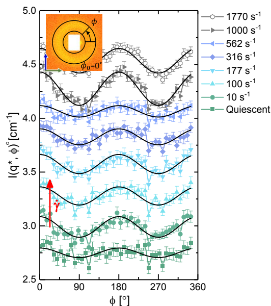
Figure 8. The azimuthal variation at q^* = 0.048 \text{ \AA}^{-1} for a representative set of shear rates. Cosinusoidal fits for each data set have been shown as black lines to highlight the extent of alignment. Error bars represent the
