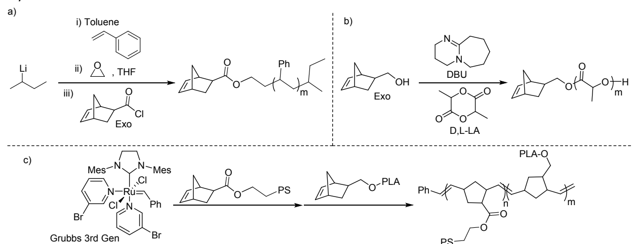
Figure 1: Synthesis of PS-b-PLA bottlebrushes. (a) Anionic polymerization of styrene to produce PS macromonomers. (b) DBU catalyzed ROP of lactide to produce PLA macromonomers. (c) Sequential addition ROMP of PS and PLA macromonomers.
