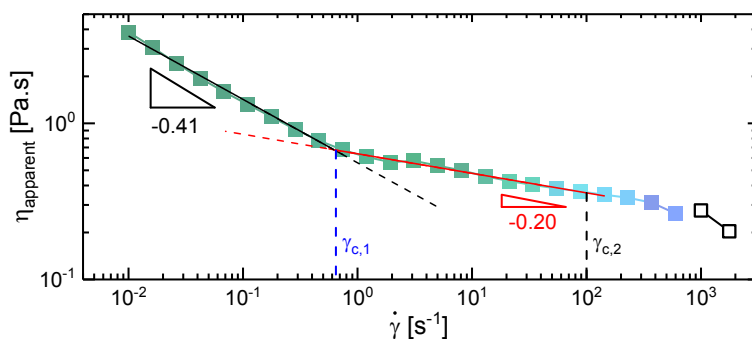
Figure 6. The steady flow response of the diblock bottlebrush solution. The color of each point represents the color captured by the microscope at the given shear rate, with open symbols corresponding to a lack of observable color.
