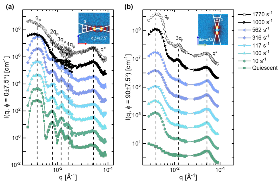
Figure 10. (a) Sector averages for select shear rates taken at 0^\circ in the 2-3 scattering plane. Dotted lines serve as guides to the eye, highlighting the initial peak positions under quiescence. (b) Sector averages for select shear rates taken at 90^\circ in the 1-3 scattering plane. Error bars represent the standard deviation of scattering intensities over the averaged area. Data have been offset to aid in the comparison of peak position and width.
