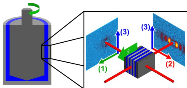
Figure 3. A schematic depicting the scattering planes that can be accessed in a concentric cylinder geometry. Scattering with the beam perpendicular to the geometry allows for the 1-3 scattering plane to be accessed,
