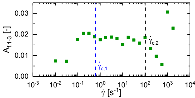
Figure 9. Alignment factor along the flow direction calculated from azimuthal sweeps performed at q = 0.048 \text{ \AA}^{-1} in the 1-3 scattering plane plotted against shear rate. Critical shear rates \dot{\gamma}_{c,1} and \dot{\gamma}_{c,2} have been highlighted with vertical dotted lines.
