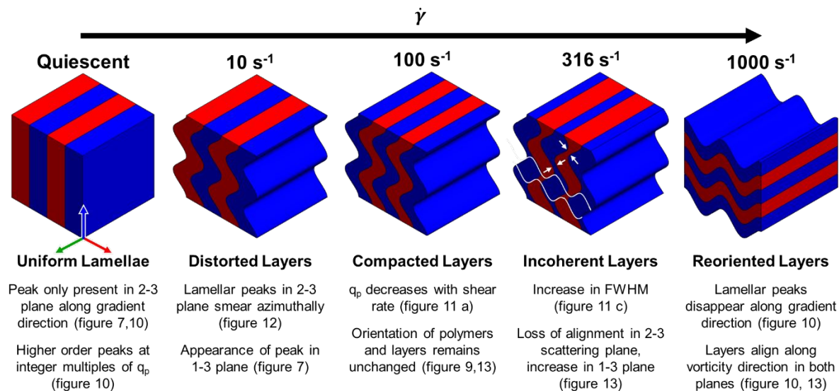
Figure 14. A schematic representation of the structural transitions undergone at different shear rates, supported by the data shown elsewhere in this paper. Arrows at \dot{\gamma} = 316 \text{ s}^{-1} serve as guides to the eye, highlighting pinch points that develop between the incoherent layers. White lines at the same shear rate indicate layers that could develop due to these pinch points.
