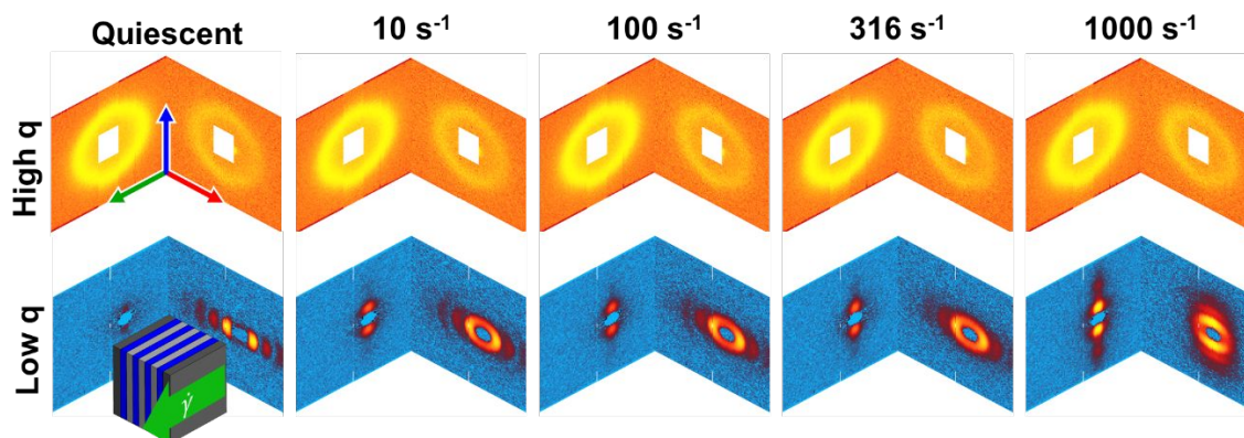
Figure 7. Representative scattering data mapped onto an isometric view. The green, red, and blue arrows represent the flow, velocity gradient, and vorticity directions, respectively.
