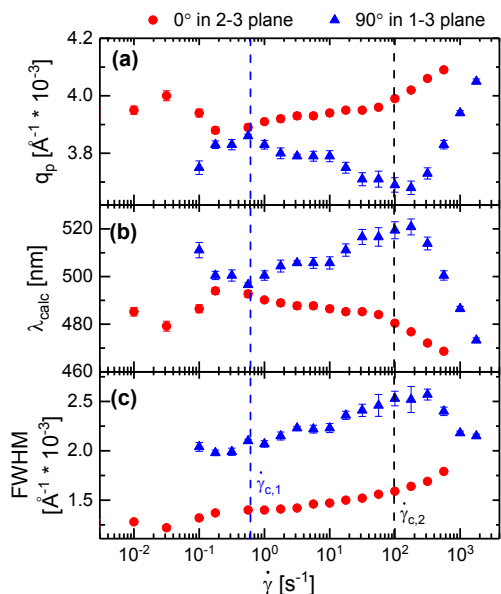
Figure 11. (a) The location of the primary peak, q_p , (b) expected reflected wavelength, \lambda_{calc} , as calculated by equation (2), and (c) the full width half max of the primary peak. Values calculated along the gradient direction in the 2-3 plane and vorticity direction in the 1-3 scattering plane. Error bars represent the standard error reported by OriginPro for the fitted gaussian peaks.
