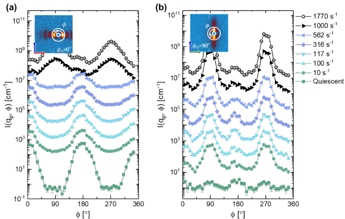
Figure 12. The azimuthal variation in the structure peak observed at q = 0.0039 \text{ \AA}^{-1} for a representative set of shear rates in the (a) 2-3 scattering plane and (b) 1-3 scattering plane. Data have been offset for the sake of comparing intensity variation with \phi .
