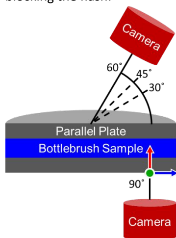
Figure 2. A schematic depicting the position of the microscope and camera setup relative to the sample during measurements. All images captured at 90^\circ correspond to the 1-3 shear plane. The light source originates from the camera at each angle. The green, red, and blue arrows correspond to the flow, gradient, and vorticity directions, respectively.
