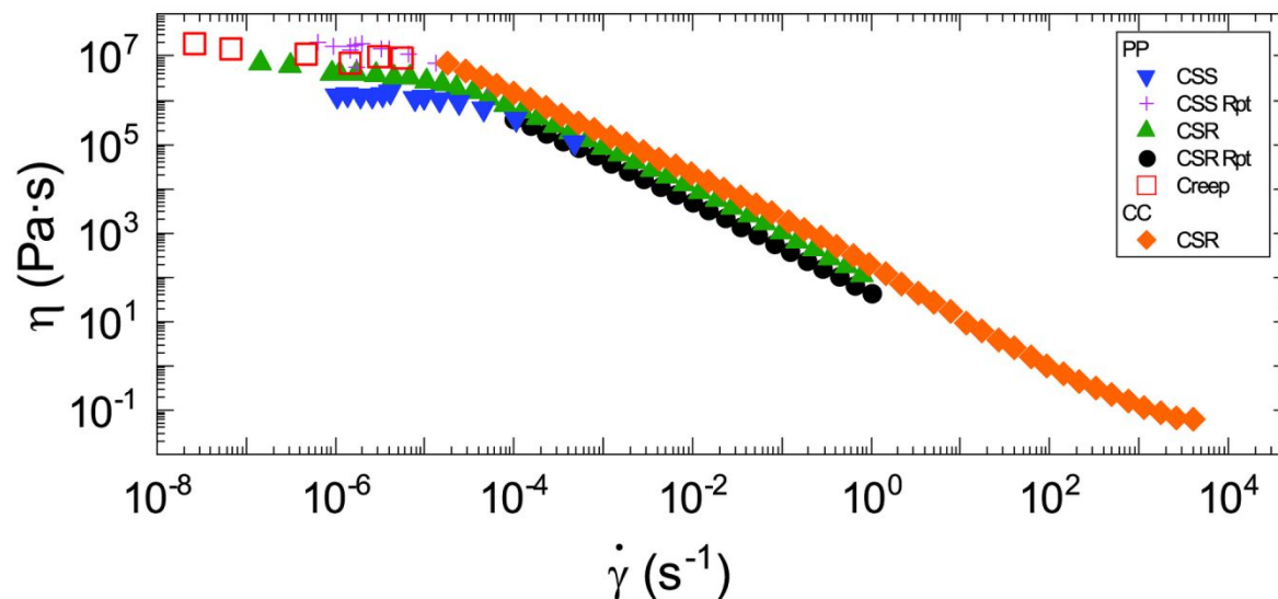
Figure 8: Viscosity versus strain rate plot corresponding to the flow curve in Fig. 2 . Blue inverted triangles and violet cross (repeat) are obtained from controlled shear stress (CSS) experiments on a parallel plate (PP) setup; green triangles (PP), black circles (repeat on PP) and orange diamonds (Couette) are obtained from controlled strain rate (CSR) experiments; open red squares are obtained from creep experiment on PP.
