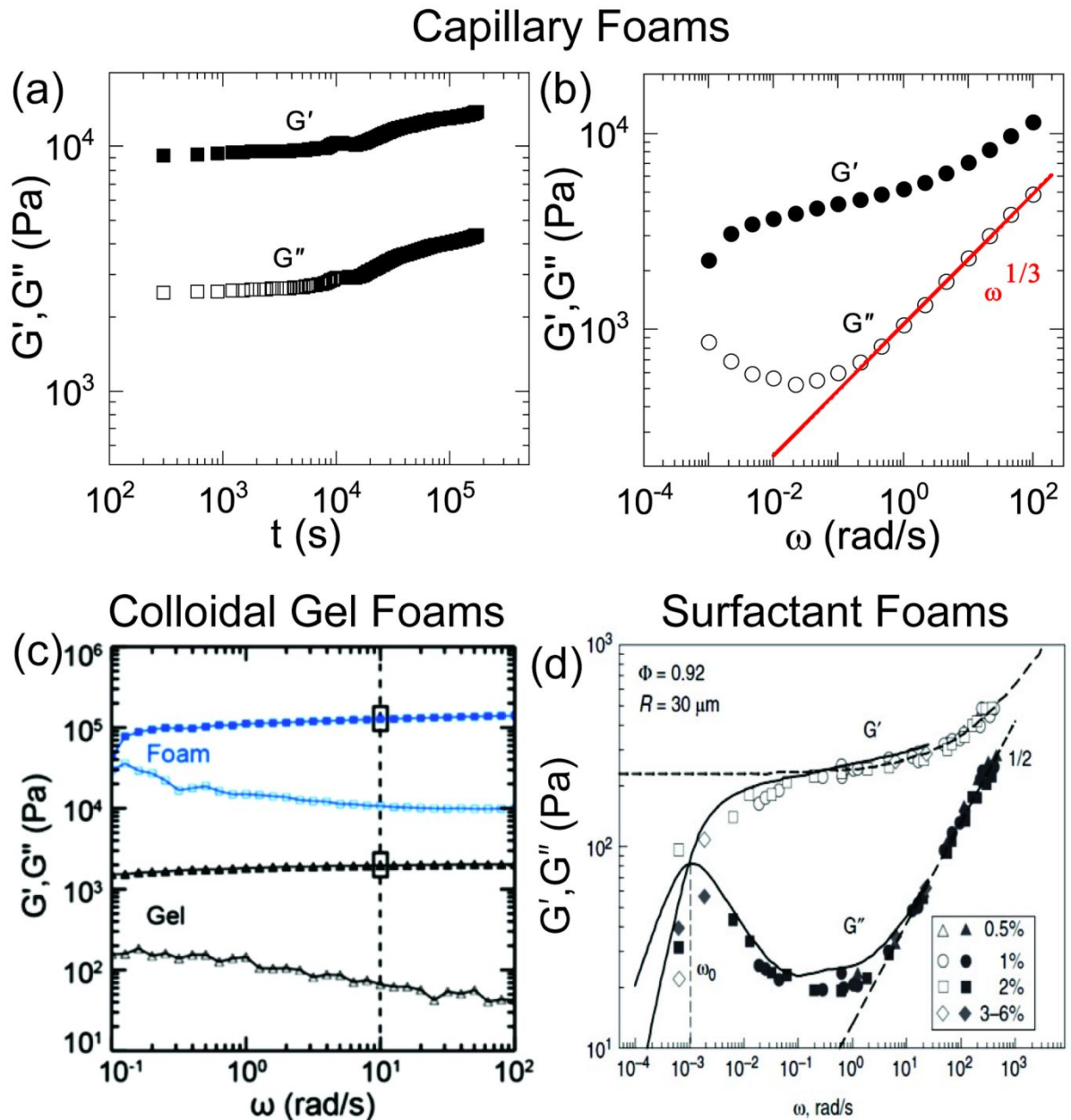
Figure 4: a) Plot of G' (filled squares) and G'' (open squares) for time sweep measurement at \omega = 10 rad/s on the CFs. b) Plot of G' (filled circles) and G'' (open circles) for frequency sweep at \gamma = 0.001 on CFs. c) Plot of G' (filled symbols) and G'' (open symbols) for frequency sweep on colloidal gels and gel foams (adapted with permission from Ref. 32. Copyright 2017 American Chemical Society). d) Plot of G' (open symbols), G'' (filled symbols) for frequency sweep on surfactant foams; symbols denote the imposed strain amplitude (adapted from Ref. 39. Reprinted with permission from Ref. 16).
