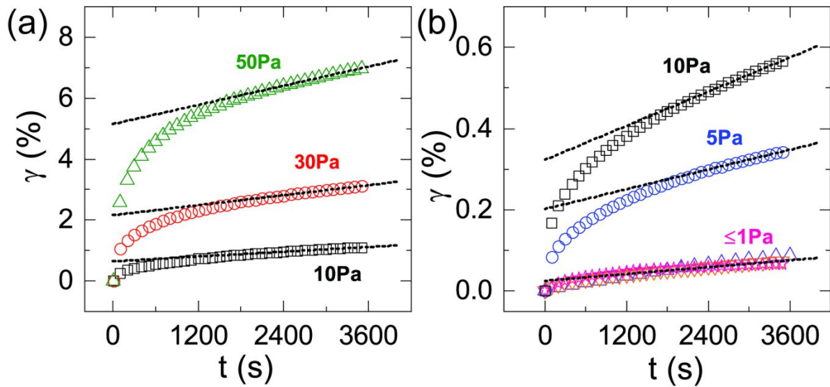
Figure 6: Plot of strain versus time in creep experiments; a) with applied stresses at 50 Pa (green triangles), 30 Pa (red circles), and 10 Pa (black squares). b) Plots of lower stresses at 10 Pa (black squares), 5 Pa (blue circles), 1 Pa (pink stars), 0.5 Pa (orange inverted triangles) and 0 Pa (violet triangles). Black dashed lines show linear fits used to obtain \dot{\gamma} .
