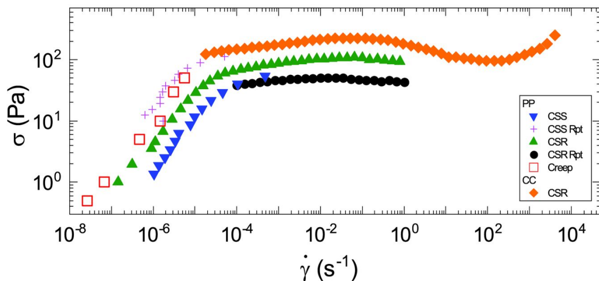
Figure 2: Plot of stress versus strain rate of the CF; blue inverted triangles and violet cross (repeat) are obtained from controlled shear stress (CSS) experiments on a parallel plate (PP) setup; green triangles (PP), black circles (repeat on PP) and orange diamonds (Couette) are
