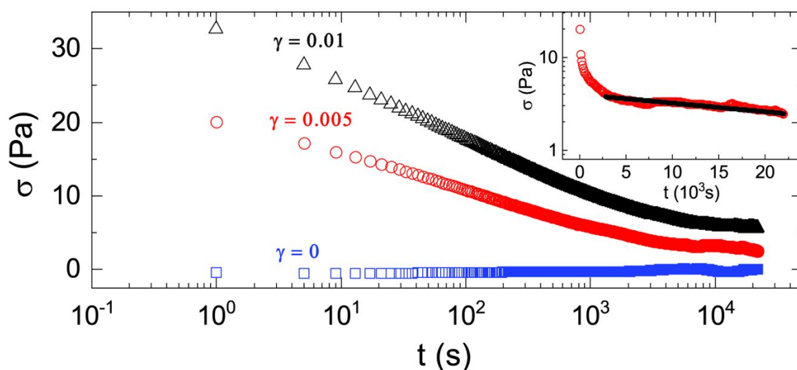
Figure 5: Plot of stress over time on CFs during stress relaxation experiments. Symbols correspond to applied strains below 10^{-6} (blue squares), applied strain in the linear regime at \gamma = 0.005 (red circles), applied strain outside the linear regime at \gamma = 0.01 (black triangles). The black line in the inset shows an exponential fit.
