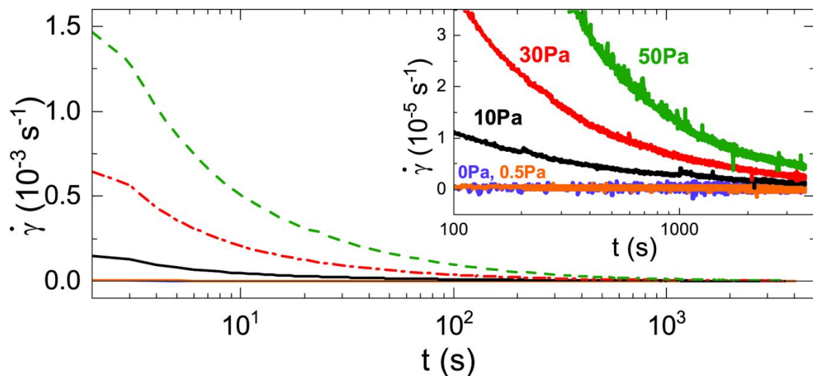
Figure 7: Evolution of strain rate in capillary foams during creep experiments; magnification of strain rate versus time at longer time period (inset). Applied stresses at 50 Pa (green
