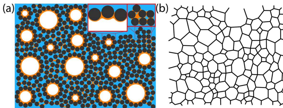
Figure 1: a) Schematic of capillary foam structure (bubble and particle sizes and volume fractions are not to scale). b) 2D representation of a high-quality surfactant foam (dry foam).
