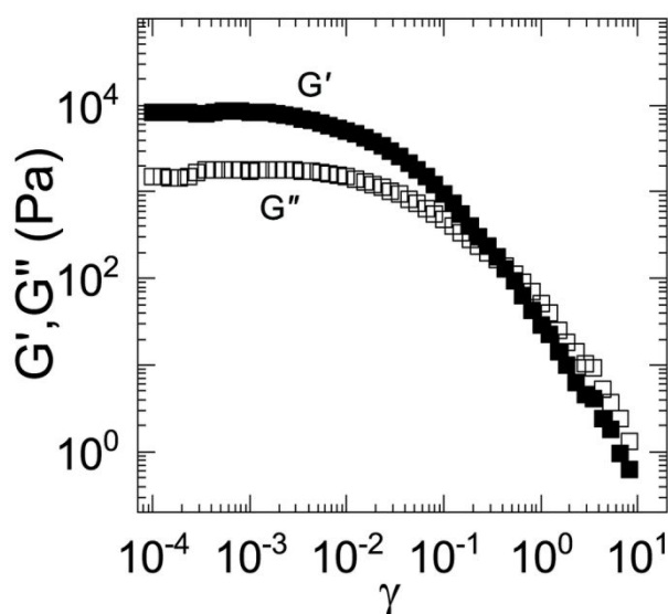
Figure 3: Plot of G' (filled square) and G'' (open square) versus the strain amplitudes tested at \omega = 1 rad/s.
