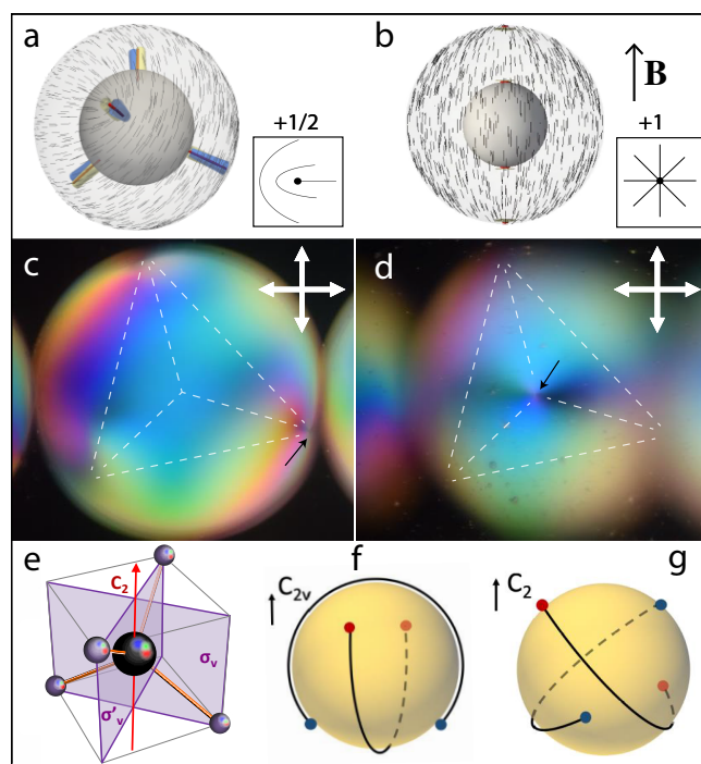
Fig. 2 Tetrahedral defect structure in homogeneous nematic shells. (a) Simulated shell with tetrahedral defect structure. The shell has four +1/2 disclination lines arranged in a tetrahedral fashion. The inset shows a schematic representation of the director field on the surface of the shell, around each +1/2 defect. This structure is expected to evolve towards a bipolar defect structure, with a pair of +1 boojums at each pole, as shown in (b), when applying a sufficiently strong magnetic field. (c), (d) Experimental shell with tetrahedral defect structure. The two images are cross-polarized micrographs showing different focal planes of the same shell: the black arrow indicates the defect that is in focus on each image. (e) Schematic showing the symmetries of a regular tetrahedron. There are three equivalent directions, connecting pairs of opposite cube faces, along which the tetrahedron has the symmetries of the C_{2v} point group: a two-fold rotational axis C_2 (in red) and two orthogonal mirror planes \sigma_v and \sigma'_v (in purple). In the schematic, we have represented these elements of symmetry for only one of the three equivalent directions. (f), (g) Schematics showing the symmetries of a tetrahedral nematic shell, where the lines represent the director field connecting +1/2 defects: the shell has the symmetries of the C_{2v} point group along the direction shown in (f), but only a C_2 rotational axis along the direction shown in (g).
