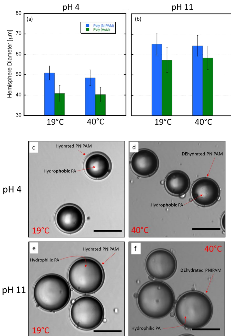
Figure 2. Janus microgel hemisphere diameter as a function of temperature and pH. (a) average change in PNIPAM and PA hemisphere diameters in response to temperature in pH 4 aqueous solution. (b) average change in PNIPAM and PA hemisphere diameters in response to temperature in pH 11 aqueous solution. (c) JMs in the amphiphilic state at pH 4/ 19^\circ\text{C} . (d) JMs in the hydrophobic state at pH 4/ 40^\circ\text{C} . (e) JMs in the hydrophilic state at pH 11/ 19^\circ\text{C} . (f) JMs in the amphiphilic state at pH 11/ 40^\circ\text{C} . Error bars represent standard deviation. Scale bars are 50 \mu\text{m} .
