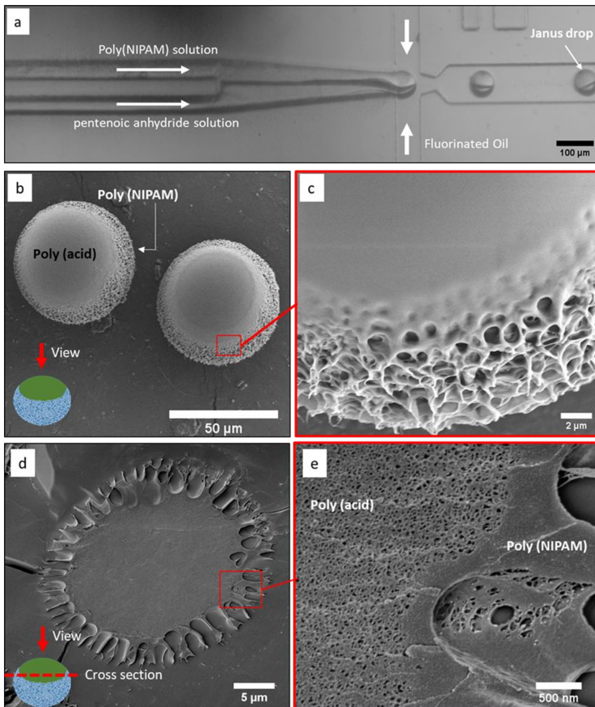
Figure 1. Janus microgel particles with poly (NIPAM) side and poly (acid) side via Janus droplet templating. (a) Janus droplet formation of polymer precursor solutions via shear by fluorinated oil in microfluidic flow-focusing device. (b) SEM image of the JM showing smooth PA surface and porous PNIPAM periphery. (c) magnified SEM image of the intersection of polymer networks showing the distinct transition from collapsed (smooth) PA to swollen (porous) PNIPAM network. (d) Cryo-SEM images of the internal fracture surface of the JM in water. (e) magnified cryo-SEM image of the relative pore sizes in each polymer network at their intersection in water.
