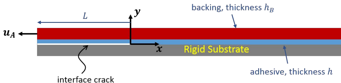
Figure 8: Schematic of the zero degree peel test. L is the length of the peel arm, L > h, h_B . The air gap between the peel arm and the substrate can be viewed as an interface crack.
