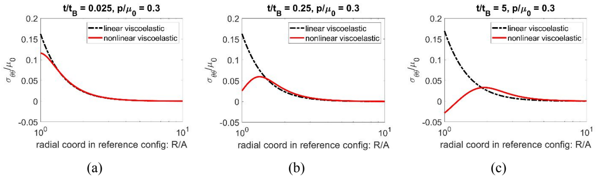
Figure 6. Distribution of normalized hoop stress \sigma_{\theta\theta}/\mu_0 at different normalized times t/t_B = 0.025, 0.25, 5 of a linear and nonlinear viscoelastic solid. Material parameters are given in eq.(14), and the constant internal pressure is p/\mu_0 = 0.3 for all t > 0 .
