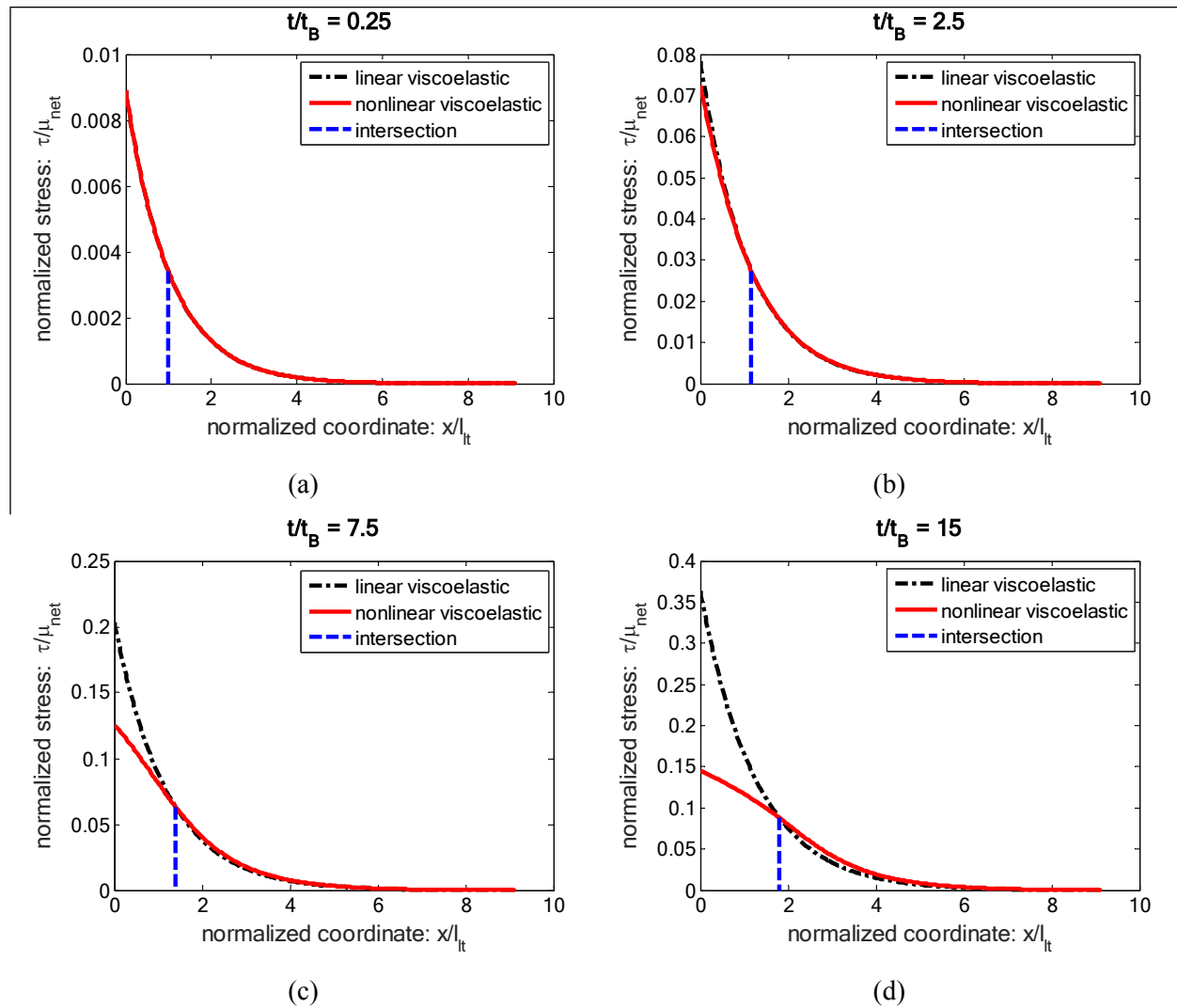
Figure 9. Shear stress profile in the zero-degree peel test at different times: t/t_B = 0.25, 2.5, 7.5, 15 . The applied displacement rate divided by the tape thickness is \dot{w}_A/h = 1/25t_B . The black dash-dotted curves are the stress profiles for the linear case, while the red solid curves are for the nonlinear case. The blue dashed line indicates the region where the stress of the nonlinear solid is lower than the linear one.
