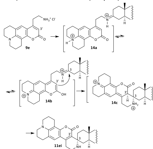
Scheme 3. Mechanism of Pictet-Spengler reactions of 4-(2-aminoethyl)coumarins 9 with ketones ( 10 ).
