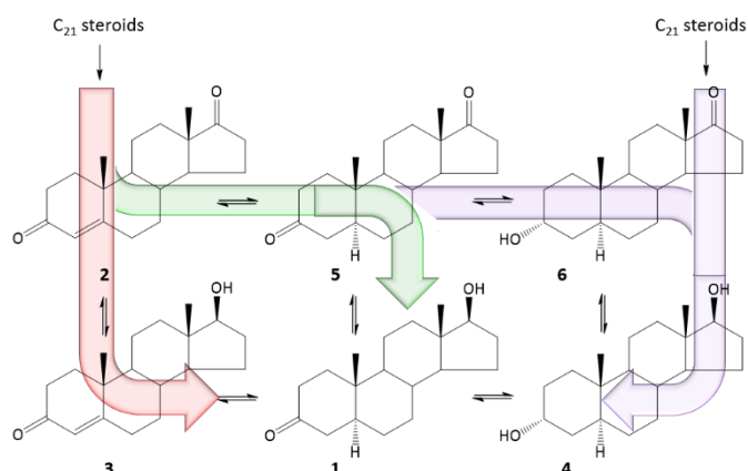
Fig. 1. Late-stage metabolic pathways converging on 5\alpha -dihydrotestosterone (DHT). Legend: frontdoor (orange), primary backdoor (green) and secondary backdoor (purple) pathways.
