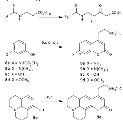
Scheme 1. Pechmann synthesis of substituted 4-(2-aminoethyl)coumarins 9 . Legend: a, CH 3 OC(=O)CH 2 CO 2 K; b, CH 3 SO 3 H; c, conc. HCl; d, TiCl(OiPr) 3 , 7.
