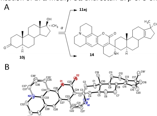
Fig. 3. Wagner-Meerwein Rearrangement. Panel A: Products of Pictet-Spengler condensation of coumarin 9e and 17 \alpha -methyl-5 \alpha -androstane-17 \beta -ol-3-one ( 10j ). Panel B: An ellipsoid plot (50% probability) for the single-crystal structure of rearrangement product ( 14 ). Hydrogen atoms were omitted to enhance clarity.
