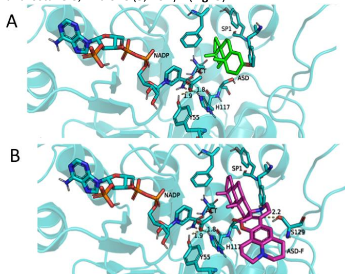
Fig. 5. Computational modeling. Panel A: 5 \alpha -Androstane-3,17-dione ( 5 ) in the SP1 binding site of AKR1C3 (PDB: 1XF0) containing proximal NADP +35 . Panel B: Pictet-Spengler adduct ( 11eh ) derived from 5 \alpha -androstane-3,17-dione ( 5 ) in the SP1 binding site of AKR1C3 (PDB: 1XF0) containing proximal NADP +35 .
