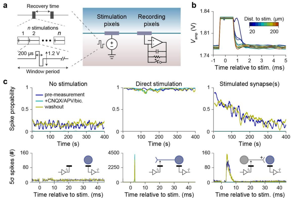
Fig. 4 | Stimulation of neurons and their synaptic connections. a , The pixel circuit configurations used for stimulation and recording of neurons. A biphasic voltage signal is repeatedly applied to stimulation pixels while the remaining pixels record. A switch in the feedback of the recording amplifier prevents saturation during stimulation and keeps V_e biased at a constant voltage before, during, and after the stimulation/shorting to help prevent long time constants associated with the electrode. b , Amplifier responses for the utilized shorting duration (feedback shorted during stimulation to +640 \mu s afterwards). The shorting prevents amplifier saturation and allows for signal recording <1 ms after stimulation. c , To reveal various types of connections during the repeated stimulations, EAP spike detection is performed on recording pixels. Three measurements are shown: an initial, with synaptic blockers, and after washout, each sequentially performed with 1 hour (3600 s) of recovery time, n = 8000 stimulations, and a window period of 50 ms, as defined in (a). The probability of an EAP spike over time (top) and a histogram of the spikes during the stimulation window (bottom, bin size 100 \mu s) are shown for each type of connection: a direct stimulation, stimulated synapse(s), and no stimulation.
