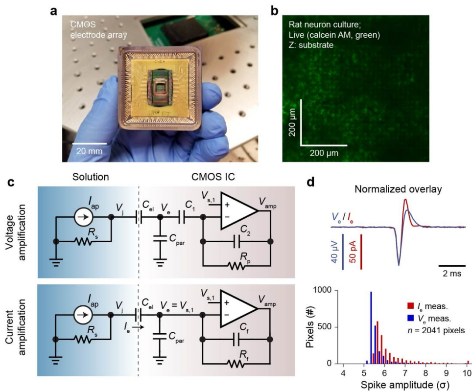
Fig. 1 | Extracellular recording of dissociated rat neurons using a CMOS electrode array. a , A CMOS electrode array packaged with a microfluidic well contains 64 \times 64 = 4,096 pixel pads ( 20 \mu\text{m} pitch) at its center connected to 4,096 amplifiers around its periphery. b , Representative confocal fluorescence microscopy image of a dense dissociated rat neuron culture on a CMOS electrode array used for the electrophysiological experiments. c , The neuron-electrode-circuit model using a voltage amplifier (top) and current amplifier (bottom). The op-amp with output, V_{\text{amp}} , amplifies extracellular neuron action potential currents, I_{\text{ap}} , which induce junction voltages, V_j , across the electrode seal resistance, R_s . The PtB electrode is modeled by its double layer capacitance, C_{\text{el}} , and parasitic line capacitance, C_p = 2 \text{ pF} . The voltage amplifier uses the ratio of capacitors to set a voltage gain of \sim 300 \text{ V/V} and a large feedback resistance of 50 \text{ G}\Omega to set a low-frequency pole of \sim 100 \text{ Hz} . The transimpedance current amplifier uses a feedback resistance of 700 \text{ M}\Omega to set its gain, and a feedback capacitance of 100 \text{ fF} to set a high-frequency pole of
