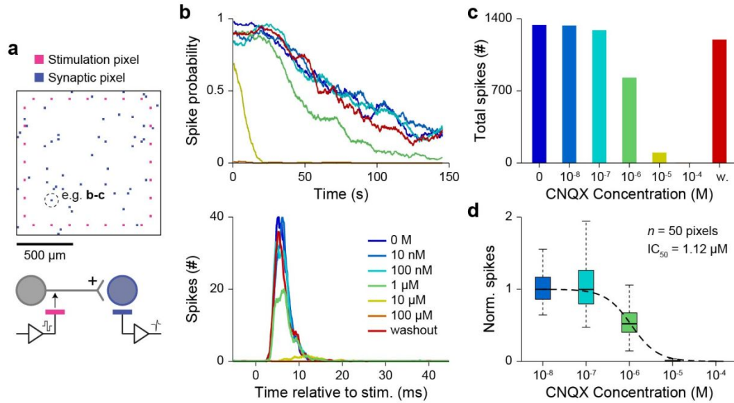
Fig. 5 | Synaptic blocker (CNQX) titration. a , Extracellular stimulation of selected pixels (magenta) excite synapses of measured extracellular neurons (blue). b , The probability over time (top), and spike histogram (bottom) are affected by the titration of CNQX, a synaptic blocker, across several orders of concentration and a subsequent washout. A window period of 50 ms and a recovery time of 600 s were used for the experiment. c , The total number of spikes reflects the drug's concentration for the example pixel in (b). d , Changes to the number of spikes across 50 synaptic pixels reveals the concentration dependence of CNQX with a calculated half maximal inhibitory concentration, IC_{50} \sim 1 \mu\text{M} .
