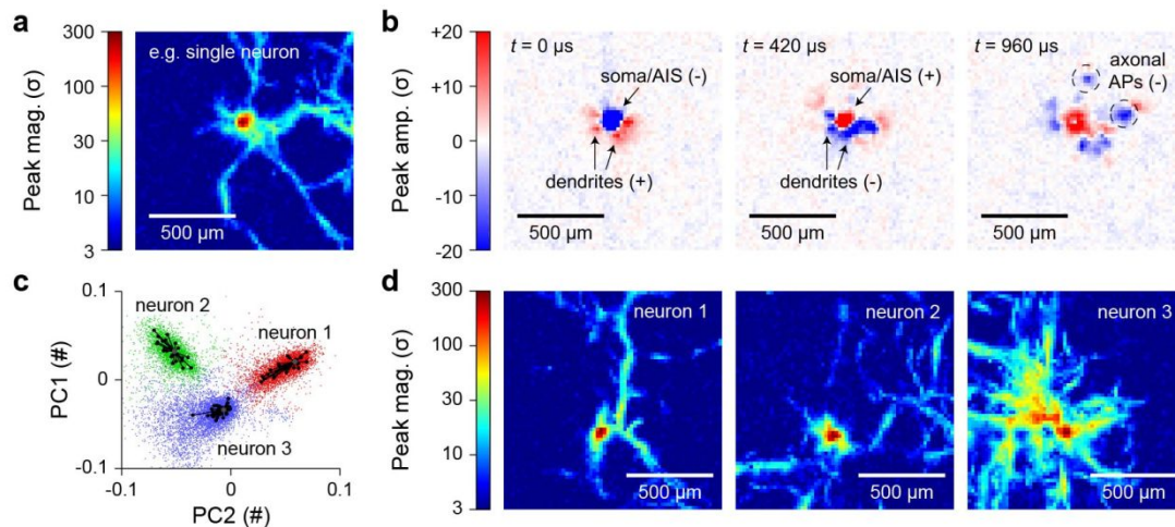
Fig. 2 | Mapping and spike sorting neurons and their action potential propagations. a , A rat neuron's electrical imprint on the pixel array is mapped from a 20-min recording and 1,800 extracellular spikes using spike-triggered-averaging (STA): the spike magnitude expressed in standard deviation ( \sigma ). b , The AP firing is visualized over time (see also Supplementary Video 1) and used to identify features of the neuron: the soma/axon initial segment (AIS) is negative and dendrites are positive at t = 0 and reverse polarities at \sim 400 \mu\text{s} , axonal AP propagations are observed to propagate away from the soma/AIS after the initial AP firing with a mainly negative polarity. c , Principle component (PC) analysis is used for spike sorting to distinguish unique neuron spikes, three neurons are determined for the pixel example. Clustering using sub-clusters (black) are combined following spike density gradients (maximum density, gray) in PC space (Supplementary Information, Methods). d , Electrical imprint for each of the three neurons show unique and distinct propagations for confirmation of the clustering.
