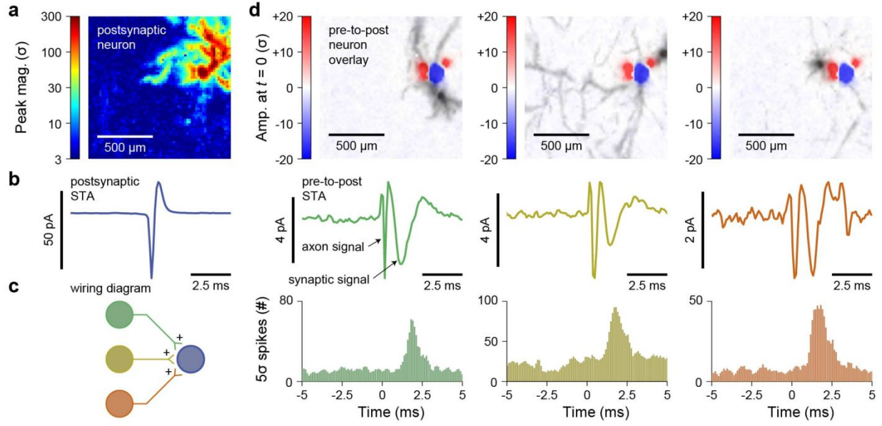
Fig. 3 | Mapping synaptic connections using spike-triggered-averaging and cross-correlation. a-c , A post synaptic neuron, with its spike-triggered-average (STA) electrical imprint and soma STA shown in (b), has multiple excitatory synaptic inputs (c). d , Pre-to-post overlays show that the soma/AIS or dendrites of the post-synaptic neuron overlay axon branches from the respective pre-synaptic neurons allowing for synapse formation. The three pre-to-post STA signals each show a synaptic signal following the axon propagation signal which are time correlated with the pre-to-post cross correlograms confirming the direct synaptic connections.
