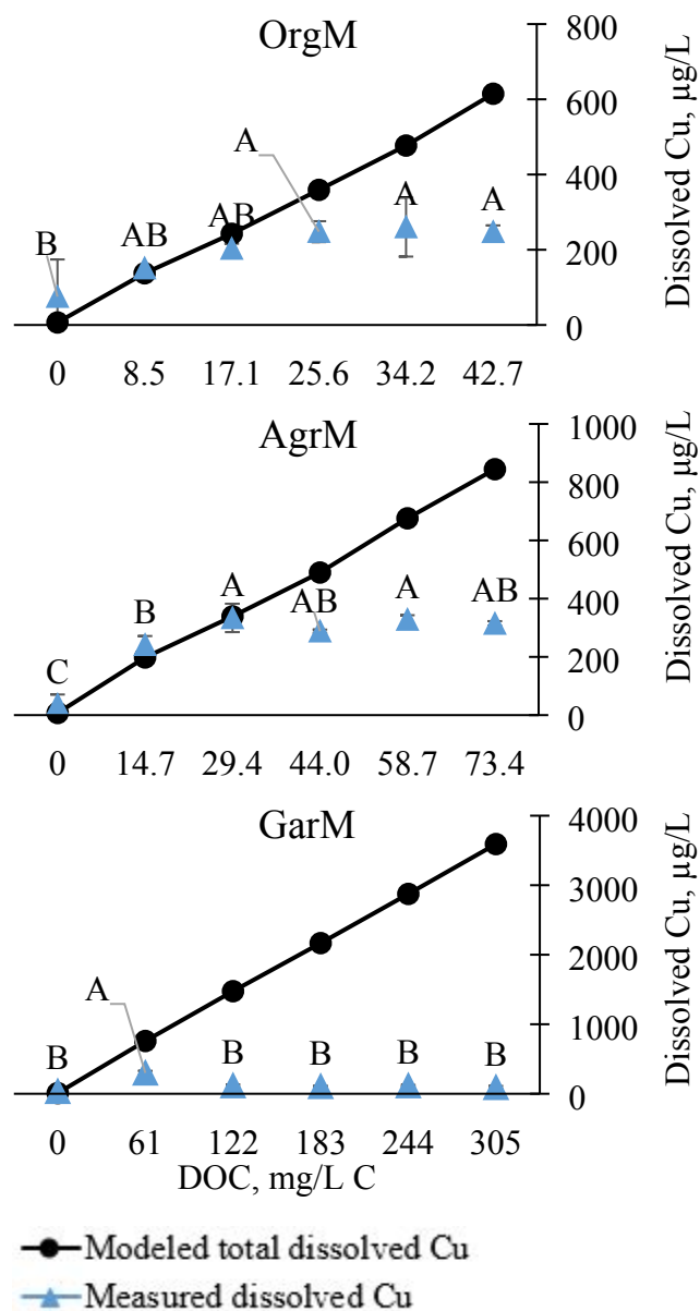
Fig. 5: Dissolved Cu concentrations from batch dissolution studies at 48 h measured after centrifugation (blue triangles) as a function of dilution of three SPEs at constant ionic strength. Measurements were compared to MINTEQA modeled Cu concentrations using default
