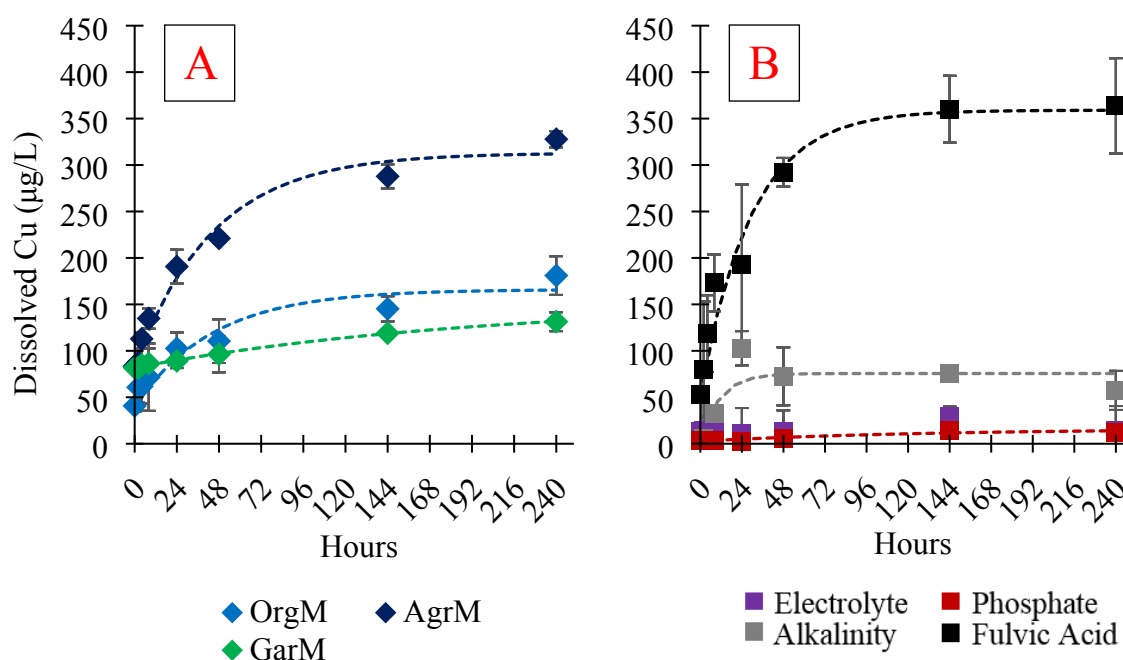
Fig. 4: Measured dissolved Cu and calculated first order kinetic models of dissolved Cu in all SPEs (A) and electrolyte, alkalinity (bicarbonate), phosphate, and fulvic acid treatments (B) as a function of time. Points are average of independent sample measurements ( n = 3 , except n = 6 in electrolyte and n = 2 in AgrM after 8 hours due to bacterial contamination of one sample). The dashed lines are the first order model results.
