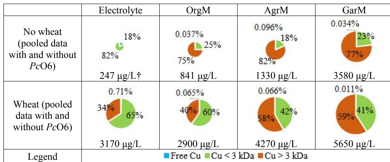
10 11 12 13 14 15 16 17 18 19 20 21 22 23 24 25 26 27 28 29 30 31 32 33 34 35 36 37 38 39 40 41 42 43 44 45 46 47 48 49 50 51 52 53 54 55 56 57 58 59 60 Fig. 2: Variations in the dissolved Cu size distribution in the sand PWs with treatments of electrolyte versus SPEs, with and without wheat growth, with CuO NPs. Data are pooled from systems with and without PcO6 inoculation. Pie areas and text below pie charts represent total dissolved Cu and are average of 12 independent sample measurements. Text overlays are shown as the amount of total dissolved Cu ( \mu\text{g/L} ), and % of the total per size category. Overlays that do not add to exactly 100% are due to rounding effects after two significant figures. The ‘no wheat’ treatments were statistically different from the ‘wheat’ treatments in each SPE. †Values for this treatment were from ultrafiltered samples, i.e. Cu < 3 kDa, as explained in Material and Methods section.
