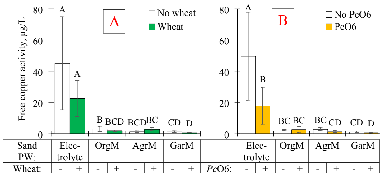
Fig. 3. The two-way interactions of wheat and SPE or electrolyte (A) and PcO6 and SPE or electrolyte (B) on free \text{Cu}^{2+} in the sand PW samples with \text{CuO} NPs. Amendment to the sand is 3.34 mM \text{Ca}(\text{NO}_3)_2 (electrolyte) or SPEs, OrgM, AgrM and GarM. The presence (+) and absence (-) of wheat or PcO6 is shown in the table below the charts. As a two-way interaction, PcO6 and non- PcO6 samples are pooled in graph A, and planted and unplanted samples are pooled in graph B; thus bars are average of 12 replicates. Error bars represent the 95% confidence interval and do not determine significance but are given to show the general spread of the data. Bars with differing letters are statistically different after Tukey HSD test. A logarithmic transformation was required to maintain normal distribution of the residuals.
