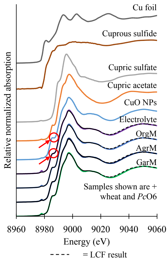
Fig. 7. Normalized X-ray absorption spectra of five standards (cupric sulfate, cupric acetate, CuO NPs, cuprous sulfide, and Cu foil) and CuO NPs from four sand PWs with wheat and PcO6 . The red circles highlight subtle difference in the shoulder between environmentally exposed and pristine CuO NPs. The linear combination fitting (LCF) results are shown with dashed lines overlaying the sample spectra. The peak appearing just before 8980 is a monochromator glitch and present in all measurements, but preserved in this figure to restrict manipulation of the data.
