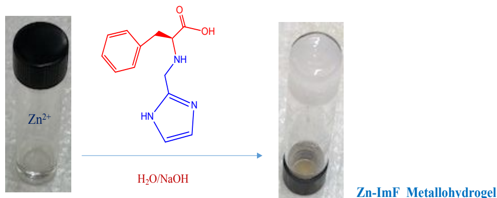
Fig. 2 Preparation of the Zn 2+ -triggered Zn-ImF metallohydrogel at the MGC of 0.07 M at room temperature.
