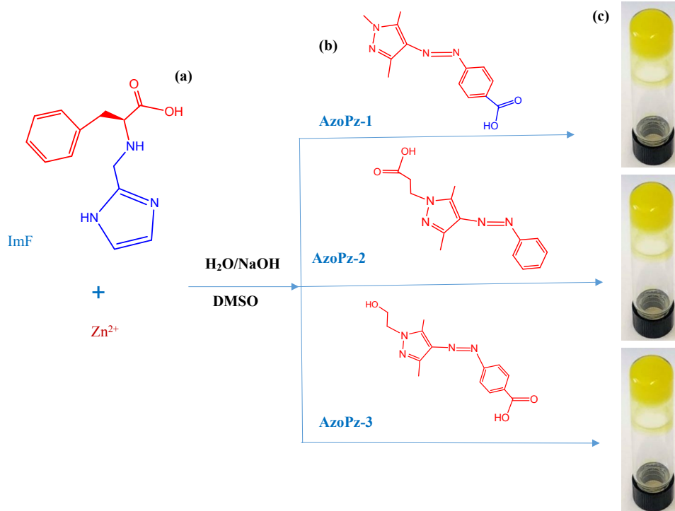
Fig. 1. a) Chemical structure of the ImF gelator; b) Molecular structures of the AzoPz-1, AzoPz-2 and AzoPz-3 photoswitches; c) Pictures of glass vials containing the metallogel coassembly formed by the Zn^{2+} ion triggered self-assembly of ImF (MGC of 0.05 M) and the three photoswitchable azo compounds at room temperature.
