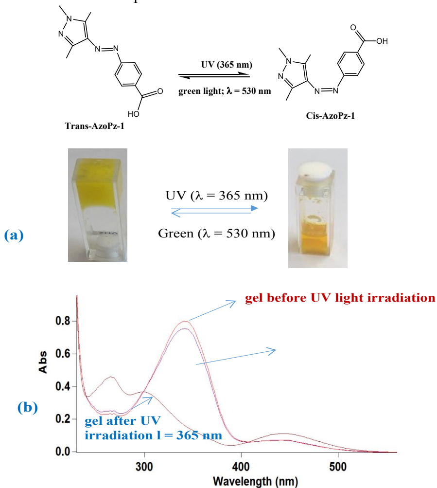
Fig. 7. (a) Photographic image of the reversible photo-induced gel-to-sol phase change of the gel formed by the Zn-Im-AzoPz-1 coassembly upon alternating UV and green light irradiation; (b) Changes in the UV-Vis spectrum of the Zn-Im-AzoPz-1 upon irradiation \lambda = 365 nm and recovery of the spectrum after with green light \lambda = 530 nm.
