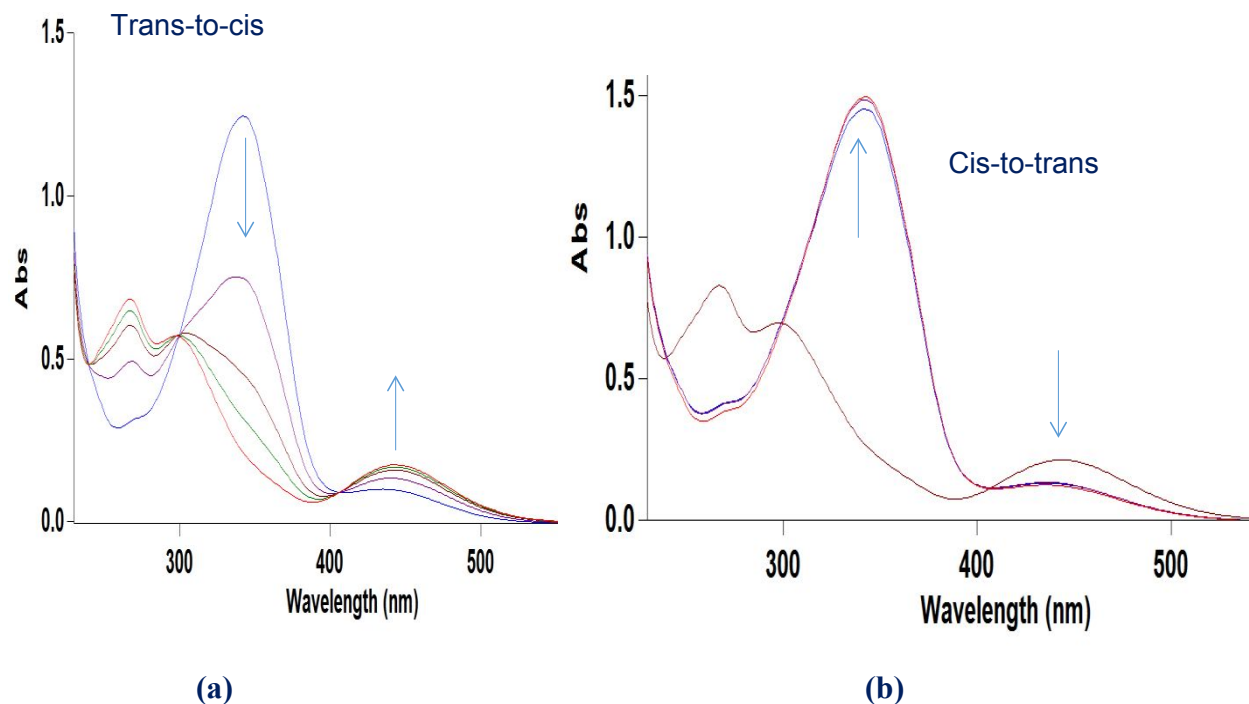
Fig. 6. UV-vis absorption spectra of AzoPz-1: a) trans-to-cis upon irradiation at \lambda = 365 nm 0-80 sec. b) cis-to-trans isomerization green light ( \lambda = 530 nm) 5-180 min.
