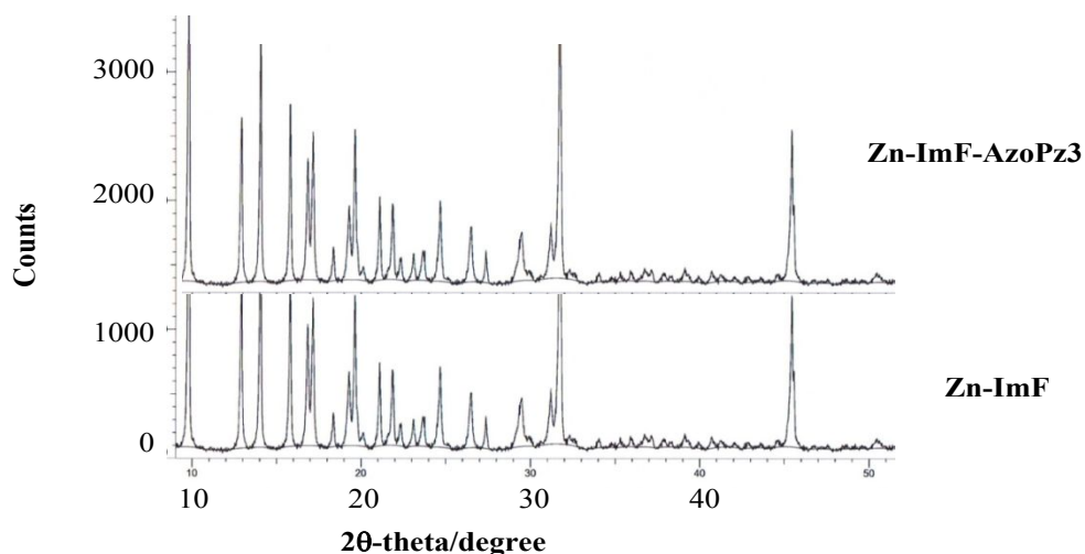
Fig. 8. XRD pattern of the Zn-ImF and Zn-ImF-AzoPz coassebly xerogels.
