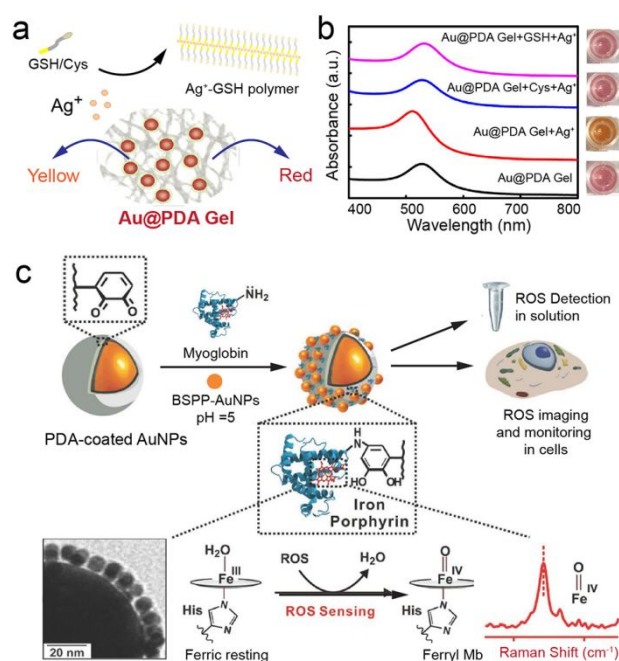
Fig. 20 In vitro biosensing of small targets via phenolic-based nanoparticles (a) Schematic illustration of the use of Au@PDA hydrogel for sensing biothiols. (b) UV-vis absorption spectra and photos of Au@PDA hydrogel with 200 μM Ag + in response to different biothiols (200 μM). (a and b) Reproduced with permission. Copyright 2018, American Chemical Society. (c) Schematic illustration for the synthesis of PDA-mediated SERS nanoprobes for detecting ROS (e.g., H 2 O 2 , O 2 - , and ·OH). The iron-porphyrin site of myoglobin in close proximity to Au core is used as a Raman reporter. Reproduced with permission. Copyright 2017, Wiley-VCH.
