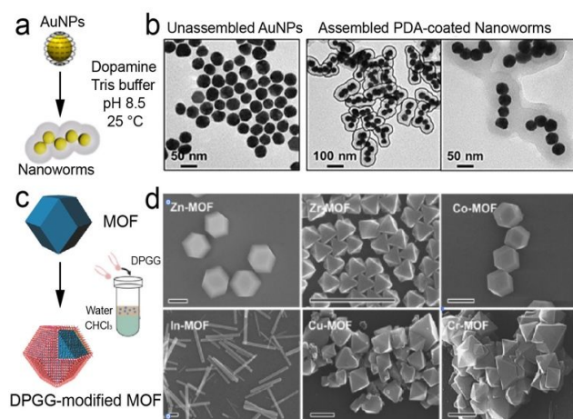
Fig. 13 In situ deposition of adhesive phenolic coating on pre-formed nanomaterials. (a) Schematic illustration of dopamine-mediated assembly of Au nanoparticles (AuNPs) into PDA-coated nanoworms. (b) TEM images of unassembled AuNPs and assembled nanoworms. (a and b) Reproduced with permission. Copyright 2019, American Chemical Society. (c) Schematic illustration of the surface functionalization of MOF particles by a phase transfer reaction. (d) SEM images of the DPGG-modified MOF particles of different metal ions. Scale bar: 1 \mu m. (c and d) Reproduced with permission. Copyright 2017, Wiley-VCH
