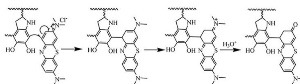
Fig. 7 The proposed adsorption mechanism between PDA and MB. Reproduced with permission. Copyright 2014, Royal Society of Chemistry.
