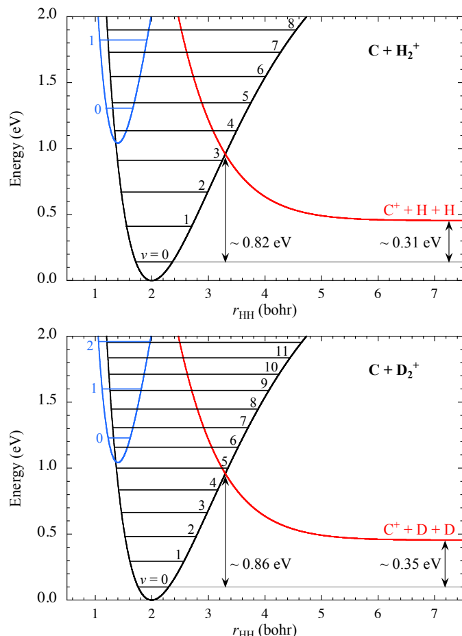
Fig. 6 Potential energy curves for the electronic states of C(^3P) + H_2^+(^2\Sigma_g^+) (black line), C(^4P) + H_2(^1\Sigma_g^+) (blue line), and C(^2P) + H_2(^3\Sigma_u^+) (red line) as a function of the diatomic bond length r_{HH} . The carbon atom/ion is located at an infinite distance from the diatom. Energies are given relative to the C(^3P) + H_2(^2\Sigma_g^+, r_e) dissociation limit. The upper panel shows the vibrational energy levels of H_2^+(^2\Sigma_g^+, v) and H_2(^1\Sigma_g^+, v') . The lower panel shows the vibrational energy levels of D_2^+(^2\Sigma_g^+, v) and D_2(^1\Sigma_g^+, v') .
