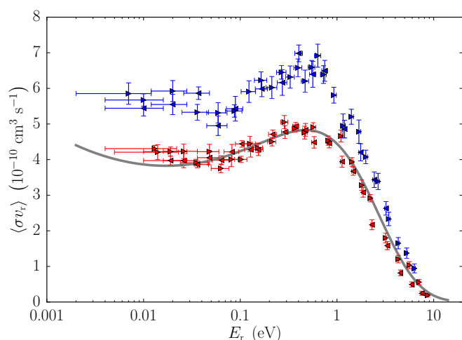
Fig. 3 Merged-beams rate coefficients \langle\sigma v_r\rangle as a function of the relative translational energy E_r . The present results for the C + H_2^+ \rightarrow CH^+ + H reaction (1) are shown in blue and those for the C + D_2^+ \rightarrow CD^+ + D reaction (2) are shown in red. The leftward pointing triangles correspond to v_n < v_i and the rightward pointing triangles to v_n > v_i . The vertical error bars represent the statistical uncertainty and the horizontal error bars show the energy spread at each E_r . The gray solid line corresponds to 0.796 times the experimental results of Schuette and Gentry 40 for reaction (2).
