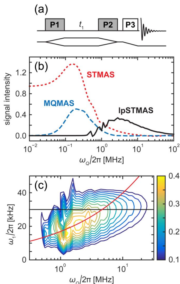
Fig. 1. Comparison of simulated S = 3/2 signal intensity for MQMAS, STMAS and lpSTMAS. (a) Three-pulse z-filter 15,16 sequence (P1 - t_1 - P2 - ZF - P3 - acq) used for SIMPSON 14 simulations. (b) Maximum signal for the MQMAS, STMAS and lpSTMAS experiments, as a function of \omega_Q , normalized to CT-selective one-pulse direct-excitation spectra. The P1 and P2 rf field was fixed to \omega_1/2\pi = 100 kHz for MQMAS and STMAS, and \omega_1/2\pi = 30 kHz for lpSTMAS. All pulses were applied on-resonance with the CT, except the P1 and P2 pulses for lpSTMAS which were applied at an offset \omega_{irr}/2\pi = +32 \cdot \nu_r = +512 kHz, where \nu_r = 16 kHz. (c) Contour plot of the lpSTMAS signal intensity as a function of \omega_1 and \omega_Q . The base contour level is set at an intensity of 0.1 and subsequent contours are at increments of 0.025. The horizontal black line denotes the position of the lpSTMAS curve shown in (b). The red curve highlights the optimal rf field dependence on the magnitude of the quadrupole coupling is approximately \omega_1 \propto \omega_Q^{0.37} .
