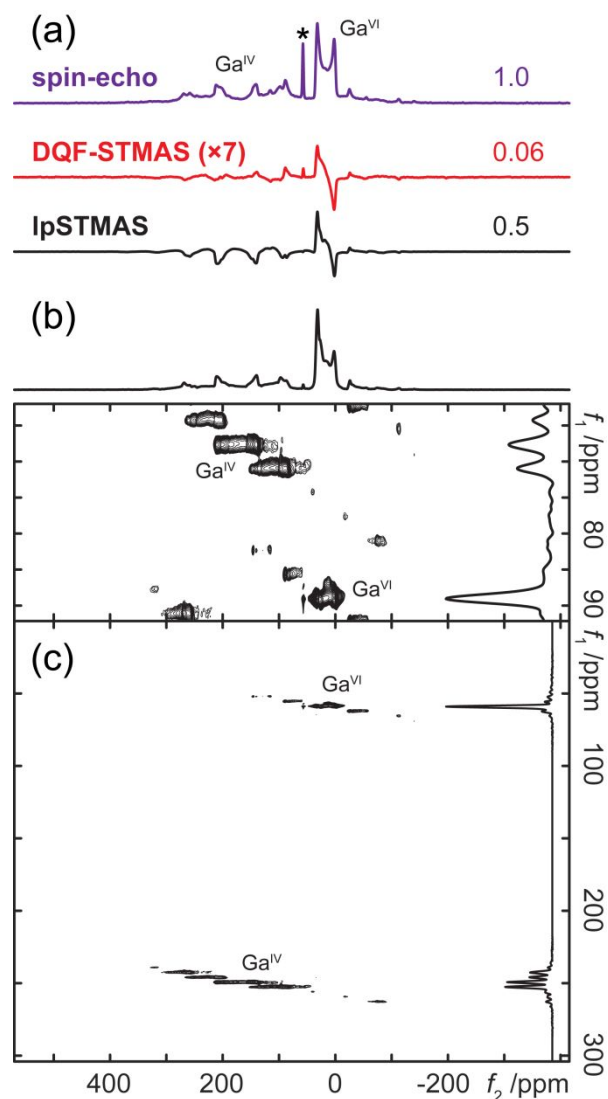
Fig. 2. (a) Experimental comparison of 71 Ga DQF-STMAS and IpSTMAS signal intensities with a spin-echo for \beta -Ga 2 O 3 . The vertical scale for the DQF-STMAS spectrum has been increased by a factor of seven to allow for easier visual comparison. The asterisk * denotes a sample impurity. 2D 71 Ga IpSTMAS spectrum after (b) isotropic shearing, and (c) Q -shearing, 22 expansion of the f 1 spectral width and shearing back into the isotropic representation to unravel spectral folding. The base contour level is set at 2% of the maximum intensity.
