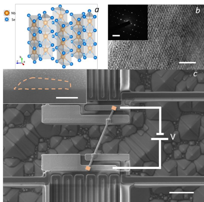
Figure 1. Crystal structure of \text{NbSe}_3 and suspended microdevice for thermal and electrical measurements. (a) A schematic diagram illustrating the crystalline structure of \text{NbSe}_3 . (b) HRTEM image of a \text{NbSe}_3 nanowire showing the well-aligned molecular chains. Inset: the selected area electron diffraction (SAD) pattern. The well defined pattern indicates the single crystalline structure. Scale bar: 5 nm (main panel); 5/nm (inset). (c) An SEM image of the measurement device with a \text{NbSe}_3 nanowire placed in between the two membranes. Inset: cross section of the measured nanowire. Scale bar: 5 \mu\text{m} (main panel); 100 nm (inset).
