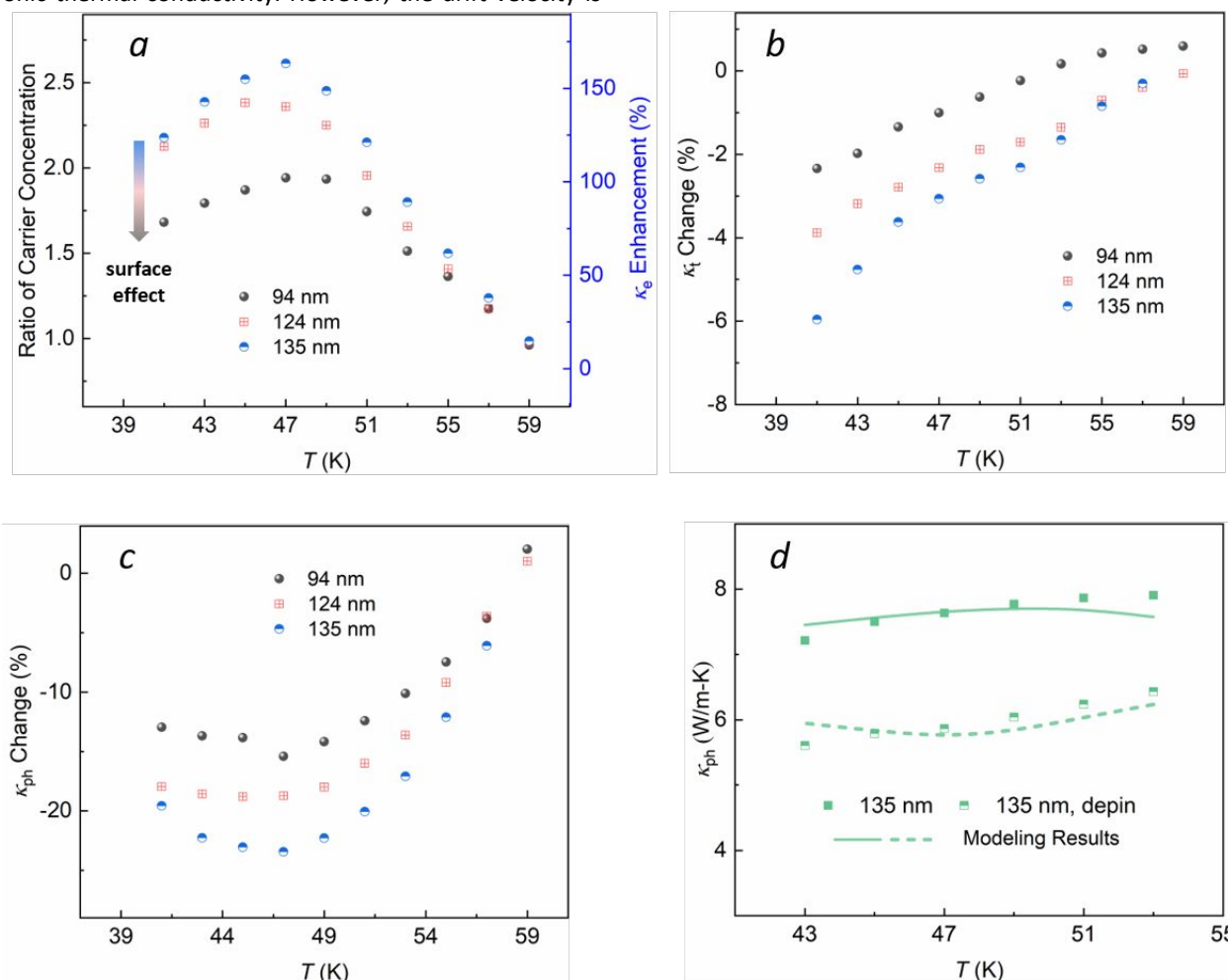
Figure 3. Thermal properties upon depinning. (a) Carrier concentration variation (Left axis) and corresponding electronic thermal conductivity enhancement (Right axis). (b) Measured total thermal conductivity reduction. (c) Lattice thermal conductivity change. (d) Experimental results and first principles calculations of \kappa_{\text{ph}} ( D_{\text{h}}=135 nm).
