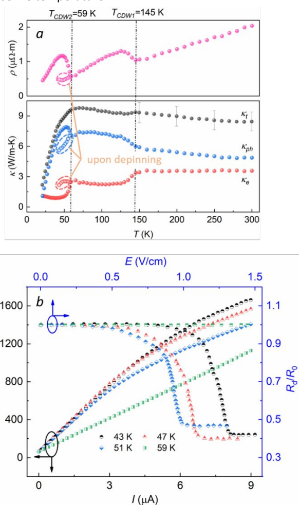
Figure 2. Depinning effect in NbSe 3 nanowires. (a) Measured pinning and depinning data for a sample with D_h=135 nm. The open dots show the data upon depinning. (b) Left-Bottom axis: I-V curves of a NbSe 3 nanowire ( D_h=135 nm) at different temperatures during the depinning test. Right-Up axis: resistance with respect to the applied electric field upon depinning normalized by the resistance when the electric field is zero for the same wire.
